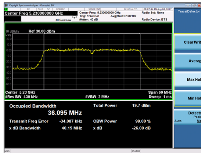
Plot 9-110. 26dB Emission Bandwidth and 99% OBW Chain B 802.11ac VHT 40 (CH. 46)
