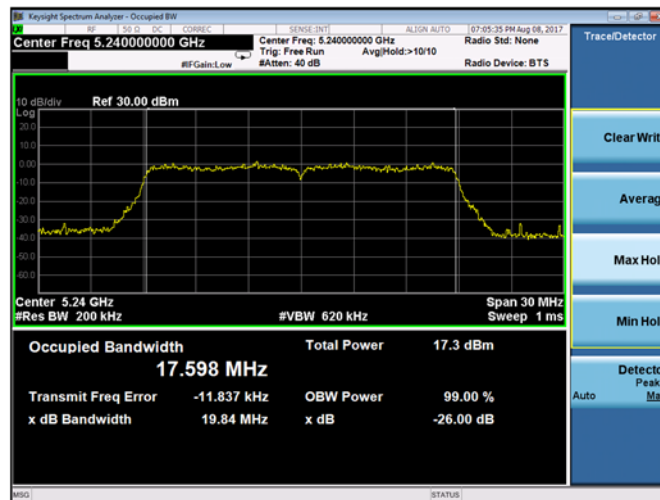
Plot 9-75. 26dB Emission Bandwidth and 99% OBW Chain A 802.11ac VHT 20 (CH. 48)
