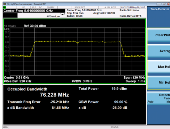
Plot 9-122. 26-dB Emission Bandwidth and 99% OBW Chain A 802.11ac VHT80 (Ch. 122)
