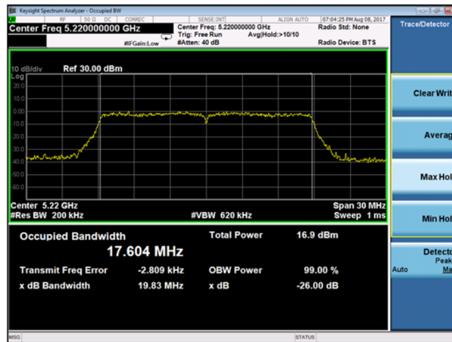
Plot 9-74. 26dB Emission Bandwidth and 99% OBW Chain A 802.11ac VHT 20 (CH. 44)
