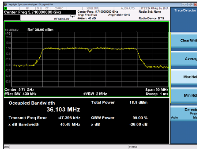
Plot 9-106. 26dB Emission Bandwidth and 99% OBW Chain A 802.11ac VHT 40 (CH. 142)
