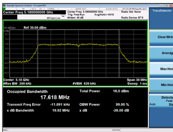
Plot 9-86. 26dB Emission Bandwidth and 99% OBW Chain B 802.11ac VHT 20 (CH. 36)
