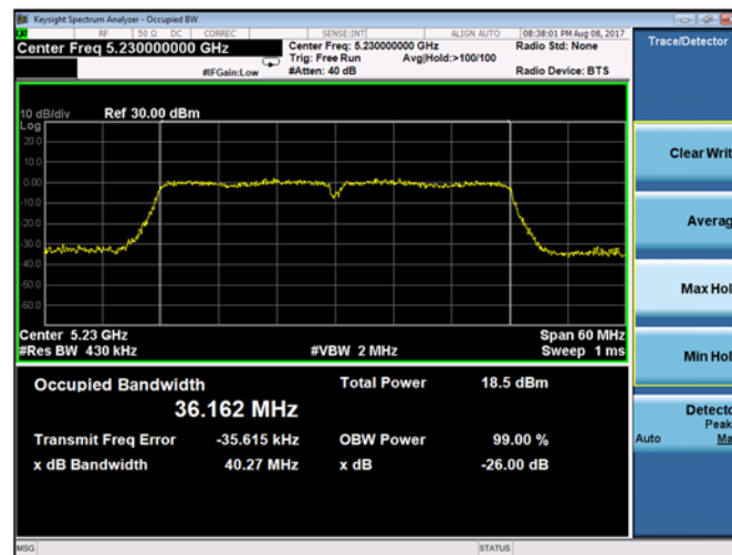
Plot 9-100. 26dB Emission Bandwidth and 99% OBW Chain A 802.11ac VHT 40 (CH. 46)
