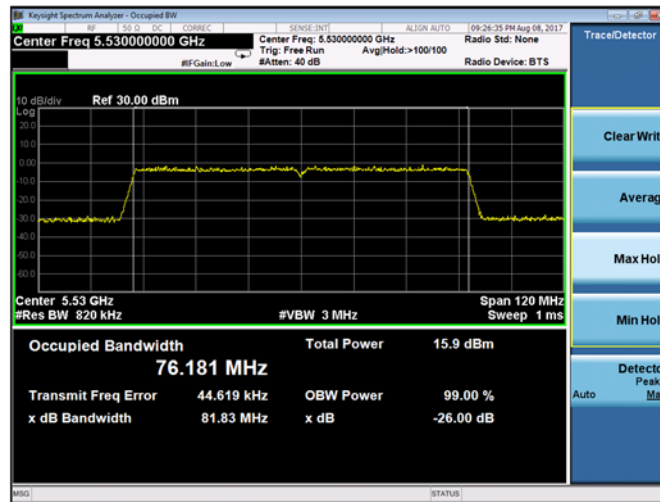
Plot 9-127. 26-dB Emission Bandwidth and 99% OBW Chain B 802.11ac VHT80 (Ch. 106)
