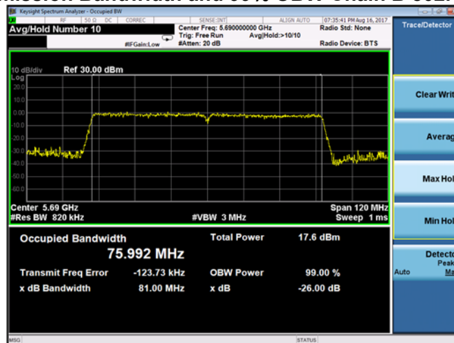
Plot 9-129. 26-dB Emission Bandwidth and 99% OBW Chain B 802.11ac VHT80 (Ch. 138)
