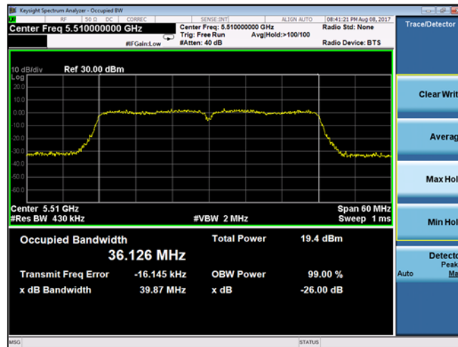
Plot 9-103. 26dB Emission Bandwidth and 99% OBW Chain A 802.11ac VHT 40 (CH. 102)
