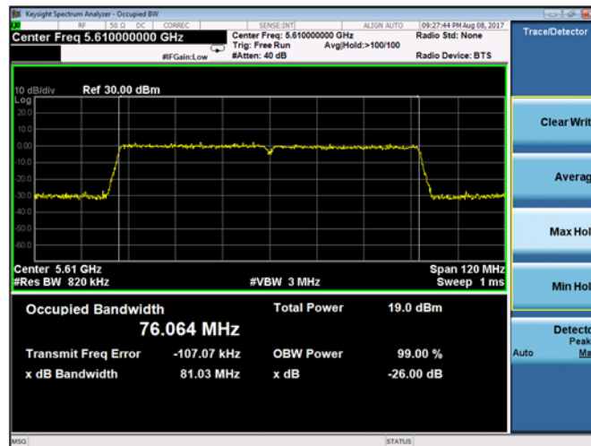
Plot 9-128. 26-dB Emission Bandwidth and 99% OBW Chain B 802.11ac VHT80 (Ch. 122)
