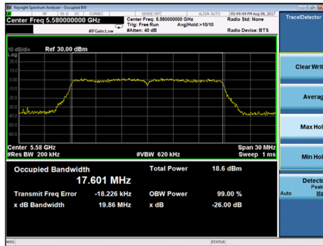
Plot 9-34. 26-dB Emission Bandwidth and 99% OBW Chain A 802.11n HT20 (Ch. 116)
