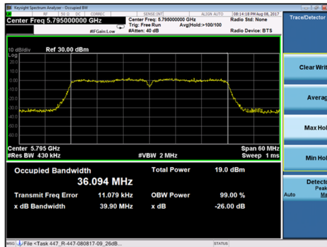
Plot 9-62. 26-dB Emission Bandwidth and 99% OBW Chain A 802.11n HT40 (Ch. 159)
