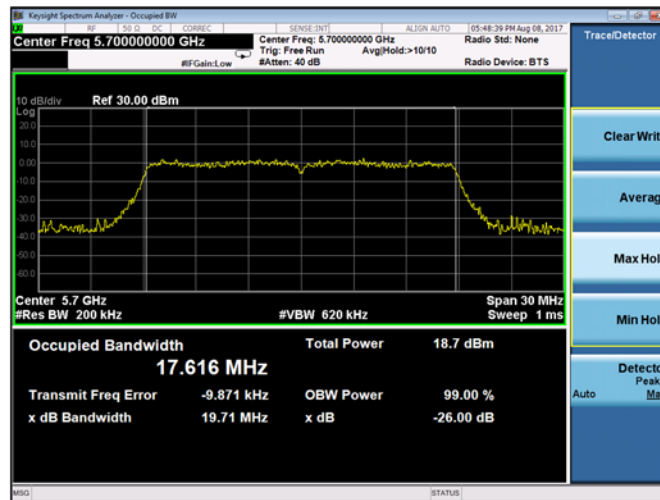
Plot 9-35. 26-dB Emission Bandwidth and 99% OBW Chain A 802.11n HT20 (Ch. 140)
