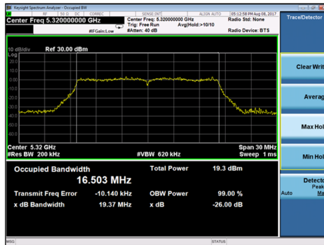
Plot 9-19. 26-dB Emission Bandwidth and 99% OBW Chain B 802.11a (Ch. 64)
