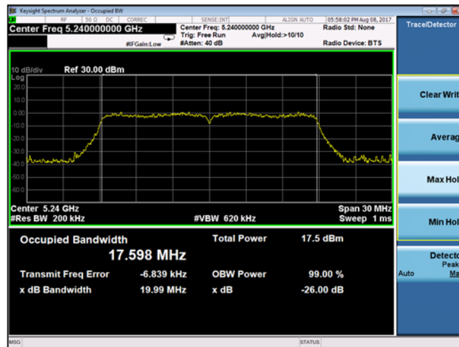
Plot 9-29. 26-dB Emission Bandwidth and 99% OBW Chain A 802.11n HT20 (Ch. 48)
