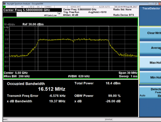
Plot 9-21. 26-dB Emission Bandwidth and 99% OBW Chain B 802.11a (Ch. 116)
