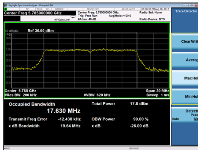
Plot 9-51. 26-dB Emission Bandwidth and 99% OBW Chain B 802.11n HT20 (Ch. 157)
