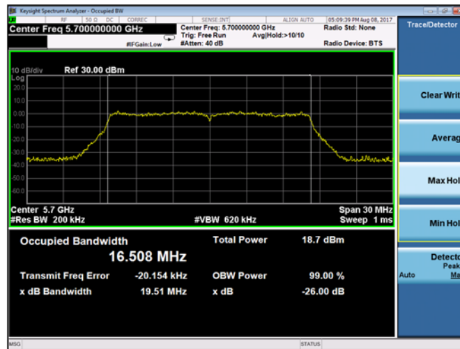
Plot 9-22. 26-dB Emission Bandwidth and 99% OBW Chain B 802.11a (Ch. 140)
