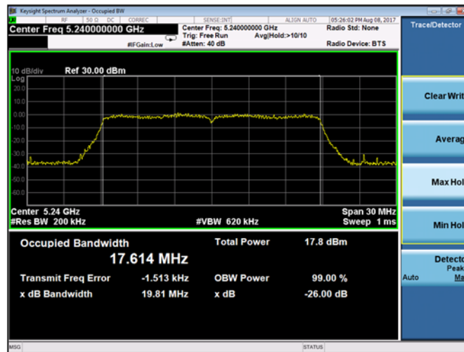
Plot 9-42. 26-dB Emission Bandwidth and 99% OBW Chain B 802.11n HT20 (Ch. 48)
