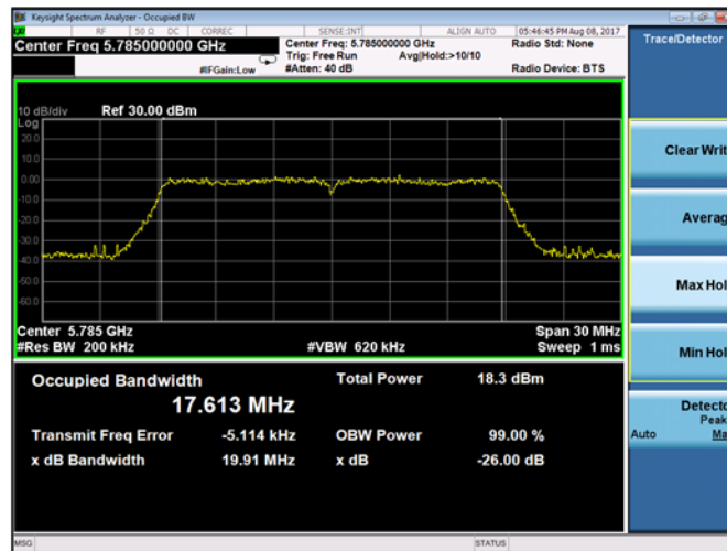
Plot 9-38. 26-dB Emission Bandwidth and 99% OBW Chain A 802.11n HT20 (Ch. 157)
