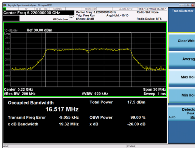
Plot 9-15. 26-dB Emission Bandwidth and 99% OBW Chain B 802.11a (Ch. 44)
