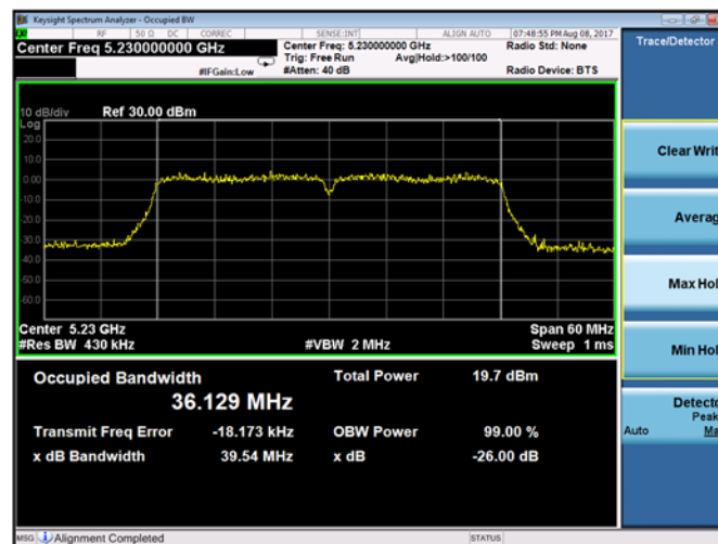
Plot 9-64. 26-dB Emission Bandwidth and 99% OBW Chain B 802.11n HT40 (Ch. 46)
