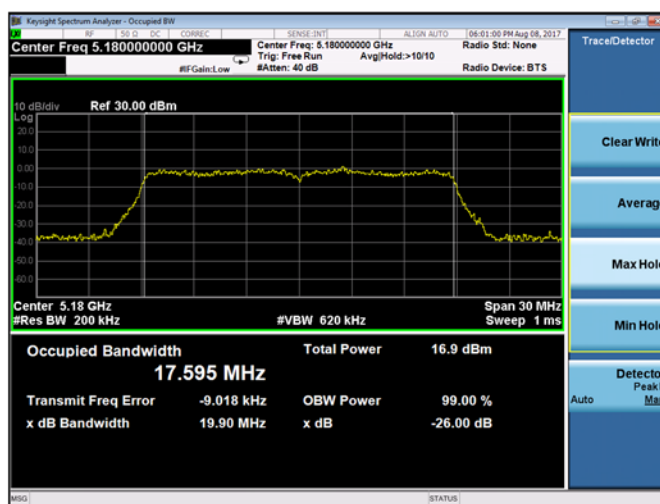
Plot 9-27. 26-dB Emission Bandwidth and 99% OBW Chain A 802.11n HT20 (Ch. 36)
