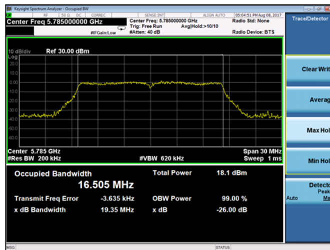
Plot 9-25. 26-dB Emission Bandwidth and 99% OBW Chain B 802.11a (Ch. 157)
