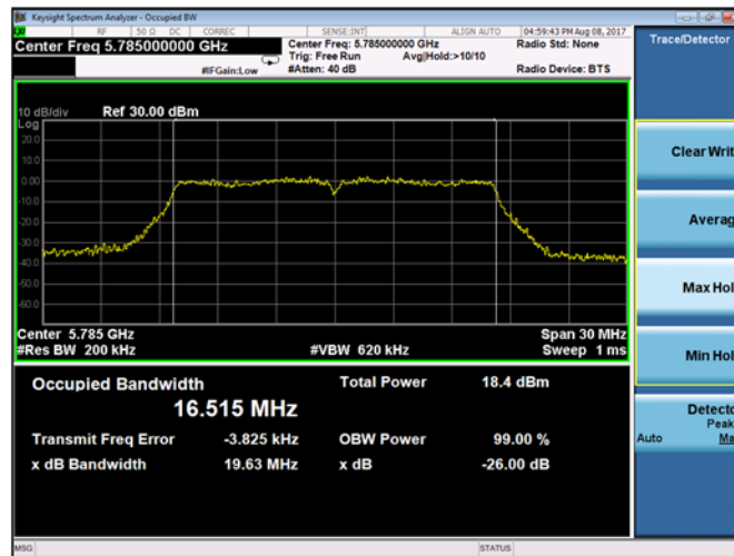
Plot 9-12. 26-dB Emission Bandwidth and 99% OBW Chain A 802.11a (Ch. 157)
