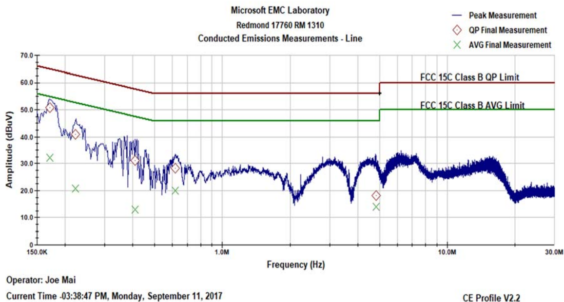
Plot 9-41. AC Line Conducted Emissions- Line (150 kHz- 30 MHz)
