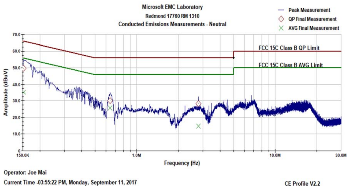
Plot 9-42. AC Line Conducted Emissions- Neutral (150 kHz- 30 MHz)
