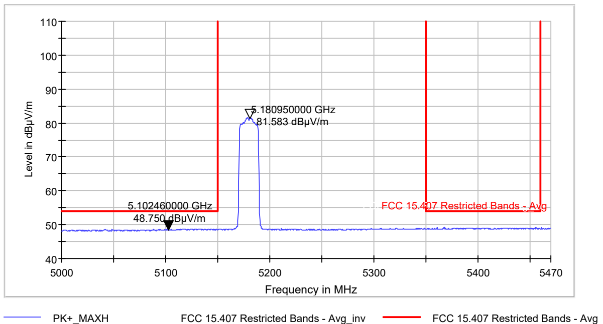
Plot 9-29. Average Radiated Band Edge Emissions Tx 802.11n (Ch. 36)
