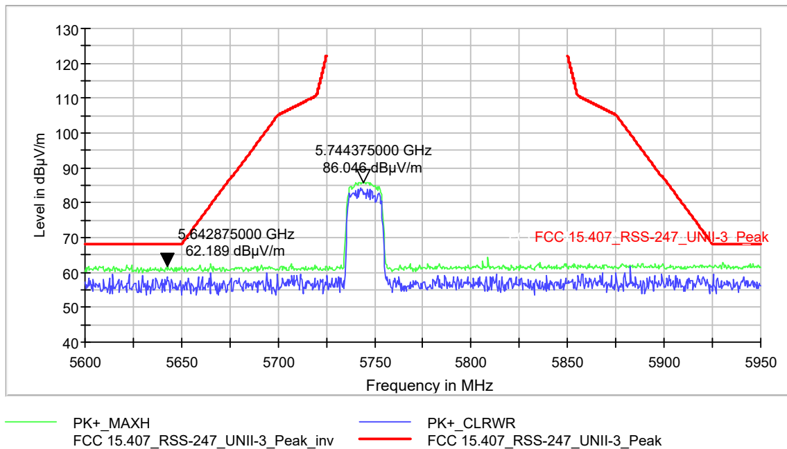
Plot 9-30. Peak Radiated Band Edge Emissions Tx 802.11n (Ch. 149)
