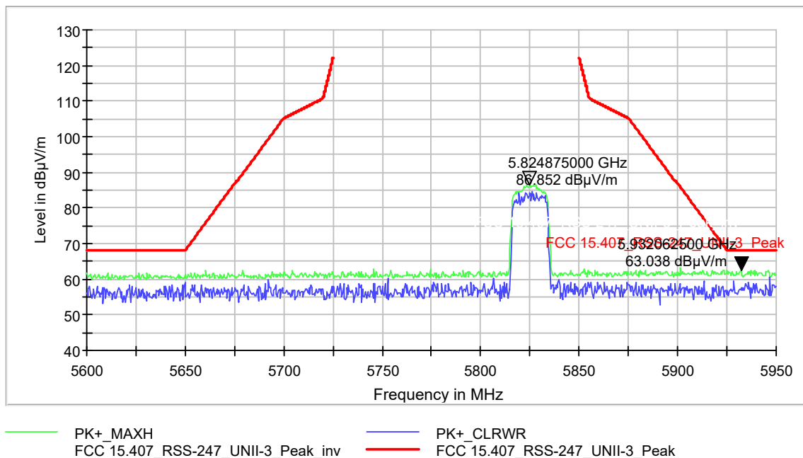
Plot 9-31. Peak Radiated Band Edge Emissions Tx 802.11n (Ch. 165)
