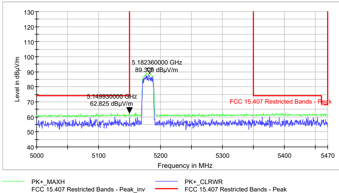
Plot 9-28. Peak Radiated Band Edge Emissions Tx 802.11n (Ch. 36)
