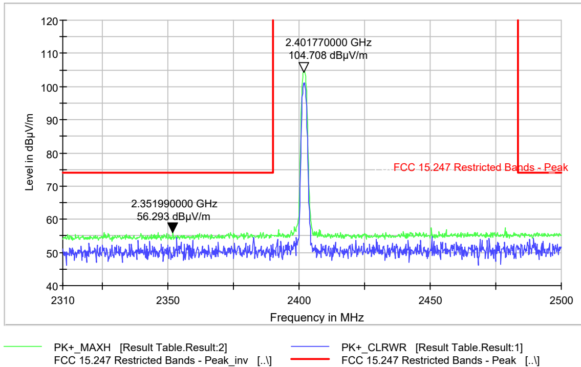
Figure 9-63 Restricted Band Edge 2-DH5 Mode- Ch. 0 (2310-2390MHz) – Peak
