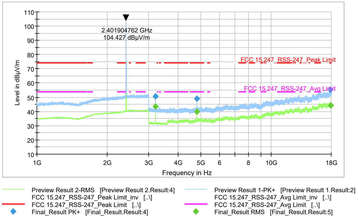
Figure 9-74 Radiated Spurious Emissions (Ch. 0) 2-DH5 (1-18 GHz)
