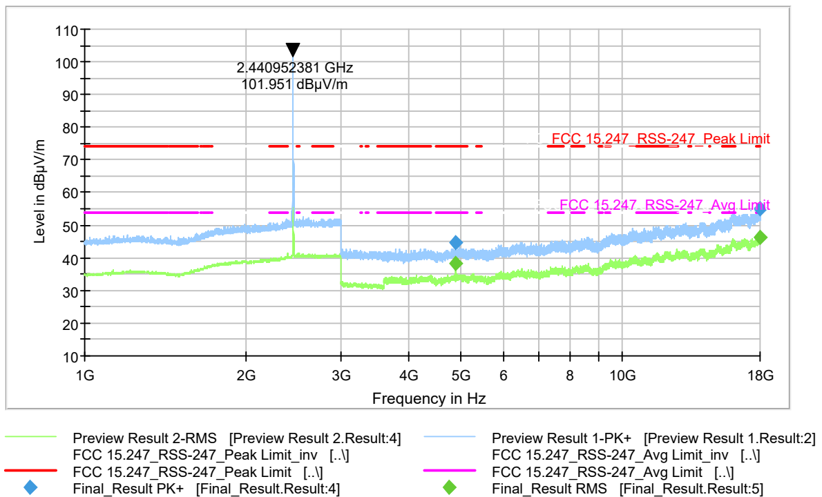
Figure 9-72 Radiated Spurious Emissions (Ch. 39) 1-DH5 (1-18 GHz)
