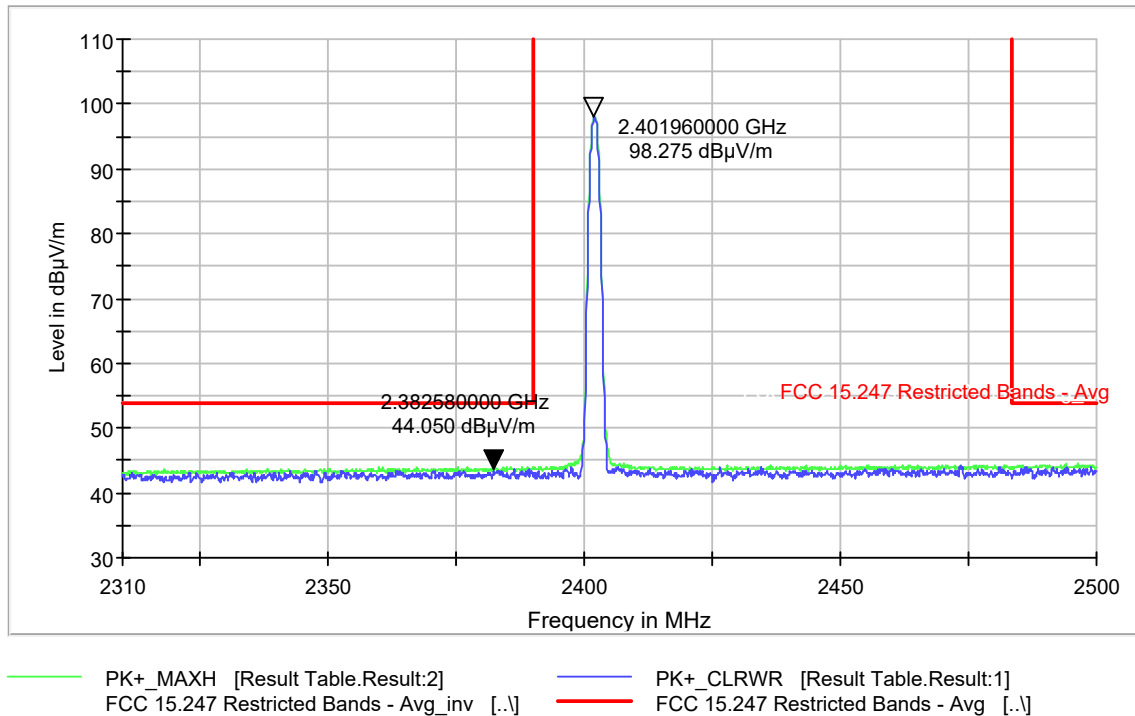
Figure 9-64 Restricted Band Edge 2-DH5 Mode- Ch. 0 (2310-2390MHz) - Average
