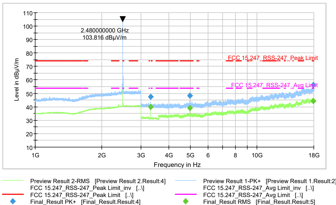
Figure 9-79 Radiated Spurious Emissions (Ch. 78) 3-DH5 (1-18 GHz)
