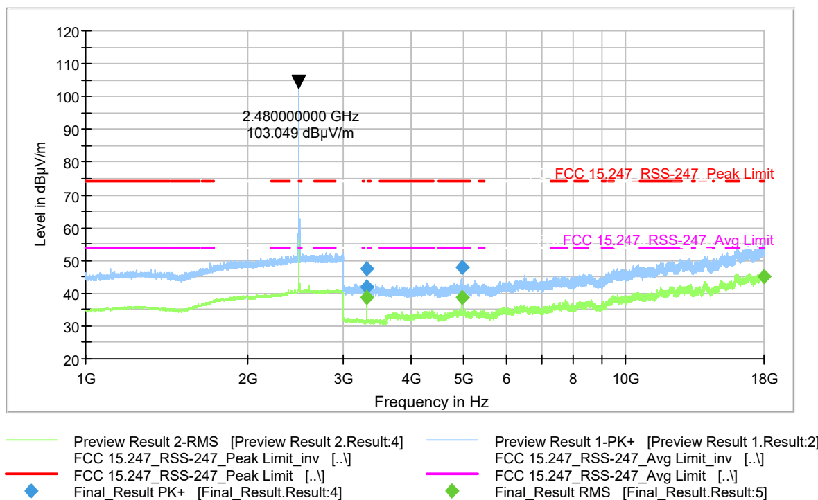
Figure 9-76 Radiated Spurious Emissions (Ch. 78) 2-DH5 (1-18 GHz)
