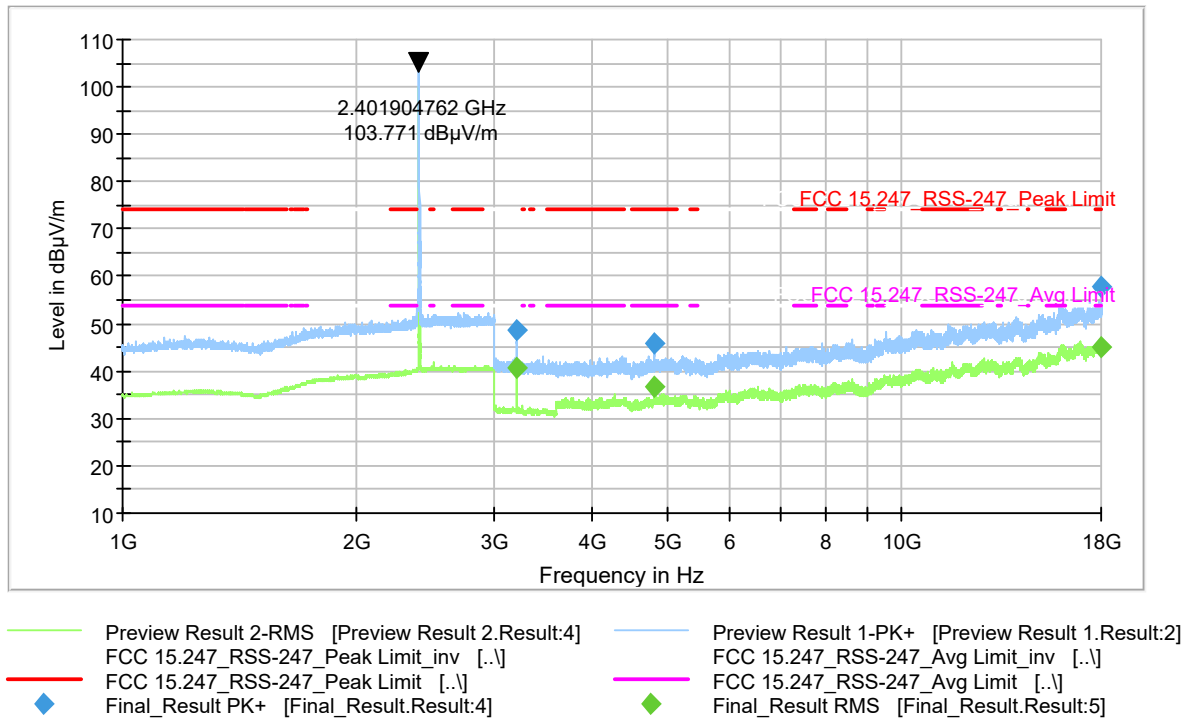
Figure 9-77 Radiated Spurious Emissions (Ch. 0) 3-DH5 (1-18 GHz)
