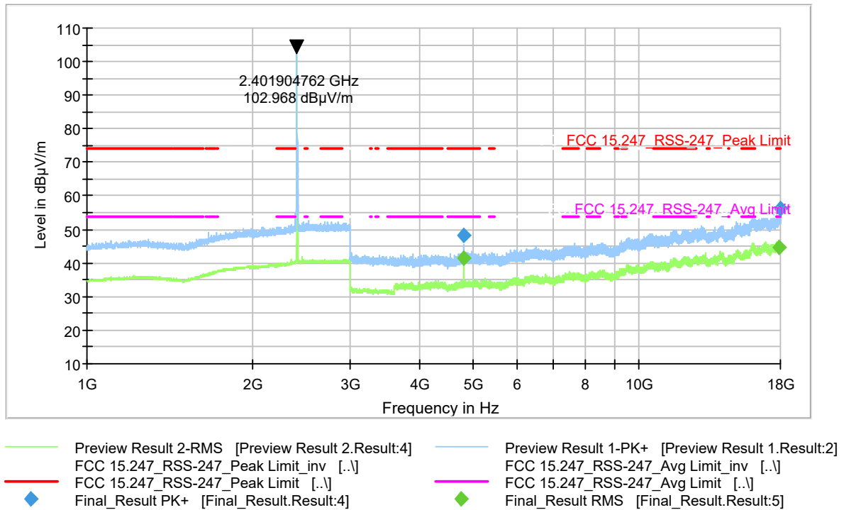
Figure 9-71 Radiated Spurious Emissions (Ch. 0) 1-DH5 (1-18 GHz)
