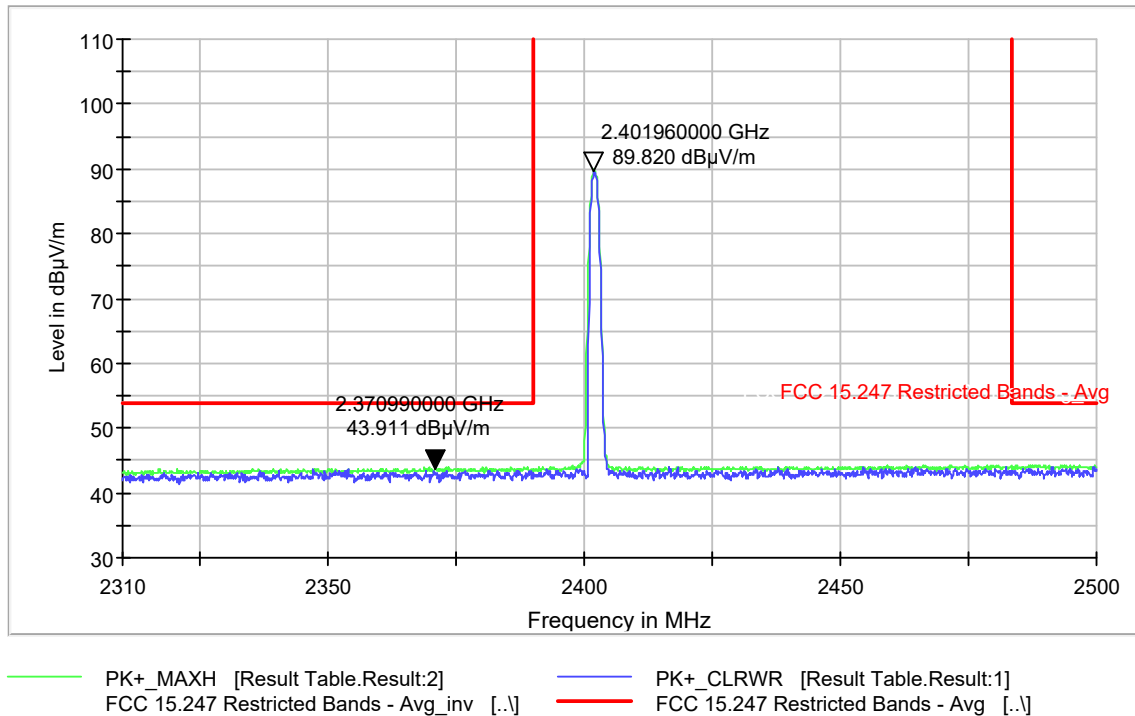
Figure 9-68 Restricted Band Edge 3-DH5 Mode- Ch. 0 (2310-2390MHz) - Average
