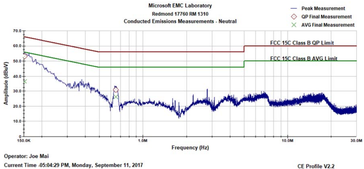
Figure 9-82 AC Line Conducted Emissions- Neutral (150 kHz- 30 MHz)
