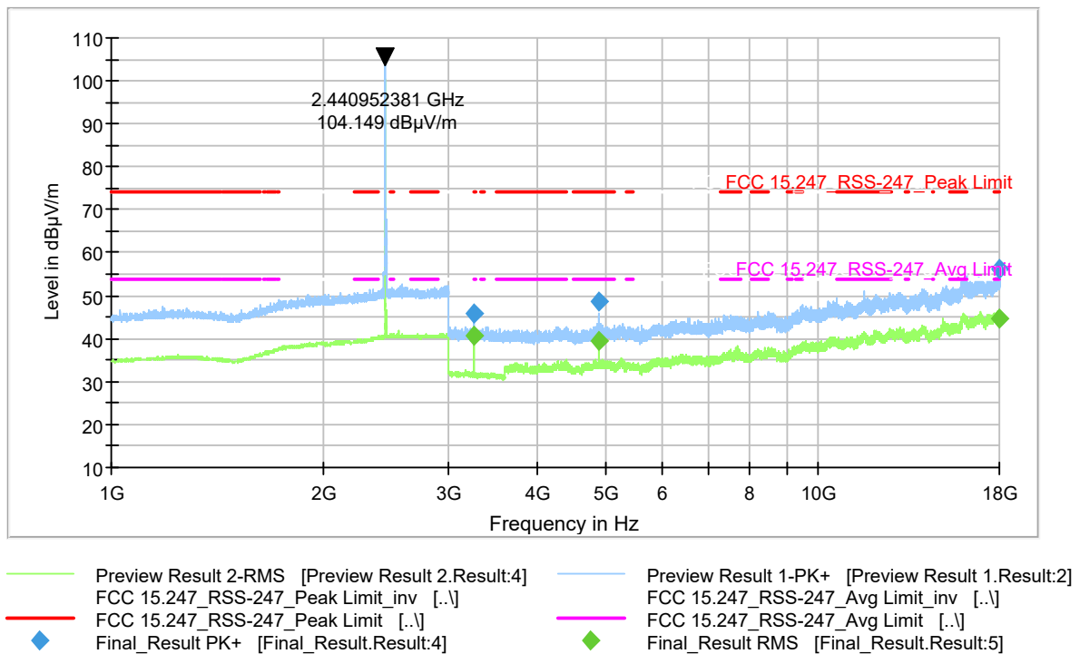
Figure 9-78 Radiated Spurious Emissions (Ch. 39) 3-DH5 (1-18 GHz)
