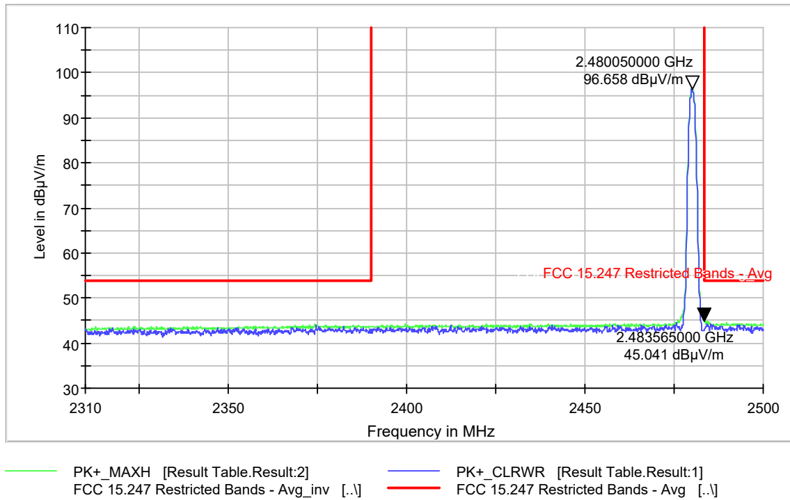
Figure 9-70 Restricted Band Edge 3-DH5 Mode- Ch. 78 (2483.5-2500MHz) - Average
