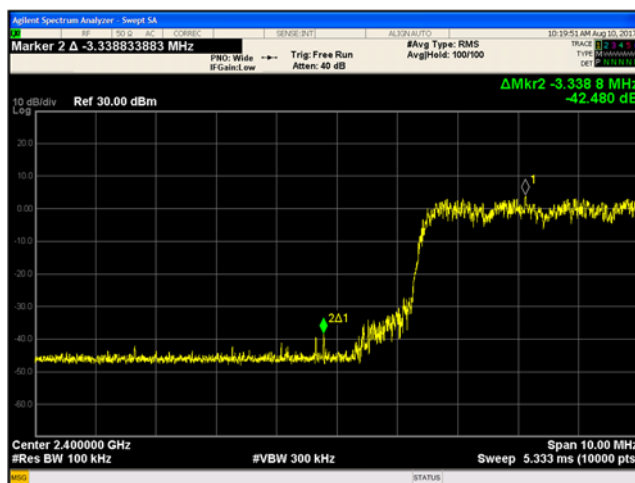
Figure 9-37 Low Channel Band edge 3-DH5 Mode (Hopping enabled)
