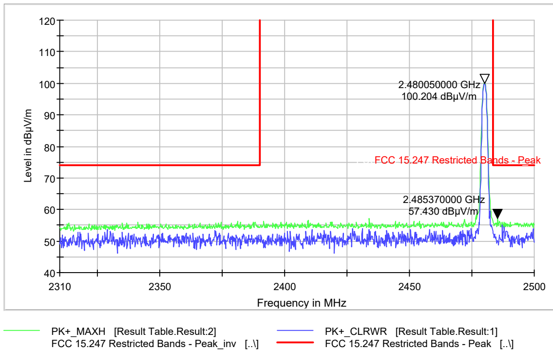
Figure 9-69 Restricted Band Edge 3-DH5 Mode- Ch. 78 (2483.5-2500MHz) – Peak
