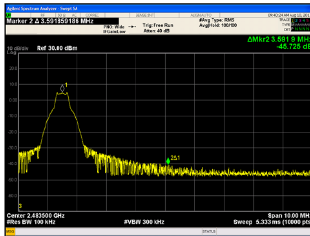
Figure 9-32 High Channel Band edge: 1-DH5 Mode (Hopping disabled)
