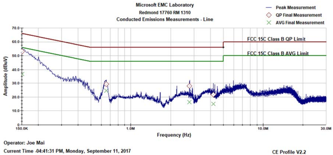
Figure 9-81 AC Line Conducted Emissions- Line (150 kHz- 30 MHz)
