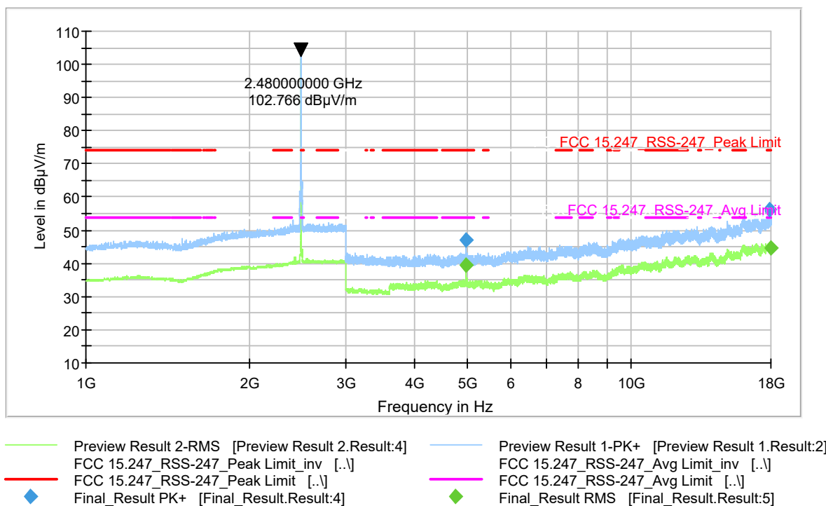
Figure 9-73 Radiated Spurious Emissions (Ch. 78) 1-DH5 (1-18 GHz)
