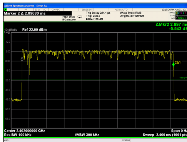
Figure 9-25 Dwell Time - DH5
