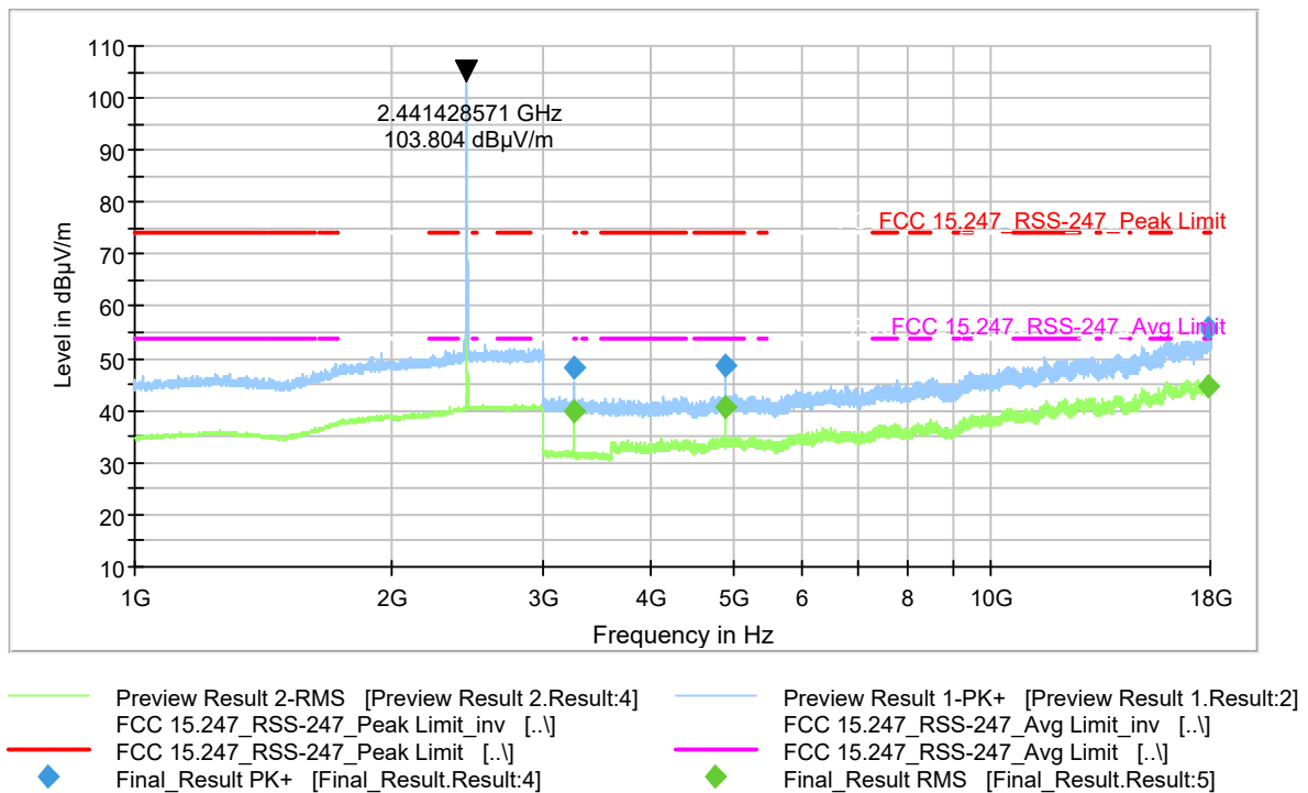
Figure 9-75 Radiated Spurious Emissions (Ch. 39) 2-DH5 (1-18 GHz)
