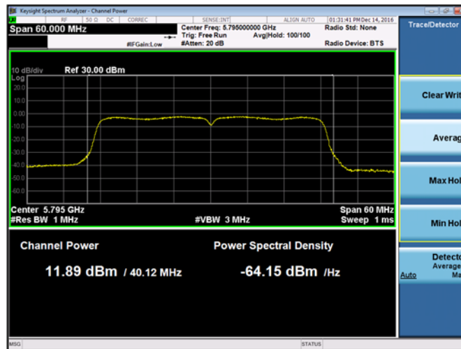
Plot 9-226. Maximum Conducted Output Power Chain B 802.11n HT40 (Ch. 159)
