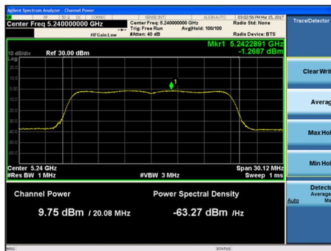
Plot 9-231. Maximum Conducted Output Power and PSD Chain A 802.11ac VHT20 (Ch. 48)
