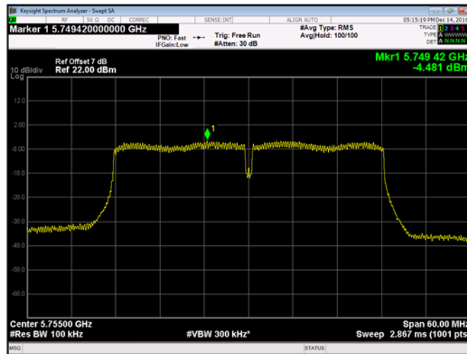
Plot 9-216. Maximum Power Spectral Density Chain A 802.11n HT40 (Ch. 151)
