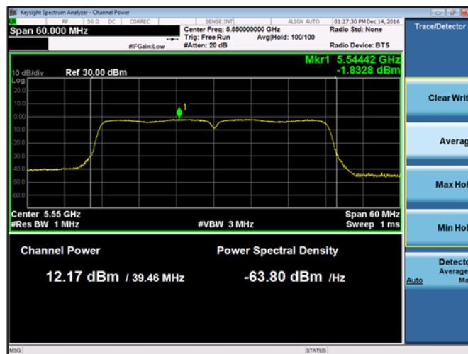
Plot 9-223. Maximum Conducted Output Power and PSD Chain B 802.11n HT40 (Ch. 110)
