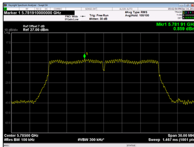
Plot 9-257. Maximum Power Spectral Density Chain B 802.11ac VHT20 (Ch. 157)
