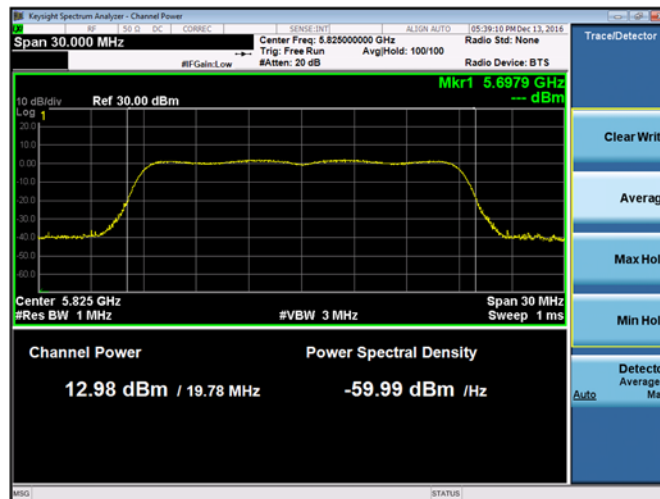
Plot 9-240. Maximum Output Power Chain A 802.11ac VHT20 (Ch. 165)
