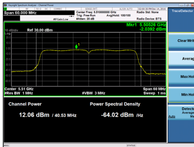
Plot 9-263. Max Conducted Output Power and PSD Chain A 802.11ac VHT40 (Ch. 102)
