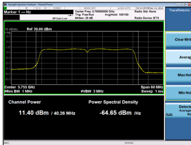
Plot 9-266. Max Conducted Output Power Chain A 802.11ac VHT40 (Ch. 151)
