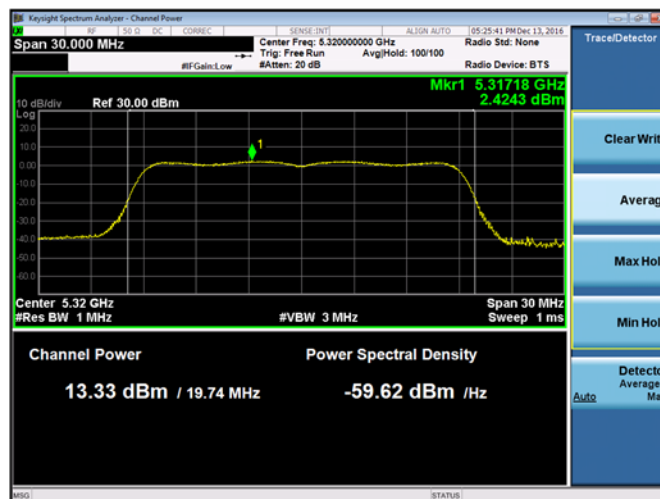
Plot 9-234. Maximum Output Power and PSD Chain A 802.11ac VHT20 (Ch. 64)
