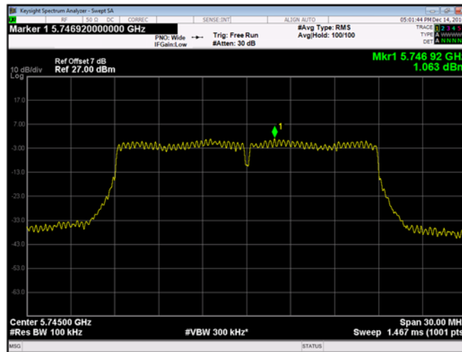
Plot 9-256. Maximum Power Spectral Density Chain B 802.11ac VHT20 (Ch. 149)
