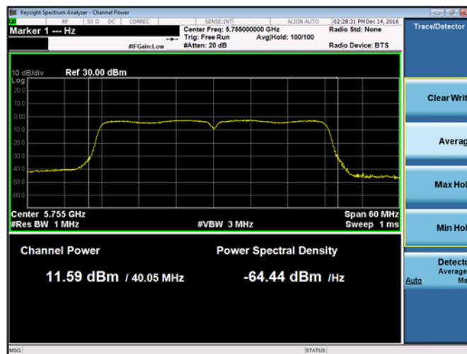
Plot 9-214. Maximum Conducted Output Power Chain A 802.11n HT40 (Ch. 151)
