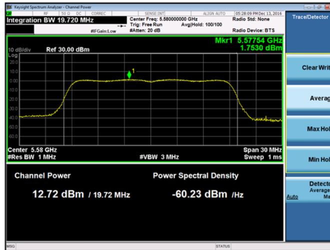
Plot 9-236. Maximum Output Power and PSD Chain A 802.11ac VHT20 (Ch. 116)
