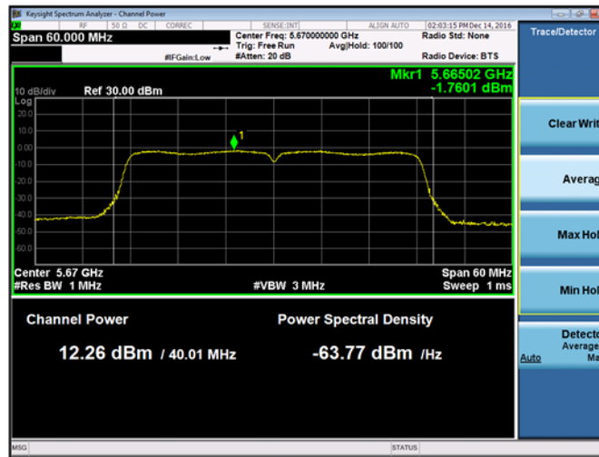
Plot 9-265. Max Conducted Output Power and PSD Chain A 802.11ac VHT40 (Ch. 134)
