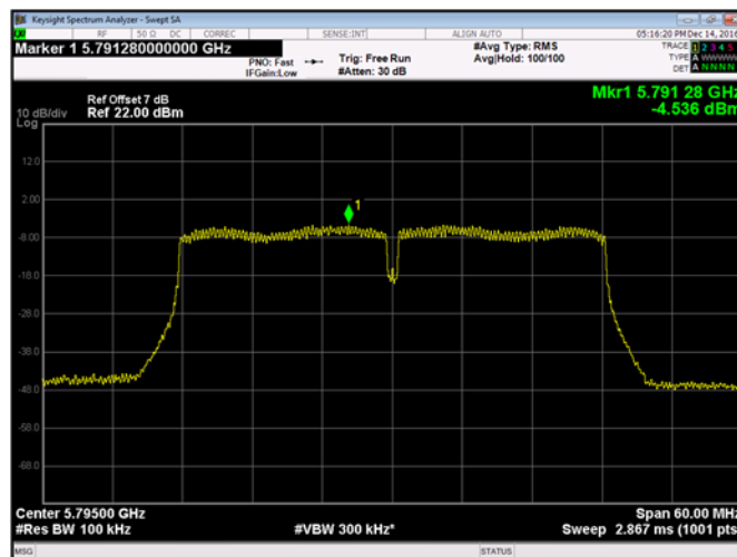
Plot 9-217. Maximum Power Spectral Density Chain A 802.11n HT40 (Ch. 159)
