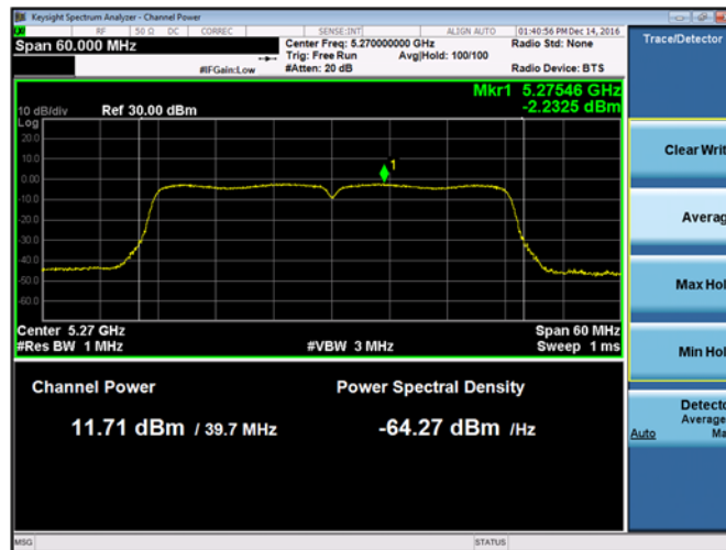
Plot 9-272. Maximum Conducted Output Power and PSD Chain B 802.11ac VHT40 (Ch. 54)
