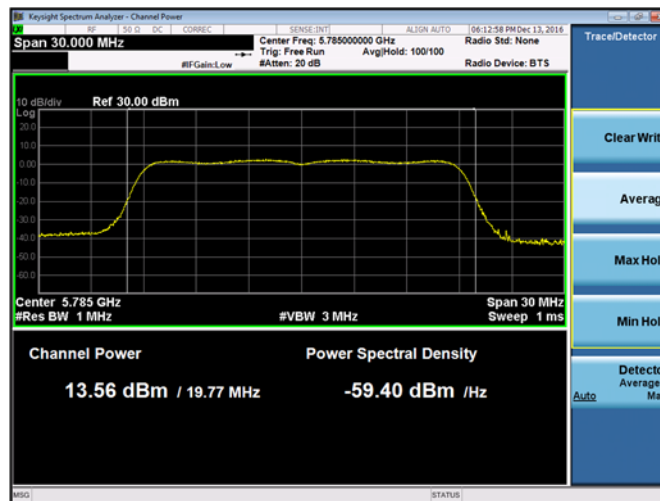
Plot 9-254. Maximum Conducted Output Power Chain B 802.11ac VHT20 (Ch. 157)
