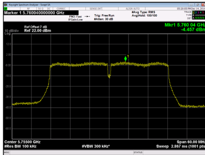
Plot 9-268. Maximum Power Spectral Density Chain A 802.11ac VHT40 (Ch. 151)
