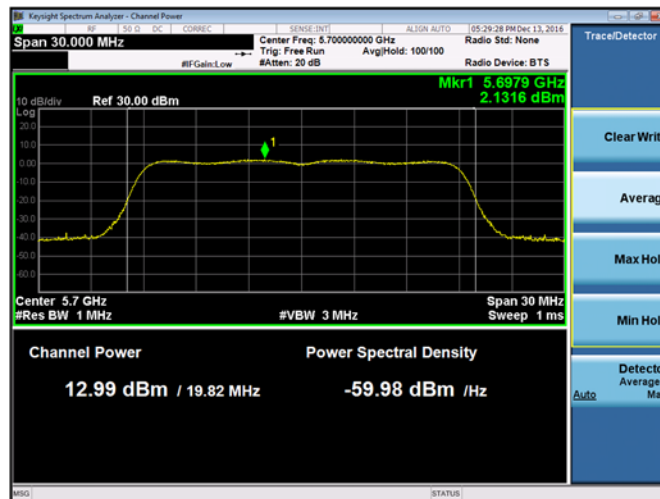
Plot 9-237. Maximum Output Power and PSD Chain A 802.11ac VHT20 (Ch. 140)
