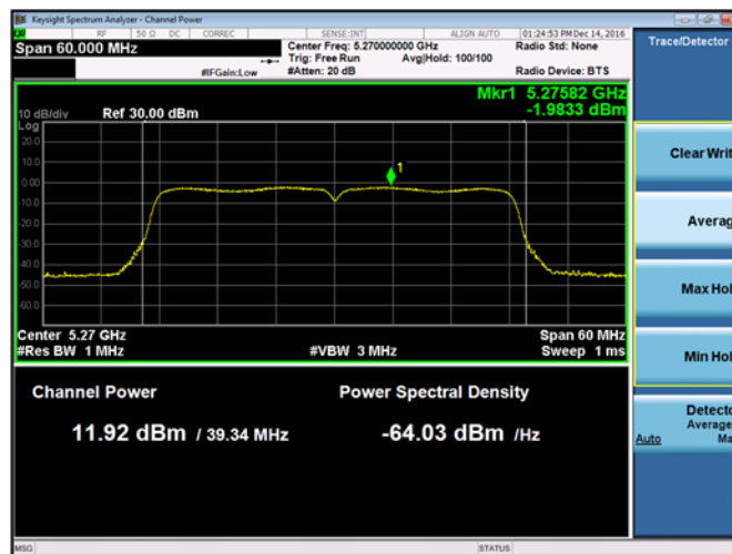
Plot 9-220. Maximum Conducted Output Power and PSD Chain B 802.11n HT40 (Ch. 54)
