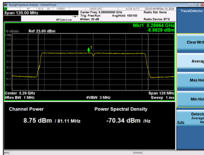
Plot 9-282. Maximum Conducted Output Power and PSD Chain A 802.11ac VHT80 (Ch. 58)
