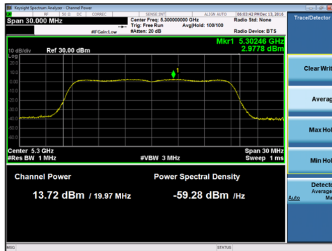
Plot 9-248. Maximum Conducted Output Power and PSD Chain B 802.11ac VHT20 (Ch. 60)
