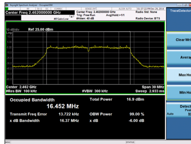
Plot 9-11 Chain A DTS Bandwidth 802.11g mode - Ch.11 (2462 MHz)
