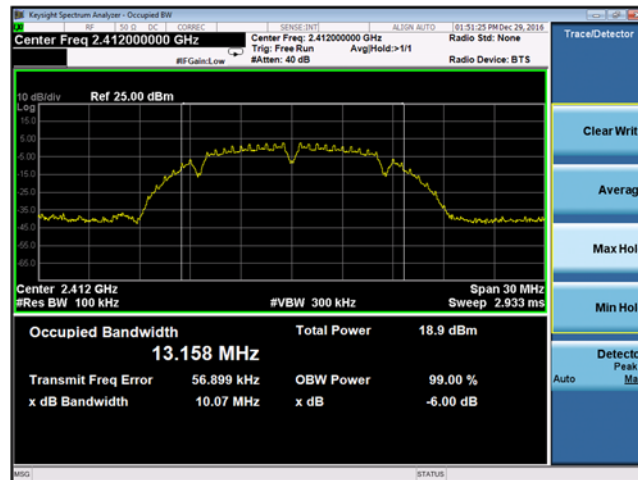
Plot 9-19 Chain B DTS Bandwidth 802.11b mode - Ch.1 (2412 MHz)
