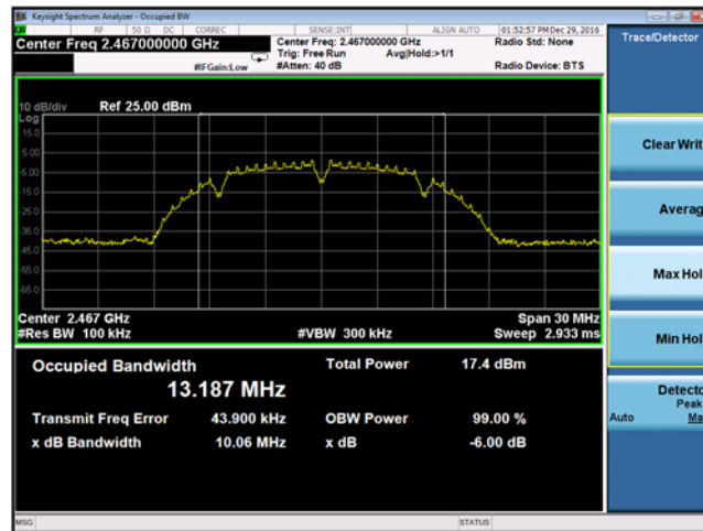
Plot 9-22 Chain B DTS Bandwidth 802.11b mode - Ch.12 (2467 MHz)
