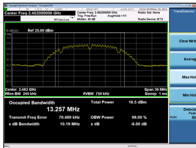
Plot 9-51 Chain B 99% Bandwidth 802.11b - Ch.11 (2462 MHz)
