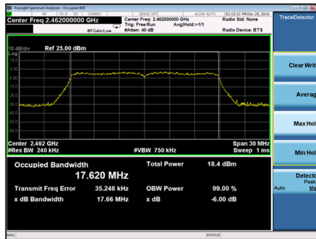
Plot 9-61 Chain B 99% Bandwidth 802.11n - Ch.11 (2462 MHz)
