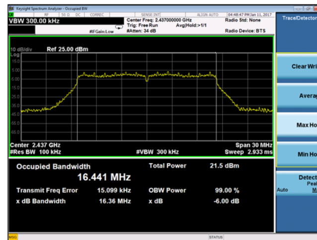
Plot 9-10 Chain A DTS Bandwidth 802.11g mode - Ch.6 (2437 MHz)
