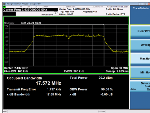
Plot 9-30 Chain B DTS Bandwidth 802.11n mode - Ch.6 (2437 MHz)
