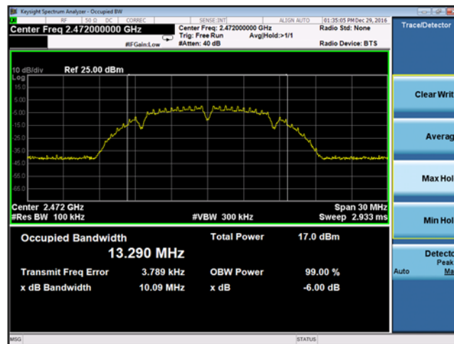
Plot 9-8 Chain A DTS Bandwidth 802.11b mode - Ch.13 (2472 MHz)
