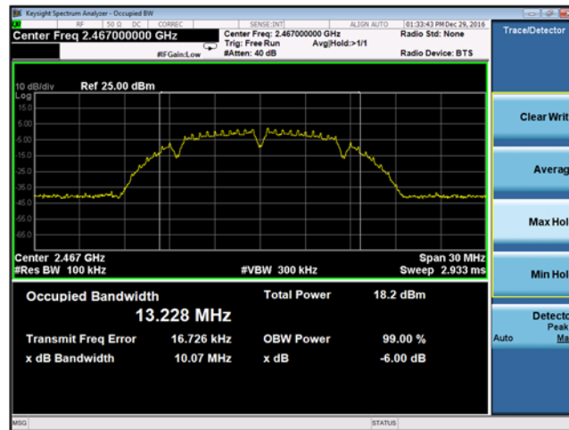
Plot 9-7 Chain A DTS Bandwidth 802.11b mode - Ch.12 (2467 MHz)
