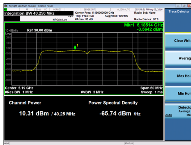
Plot 9-166. Maximum Conducted Output Power and PSD Chain B 802.11n HT40 (Ch. 38)
