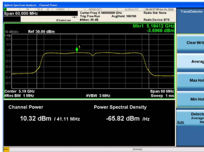
Plot 9-155. Maximum Conducted Output Power and PSD Chain A 802.11n HT40 (Ch. 38)
