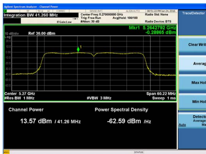
Plot 9-157. Maximum Conducted Output Power and PSD Chain A 802.11n HT40 (Ch. 54)
