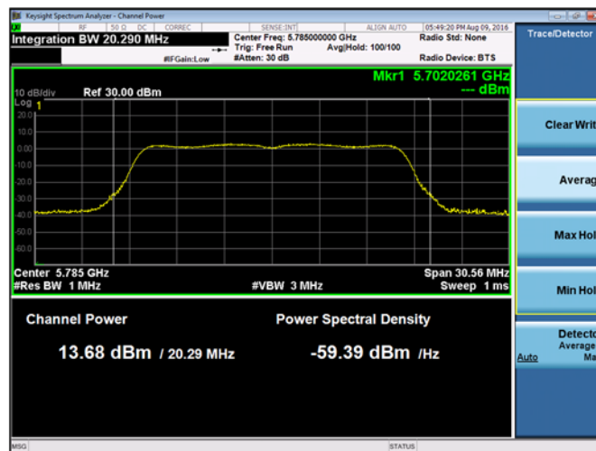
Plot 9-105. Maximum Conducted Output Power Chain A 802.11a (Ch. 157)
