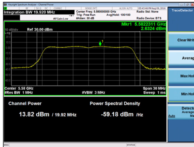
Plot 9-102. Maximum Conducted Output Power and PSD Chain A 802.11a (Ch. 116)
