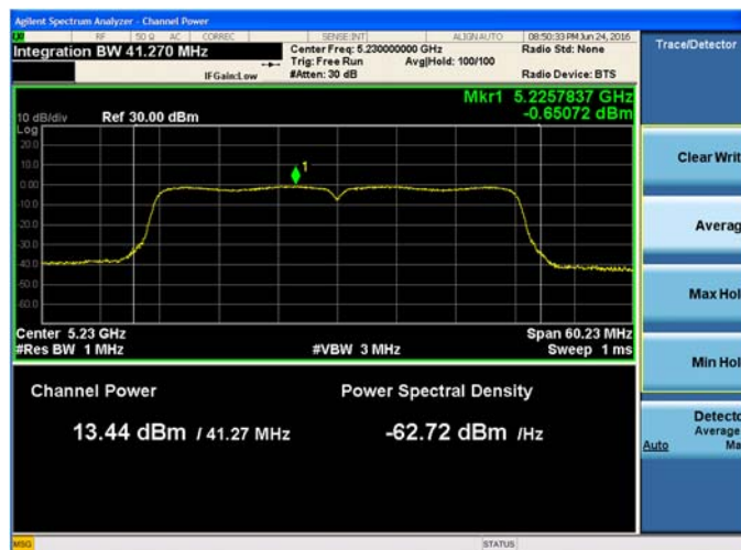
Plot 9-156. Maximum Conducted Output Power and PSD Chain A 802.11n HT40 (Ch. 46)
