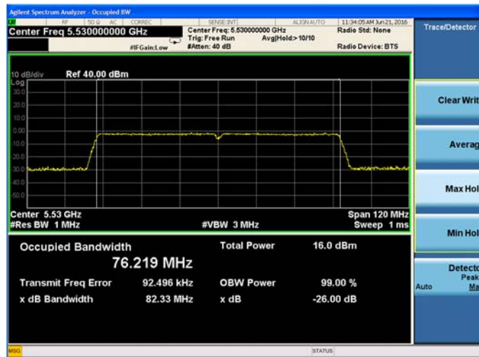
Plot 9-69. 26-dB Emission Bandwidth and 99% OBW Chain A 802.11ac VHT80 (Ch. 106)
