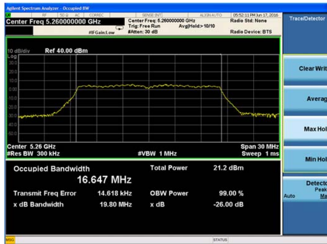
Plot 9-16. 26-dB Emission Bandwidth and 99% OBW Chain B 802.11a (Ch. 52)
