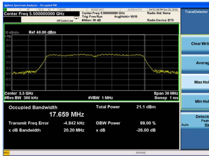
Plot 9-43. 26-dB Emission Bandwidth and 99% OBW Chain B 802.11n HT20 (Ch. 100)
