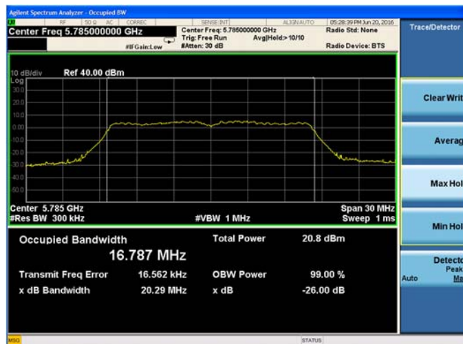
Plot 9-11. 26-dB Emission Bandwidth and 99% OBW Chain A 802.11a (Ch. 157)
