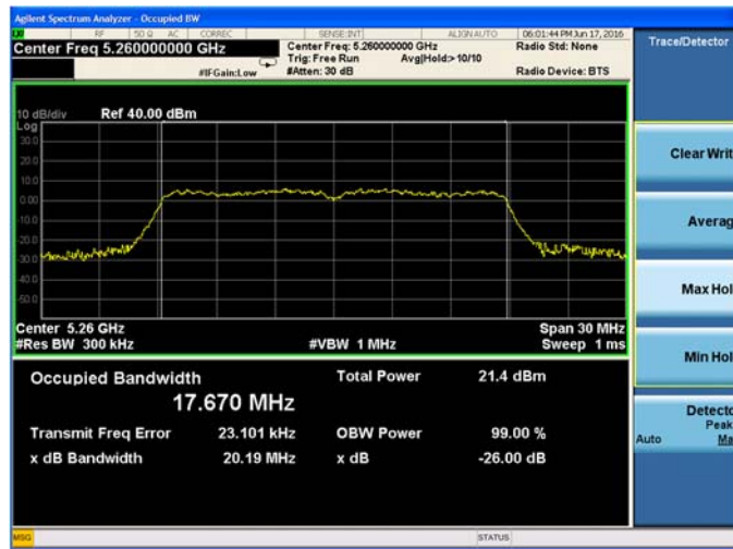
Plot 9-40. 26-dB Emission Bandwidth and 99% OBW Chain B 802.11n HT20 (Ch. 52)
