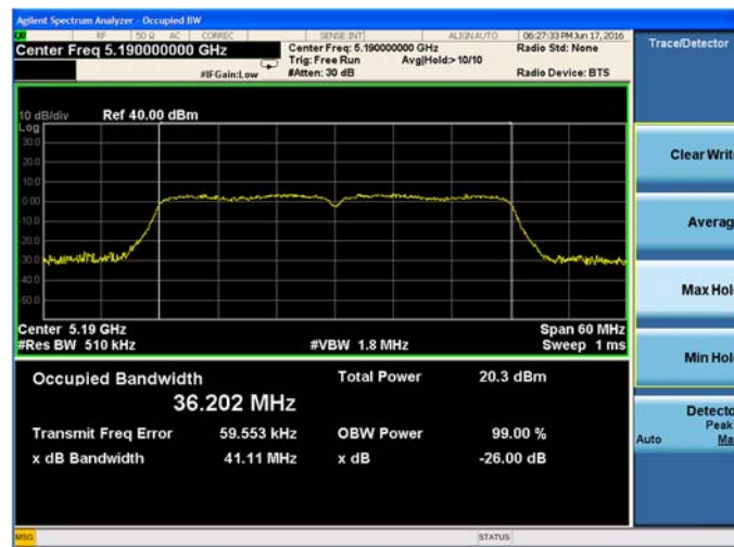
Plot 9-49. 26-dB Emission Bandwidth and 99% OBW Chain A 802.11n HT40 (Ch. 38)
