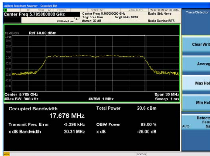
Plot 9-35. 26-dB Emission Bandwidth and 99% OBW Chain A 802.11n HT20 (Ch. 157)
