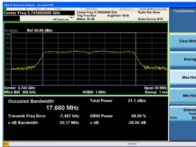
Plot 9-46. 26-dB Emission Bandwidth and 99% OBW Chain B 802.11n HT20 (Ch. 149)
