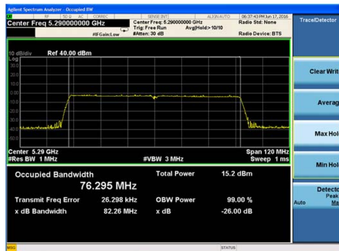
Plot 9-68. 26-dB Emission Bandwidth and 99% OBW Chain A 802.11ac VHT80 (Ch. 58)
