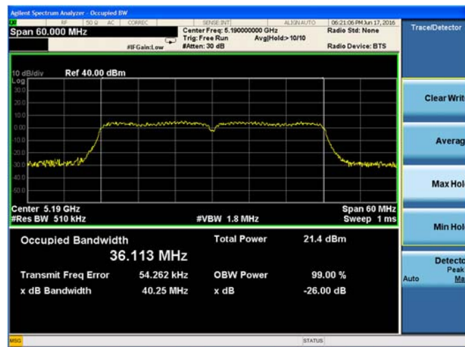
Plot 9-58. 26-dB Emission Bandwidth and 99% OBW Chain B 802.11n HT40 (Ch. 38)
