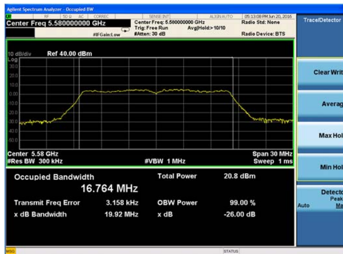
Plot 9-8. 26-dB Emission Bandwidth and 99% OBW Chain A 802.11a (Ch. 116)
