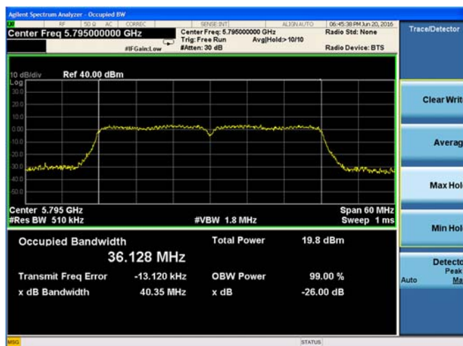
Plot 9-66. 26-dB Emission Bandwidth and 99% OBW Chain B 802.11n HT40 (Ch. 159)
