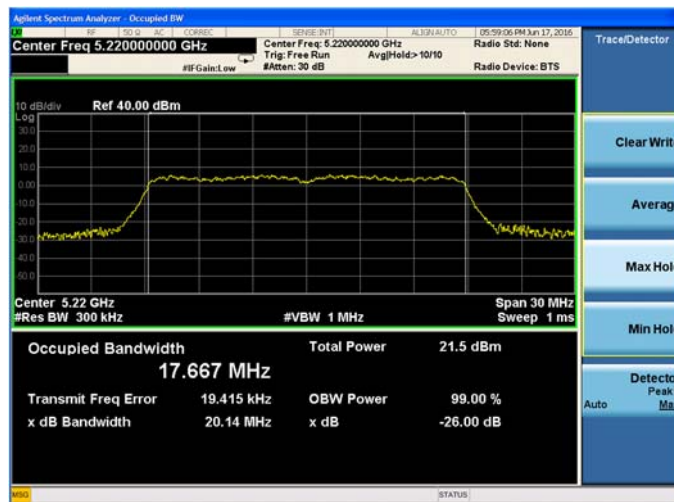
Plot 9-38. 26-dB Emission Bandwidth and 99% OBW Chain B 802.11n HT20 (Ch. 44)
