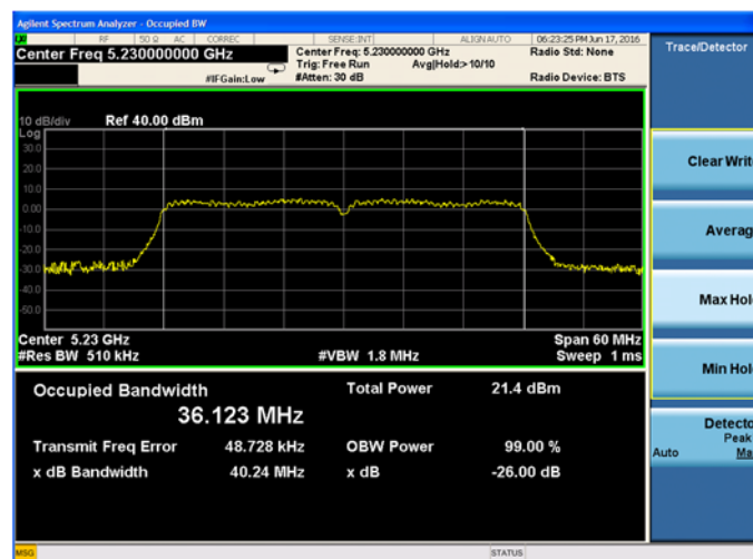
Plot 9-59. 26-dB Emission Bandwidth and 99% OBW Chain B 802.11n HT40 (Ch. 46)
