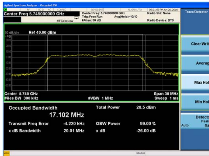
Plot 9-10. 26-dB Emission Bandwidth and 99% OBW Chain A 802.11a (Ch. 149)
