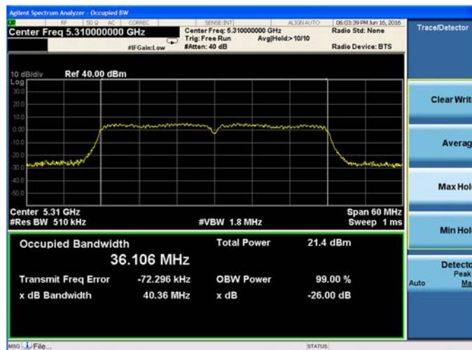
Plot 9-61. 26-dB Emission Bandwidth and 99% OBW Chain B 802.11n HT40 (Ch. 62)
