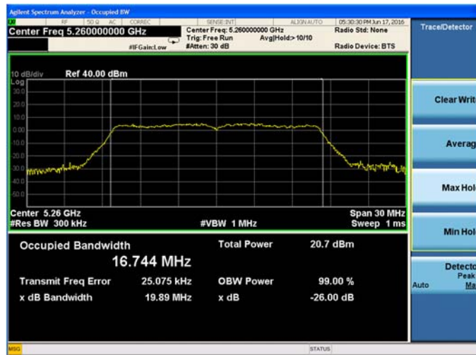
Plot 9-4. 26-dB Emission Bandwidth and 99% OBW Chain A 802.11a (Ch. 52)
