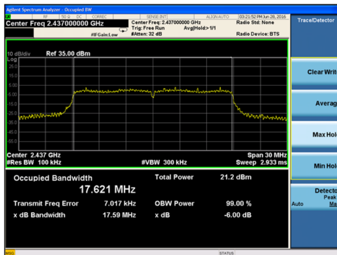
Plot 9-25 Chain B DTS Bandwidth 802.11n mode - Ch.6 (2437 MHz)
