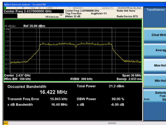
Plot 9-21 Chain B DTS Bandwidth 802.11g mode - Ch.6 (2437 MHz)
