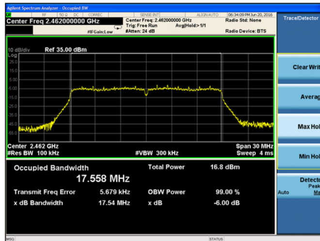
Plot 9-14 Chain A DTS Bandwidth 802.11n mode - Ch.11 (2462 MHz)
