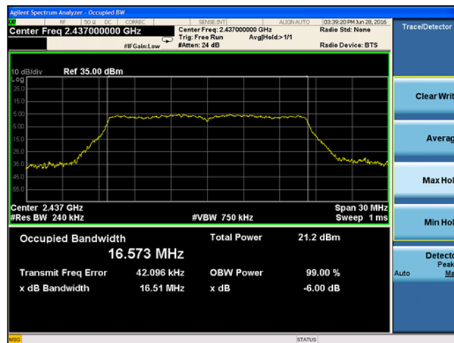
Plot 9-45 Chain B 99% Bandwidth 802.11g - Ch.6 (2437 MHz)
