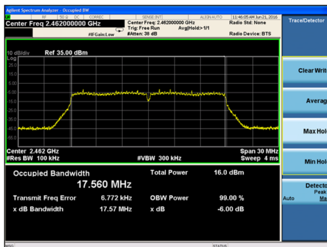
Plot 9-26 Chain B DTS Bandwidth 802.11n mode - Ch.11 (2462 MHz)
