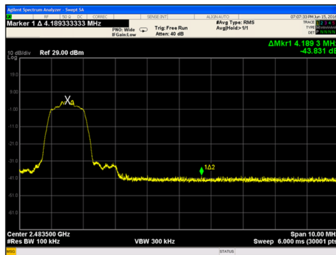
Plot 9-31. High Channel Band edge: 2-DH5 Mode (Hopping disabled)
