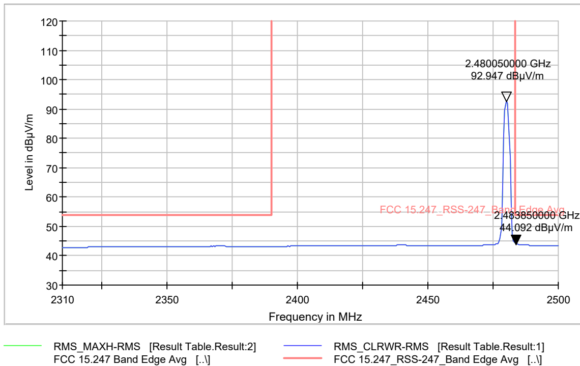
Plot 9-66. Restricted Band Edge 3-DH5 Mode- Ch. 78 (2483.5-2500MHz) - Average
