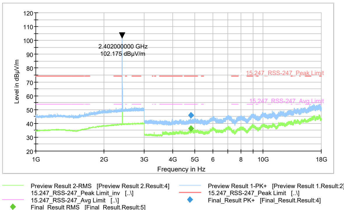
Plot 9-68. Radiated Spurious Emissions (Ch. 0) (1-18 GHz)
