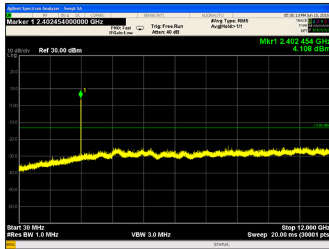
Plot 9-35. Conducted Spurious Emissions 30-12000 MHz: 1-DH5 Mode (Ch. 0)
