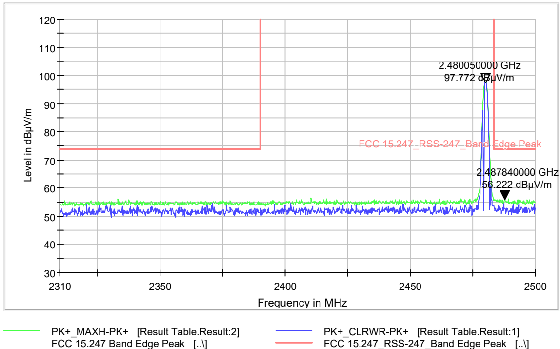
Plot 9-65. Restricted Band Edge 3-DH5 Mode- Ch. 78 (2483.5-2500MHz) – Peak
