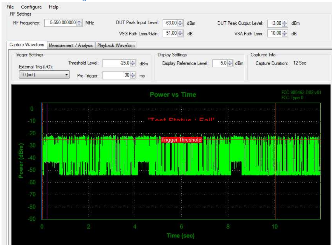
Figure 2. Channel Loading
