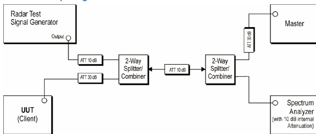
Fig.1. Test Setup for Antenna port conducted measurements
