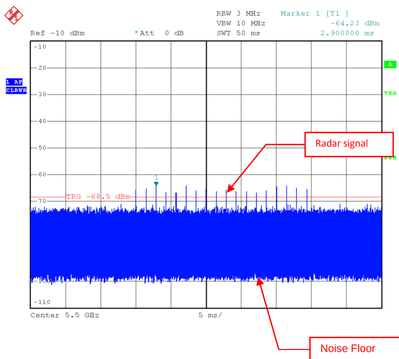
Radar Signal 0
