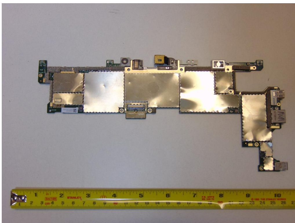
Figure 4 Motherboard (front)
