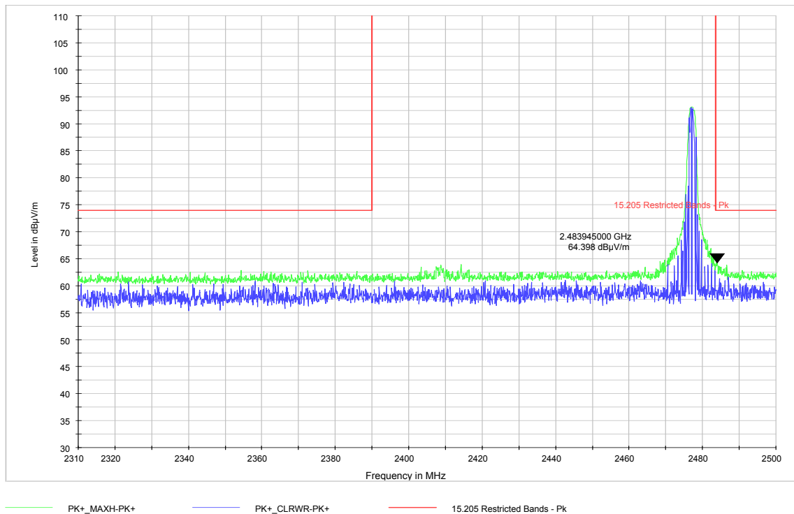
Figure 9-19 Radiated Restricted Band Edge (2477MHz) Peak detector
