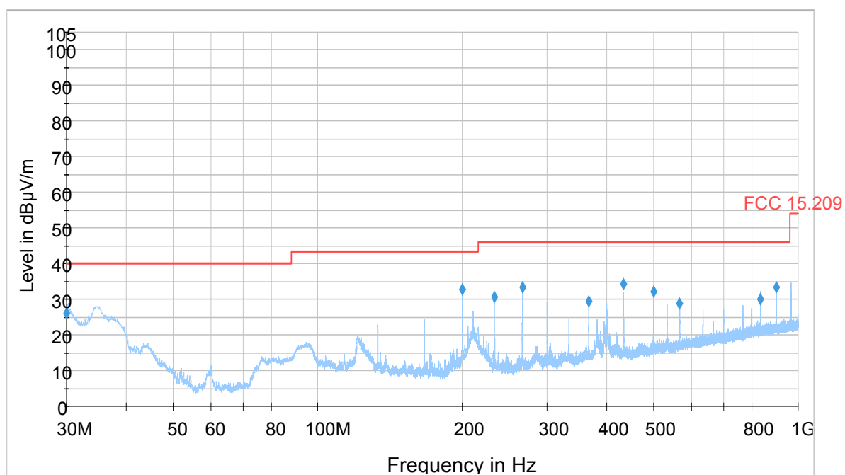
Figure 9-9 Radiated Spurious Emissions (2440 MHz) (30MHz - 1GHz)
