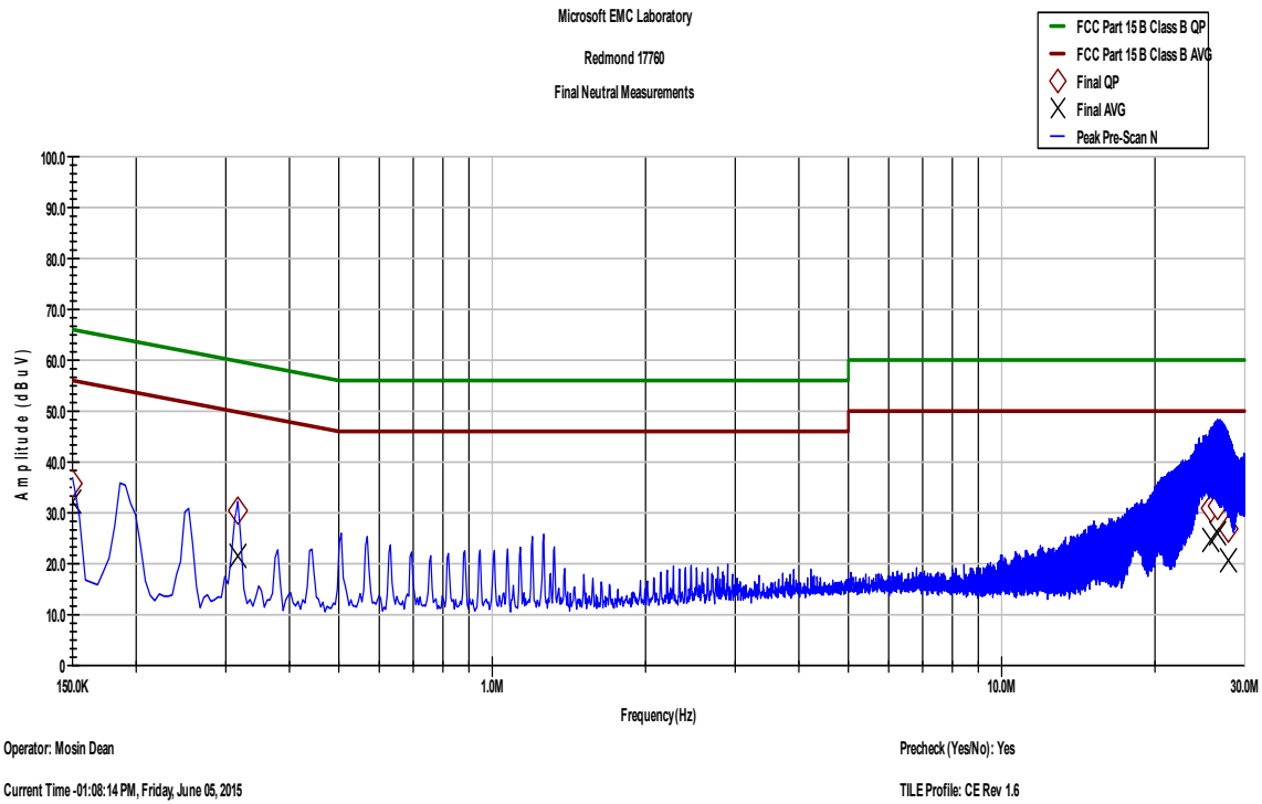
Figure 9-22 AC Conducted Emissions - Neutral (150 kHz-30MHz)
