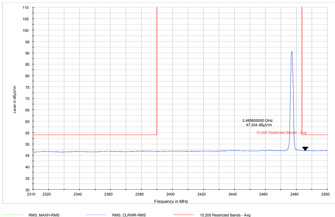
Figure 9-20 Radiated Restricted Band Edge (2477 MHz) Average detector
