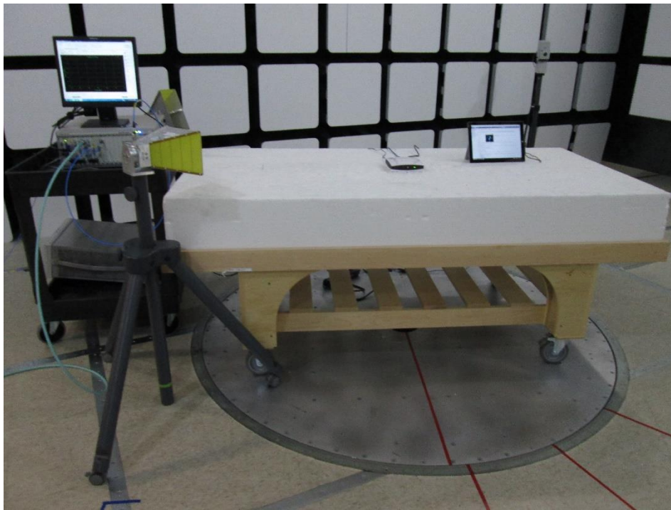
Figure 1-1 Radiated Test Setup
