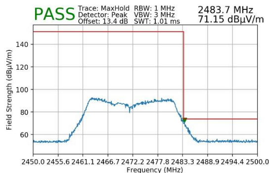
Plot 7-26. Restricted Upper Band Edge Measurement MIMO (Peak)
