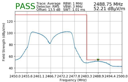
Plot 7-23. Restricted Upper Band Edge Measurement MIMO (Average)
