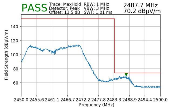
Plot 7-22. Restricted Upper Band Edge Measurement MIMO (Peak)
