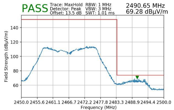
Plot 7-24. Restricted Upper Band Edge Measurement MIMO (Peak)
