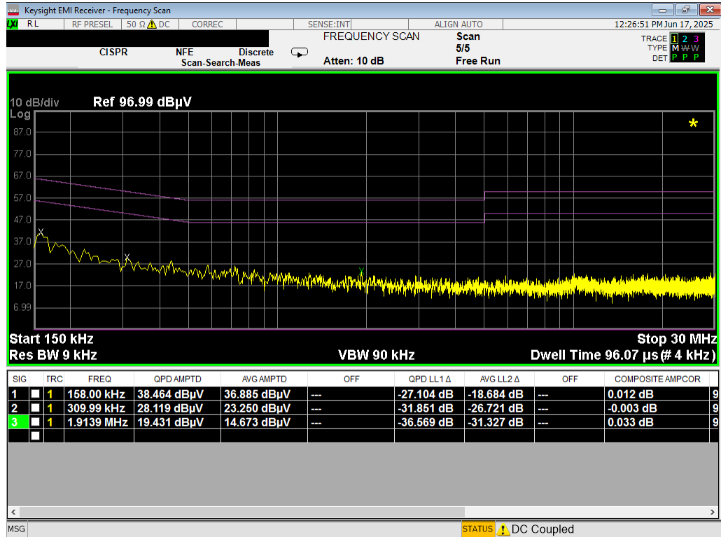
Plot 7-27. Line Conducted Plot with 802.11b – Ch.6 (L1)
