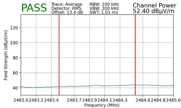
Plot 7-21. Restricted Upper Band Edge Measurement MIMO (Average)
