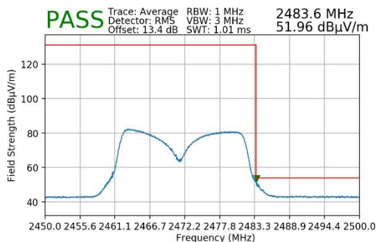
Plot 7-25. Restricted Upper Band Edge Measurement MIMO (Average)
