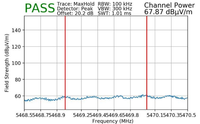
Plot 7-22. Lower Band Edge Plot MIMO (Peak – UNII Band 2C)
