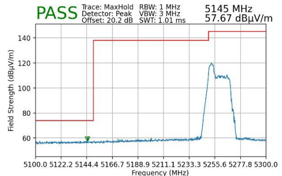
Plot 7-20. Lower Band Edge Plot MIMO (Peak – UNII Band 2A)
