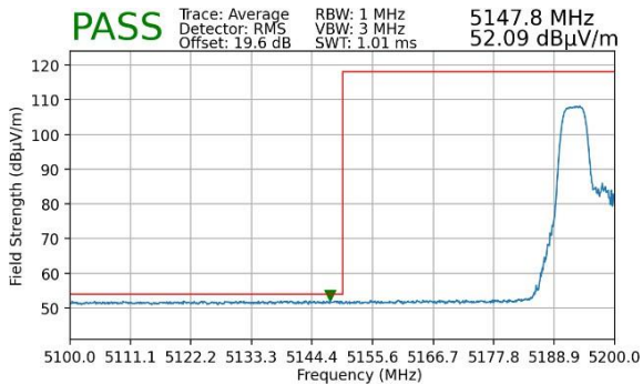
Plot 7-15. Lower Band Edge Plot MIMO (Average – UNII Band 1)
