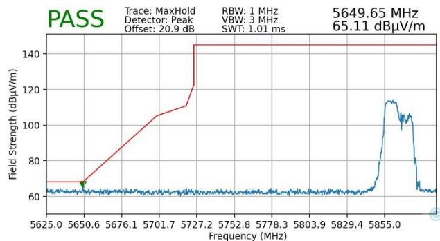
Plot 7-25. Lower Band Edge Plot MIMO (Peak – UNII Band 4)
