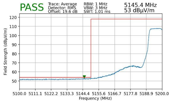
Plot 7-17. Lower Band Edge Plot MIMO (Average – UNII Band 1)
