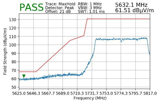
Plot 7-35. Lower Band Edge Plot MIMO (Peak – UNII Band 3)
