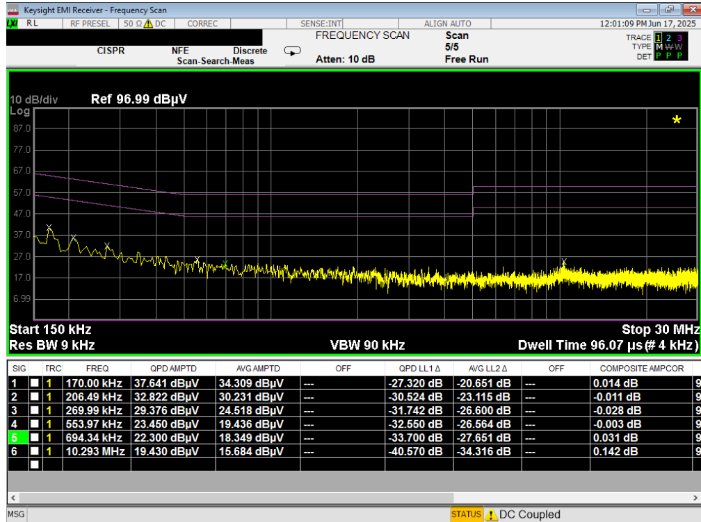
Plot 7-44. Line Conducted Plot with 802.11a UNII Band 3 – Ch.157 (L1)
