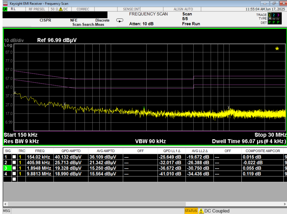
Plot 7-42. Line Conducted Plot with 802.11a UNII Band 2C – Ch.120 (L1)
