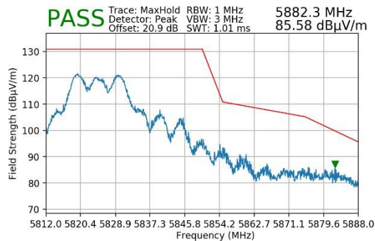
Plot 7-24. Upper Band Edge Plot MIMO (Peak – UNII Band 3)
