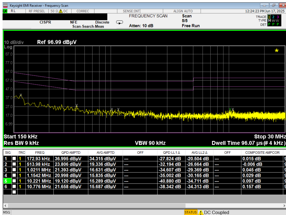
Plot 7-39. Line Conducted Plot with 802.11a UNII Band 1 – Ch.40 (N)
