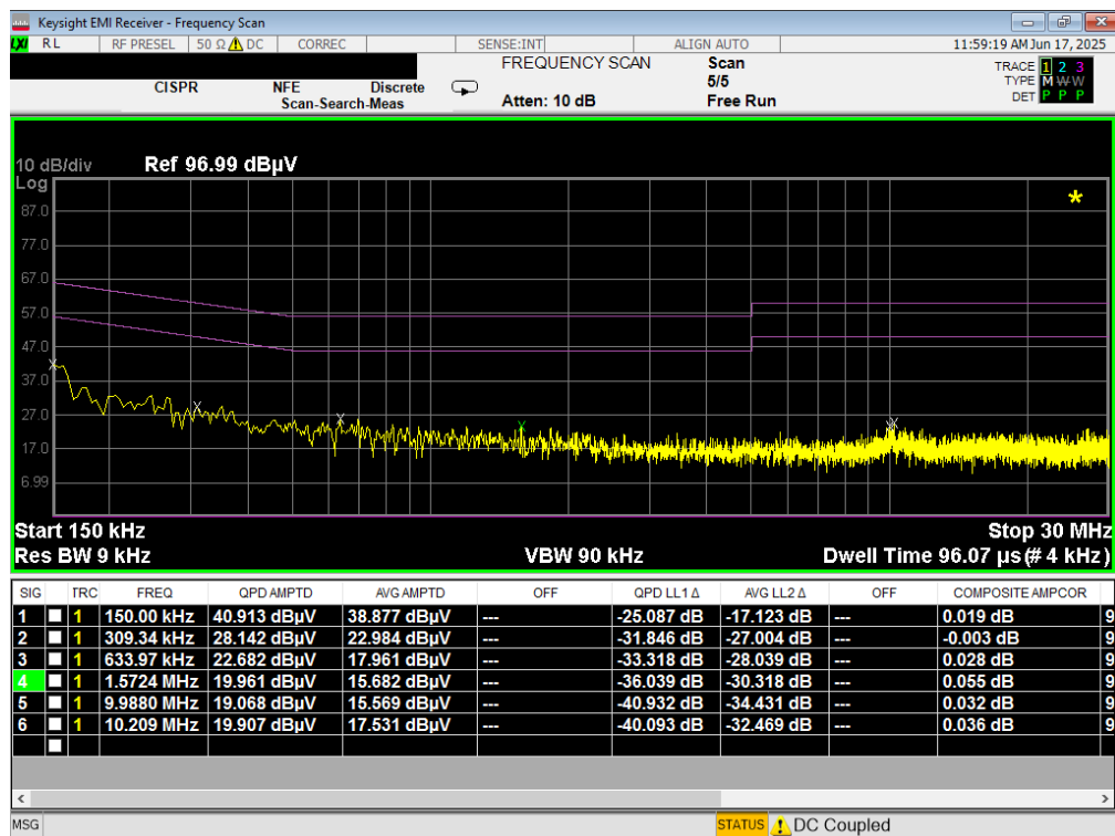
Plot 7-45. Line Conducted Plot with 802.11a UNII Band 3 – Ch.157 (N)
