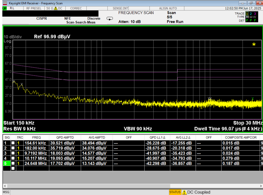
Plot 7-46. Line Conducted Plot with 802.11a UNII Band 4 – Ch.173 (L1)
