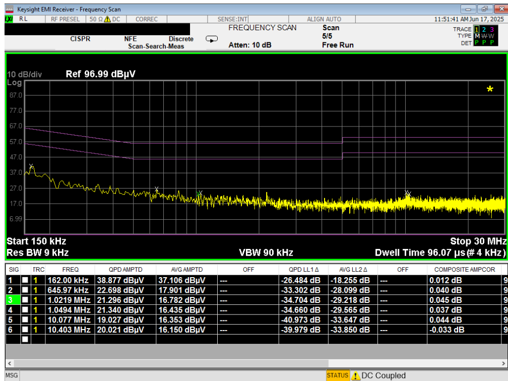
Plot 7-41. Line Conducted Plot with 802.11a UNII Band 2A – Ch.56 (N)
