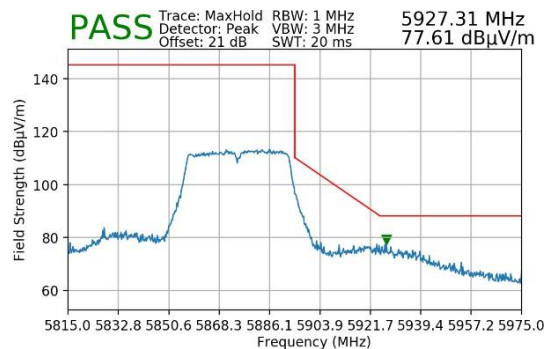
Plot 7-34. Upper Band Edge Plot MIMO (Peak – UNII Band 4)
