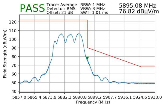
Plot 7-26. Upper Band Edge Plot MIMO (Average – UNII Band 4)
