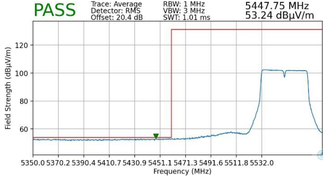
Plot 7-30. Lower Band Edge Plot MIMO (Average – UNII Band 2C)
