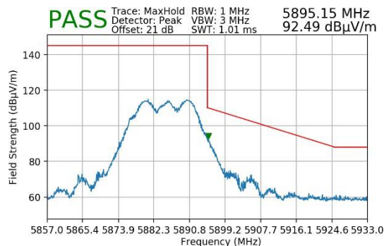
Plot 7-27. Upper Band Edge Plot MIMO (Peak – UNII Band 4)
