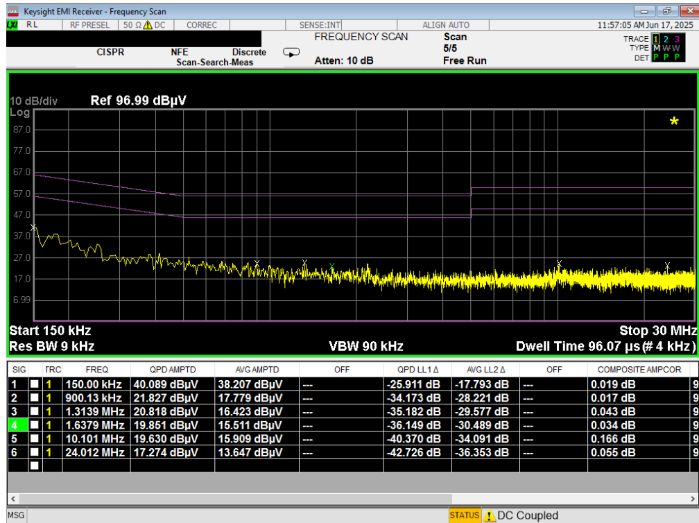
Plot 7-43. Line Conducted Plot with 802.11a UNII Band 2C – Ch.120 (N)
