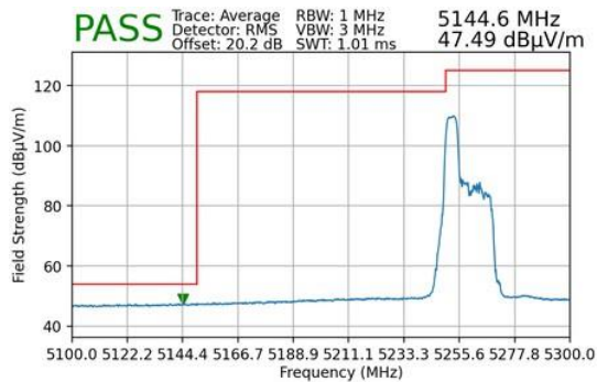
Plot 7-19. Lower Band Edge Plot MIMO (Average – UNII Band 2A)
