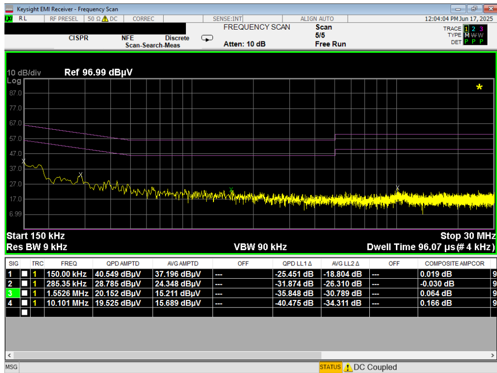
Plot 7-47. Line Conducted Plot with 802.11a UNII Band 4 – Ch.173 (N)
