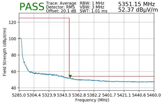
Plot 7-28. Upper Band Edge Plot MIMO (Average – UNII Band 2A)
