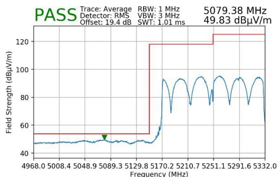
Plot 7-36. Lower Band Edge Plot MIMO (Average – UNII Band 1)
