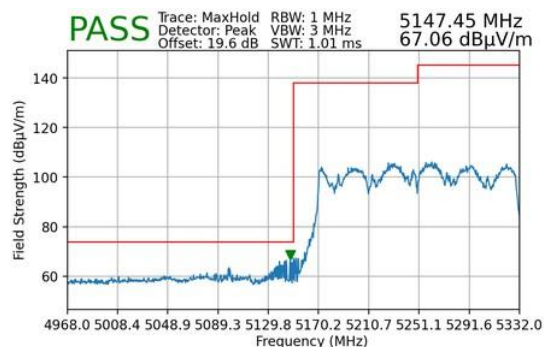
Plot 7-37. Lower Band Edge Plot MIMO (Peak – UNII Band 1)
