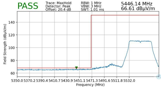
Plot 7-31. Lower Band Edge Plot MIMO (Peak – UNII Band 2C)
