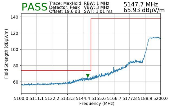
Plot 7-14. Lower Band Edge Plot MIMO (Peak – UNII Band 1)
