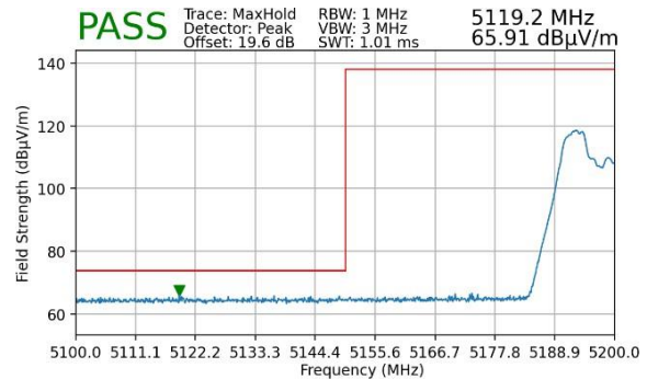
Plot 7-16. Lower Band Edge Plot MIMO (Peak – UNII Band 1)
