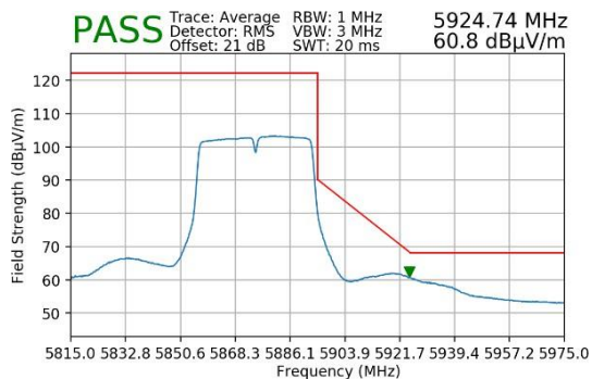
Plot 7-33. Upper Band Edge Plot MIMO (Average – UNII Band 4)
