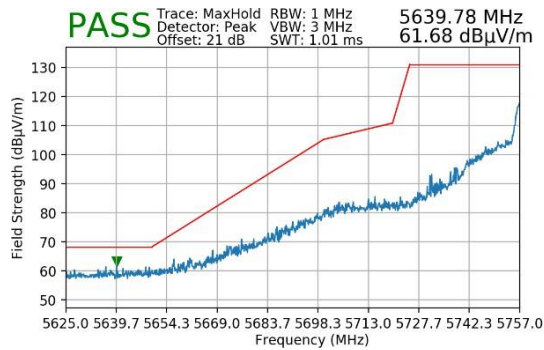
Plot 7-23. Low Band Edge Plot MIMO (Peak – UNII Band 3)
