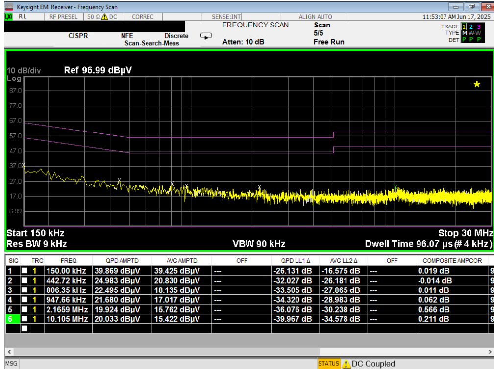
Plot 7-40. Line Conducted Plot with 802.11a UNII Band 2A – Ch.56 (L1)
