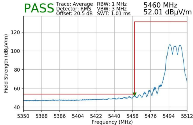
Plot 7-21. Lower Band Edge Plot MIMO (Average – UNII Band 2C)
