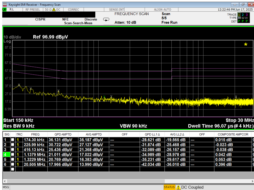
Plot 7-38. Line Conducted Plot with 802.11a UNII Band 1 – Ch.40 (L1)
