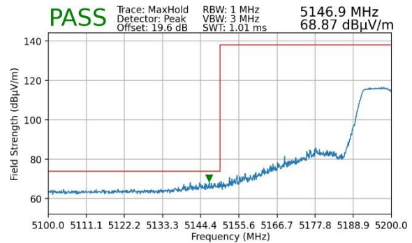
Plot 7-18. Lower Band Edge Plot MIMO (Peak – UNII Band 1)
