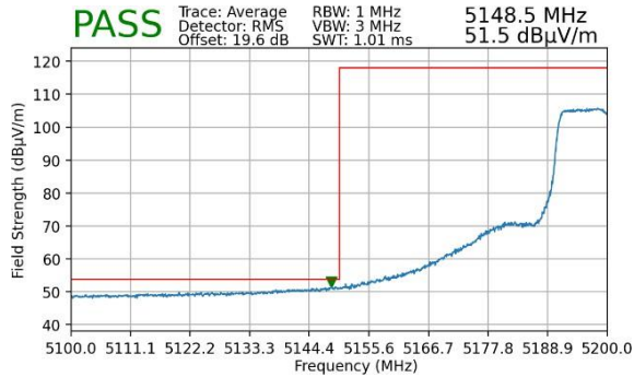
Plot 7-13. Lower Band Edge Plot MIMO (Average – UNII Band 1)
