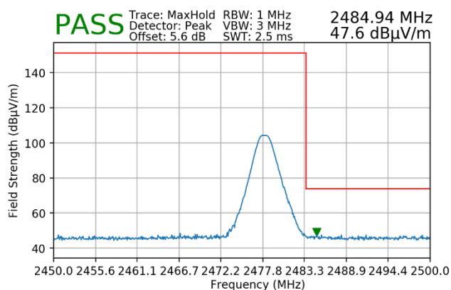
Plot 7-2. Radiated Restricted Upper Band Edge Measurement (Peak) – DUAL
