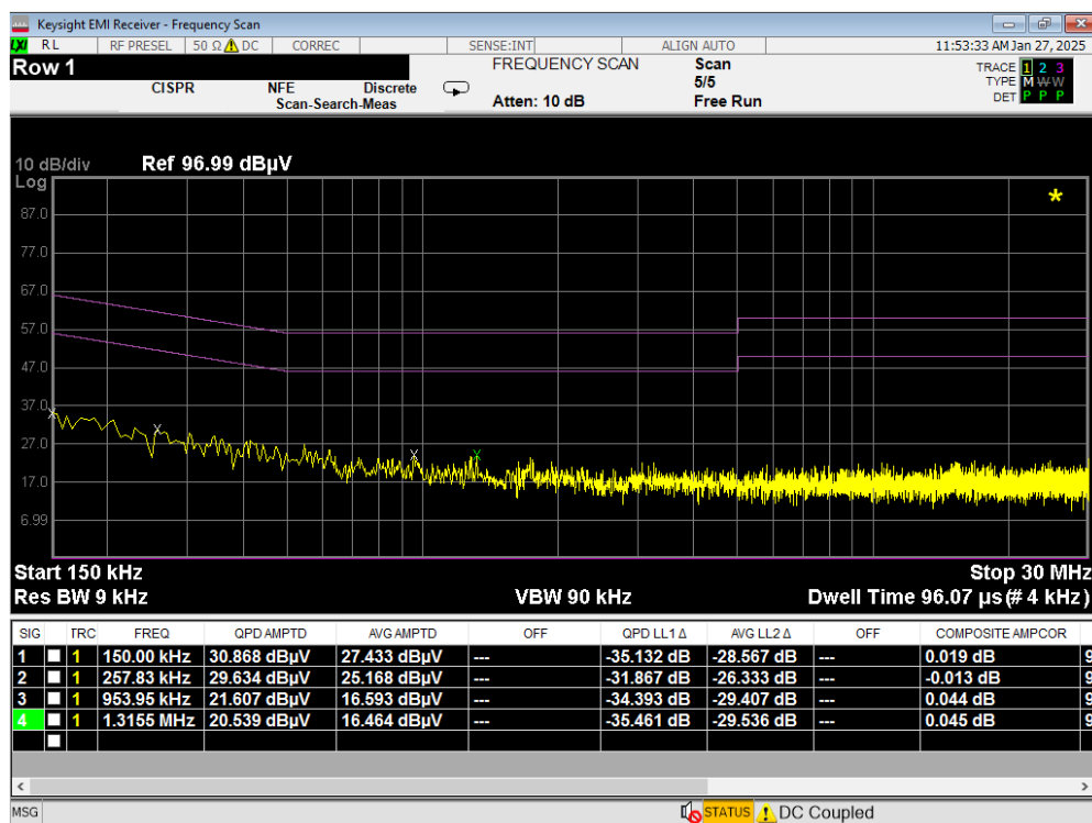
Plot 7-4. Line Conducted Plot with Bluetooth LE (N)
