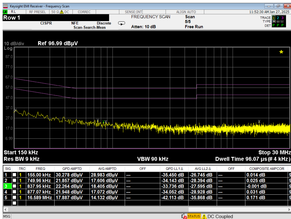
Plot 7-3. Line Conducted Plot with Bluetooth LE (L1)
