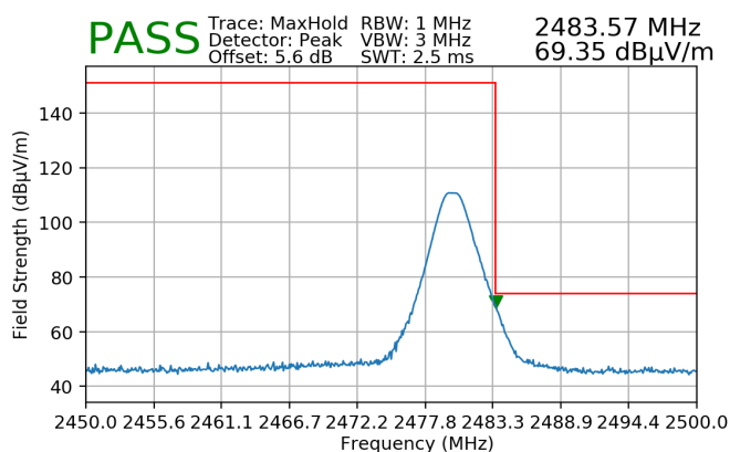
Plot 7-2. Radiated Restricted Upper Band Edge Measurement (Peak) – DUAL
