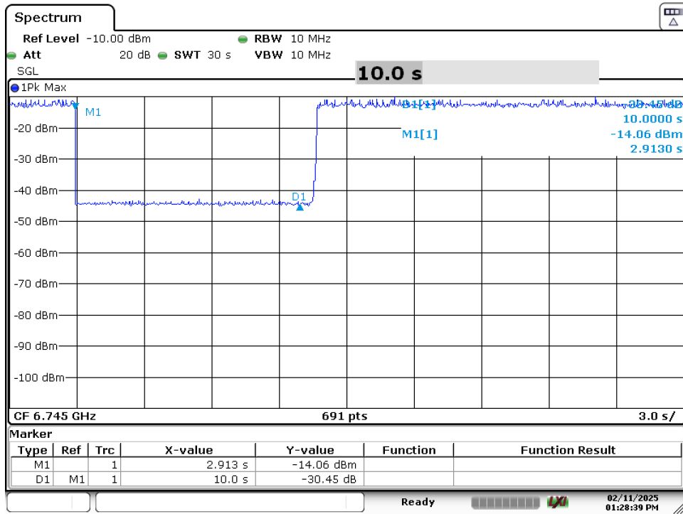
Plot 7-12. Contention Based Protocol Timing Plot (320MHz (UNII Band 7) – Ch. 159 Mid) - Ceased
