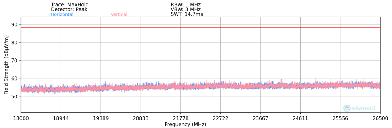
Plot 7-4. Radiated Spurious Plot 18GHz - 26.5GHz (802.11be (20MHz 52T)) Ch.49
