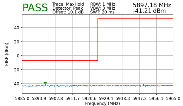
Plot 7-9. Lower Band Edge Plot MIMO (Peak – UNII Band 5)
