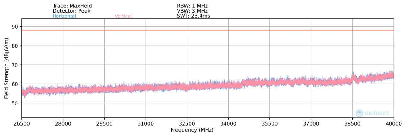
Plot 7-5. Radiated Spurious Plot 26.5GHz - 40GHz (802.11be(20MHz 52T)) Ch.49
