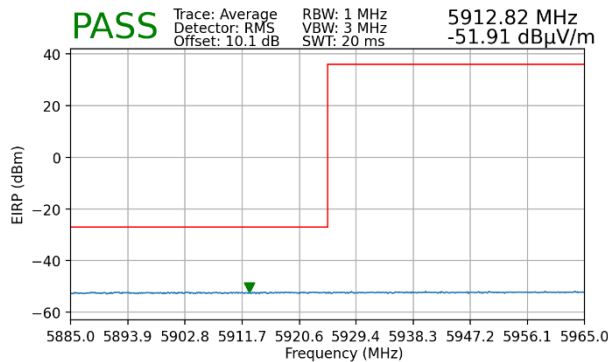
Plot 7-8. Lower Band Edge Plot MIMO (Average – UNII Band 5)
