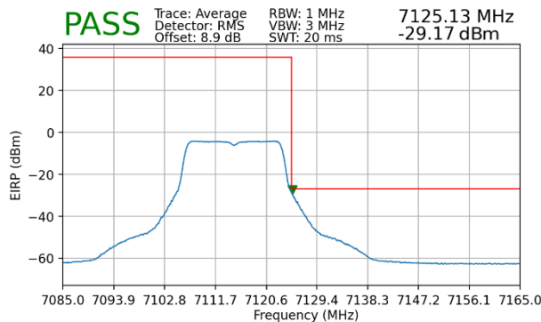
Plot 7-10. Upper Band Edge Plot MIMO (Average – UNII Band 8)
