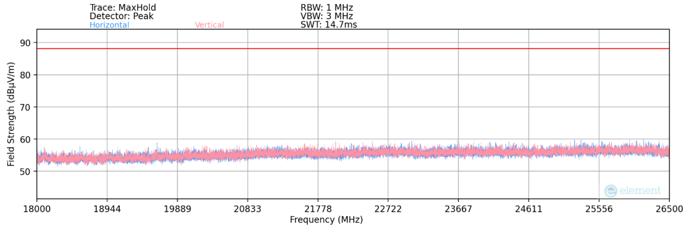
Plot 7-4. Radiated Spurious Plot 18GHz - 26.5GHz (802.11be (20MHz 52T) Ch.40)
