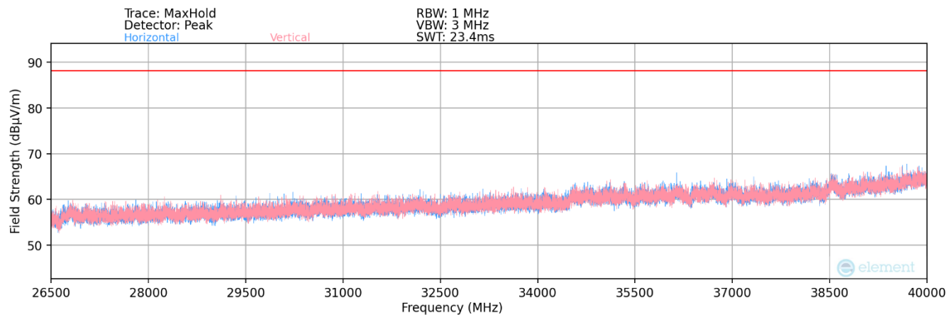
Plot 7-7. Radiated Spurious Plot 26.5GHz - 40GHz (802.11be(320MHz) Ch.31)
