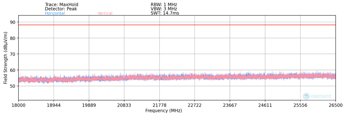
Plot 7-6. Radiated Spurious Plot 18GHz - 26.5GHz (802.11be (320MHz) Ch.31)
