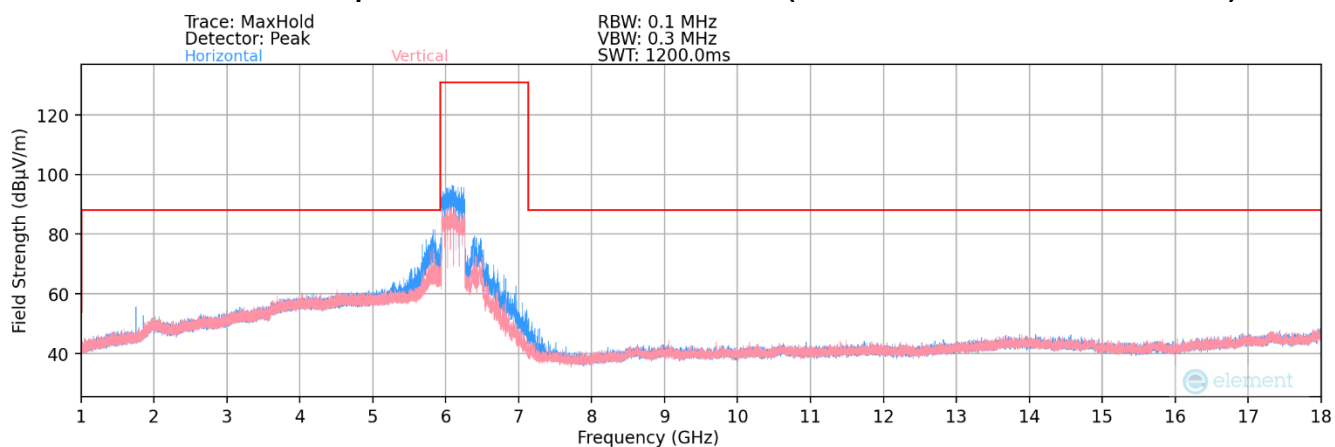
Plot 7-3. Radiated Spurious Plot 1GHz – 18GHz MIMO (802.11be – UNII Band 5 Ch. 31)
