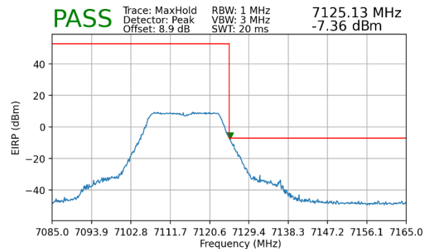
Plot 7-11. Upper Band Edge Plot MIMO (Peak – UNII Band 8)
