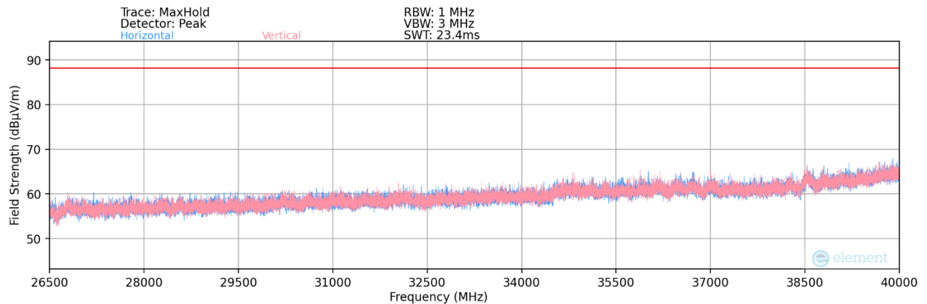
Plot 7-5. Radiated Spurious Plot 26.5GHz - 40GHz (802.11be(20MHz 52T) Ch.40)
