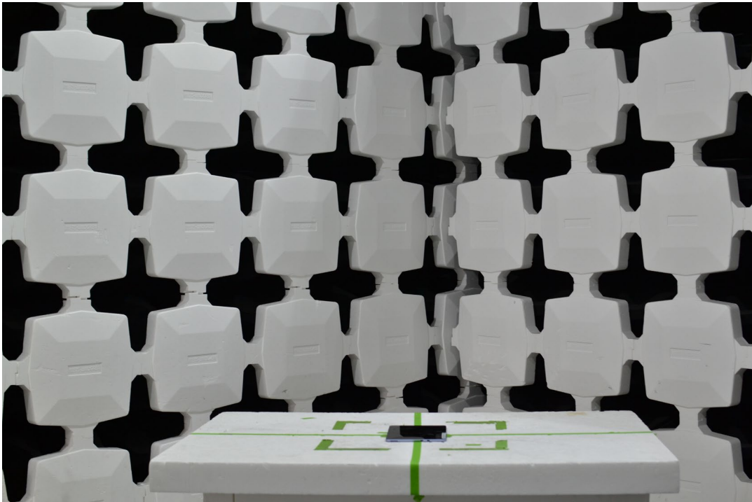
Figure 1. Test Setup – X Position – 30MHz-1GHz – NFC
