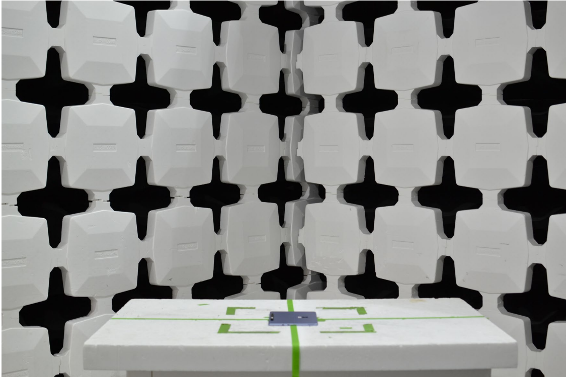
Figure 7. Test Setup – X Position – 30MHz-1GHz – Pen Charging
