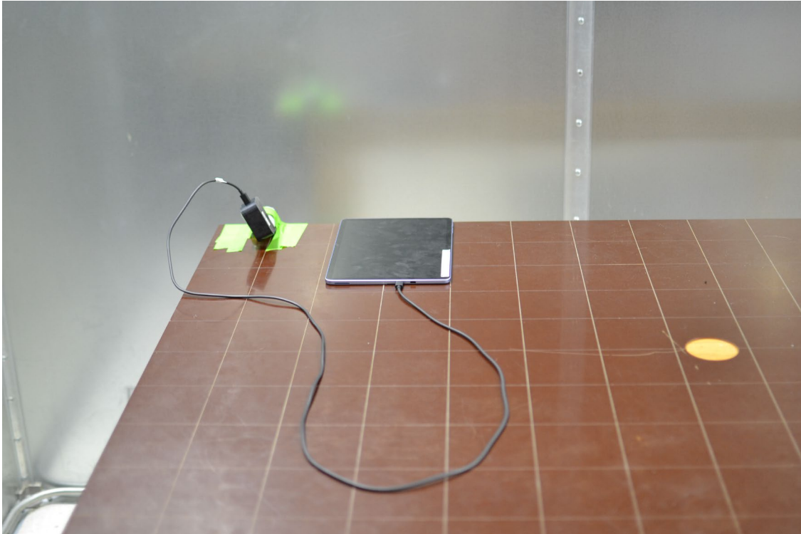
Figure 11. Test Setup – ACLC – <30MHz – NFC
