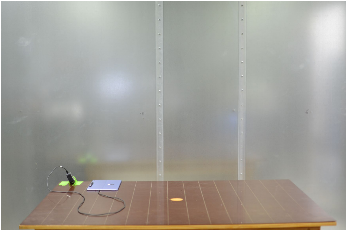
Figure 12. Test Setup – ACLC – <30MHz – Pen Charging
