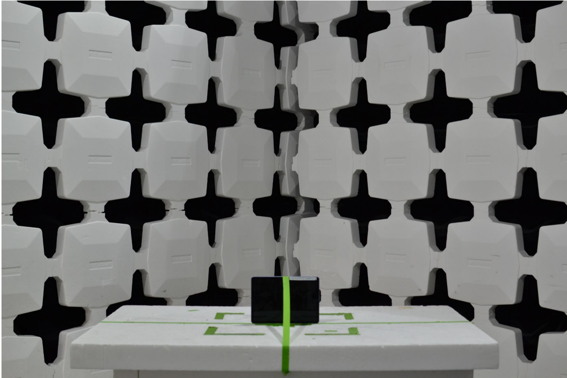
Figure 5. Test Setup – Z Position – 30MHz-1GHz – NFC
