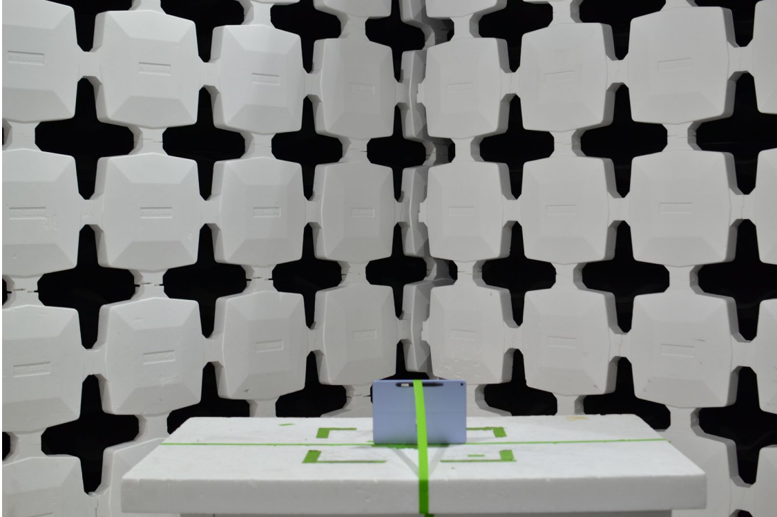
Figure 9. Test Setup – Z Position – 30MHz-1GHz – Pen Charging
