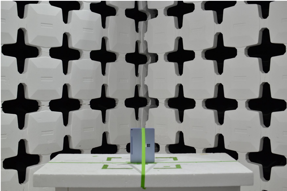
Figure 4. Test Setup – Y Position – 30MHz-1GHz – NFC
