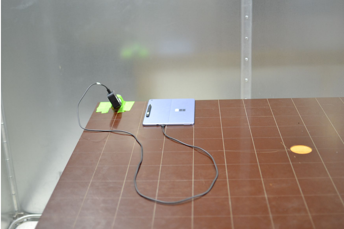
Figure 13. Test Setup – ACLC – <30MHz – Pen Charging
