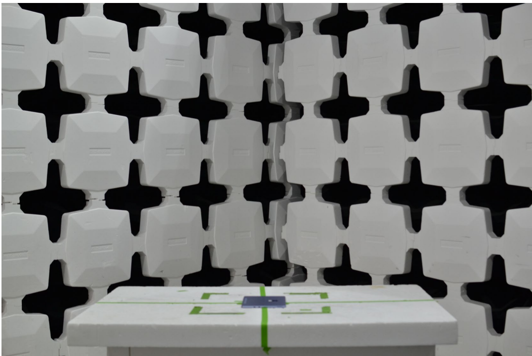
Figure 2. Test Setup – X Position – 30MHz-1GHz - NFC
