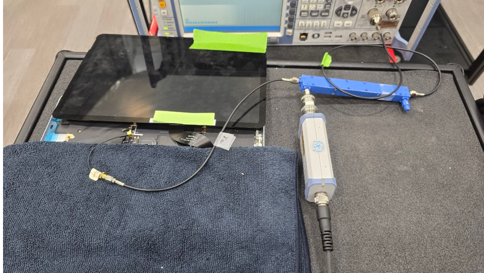
Test Setup Photo 1 – Conducted Test Setup (Figure 6-1a)
