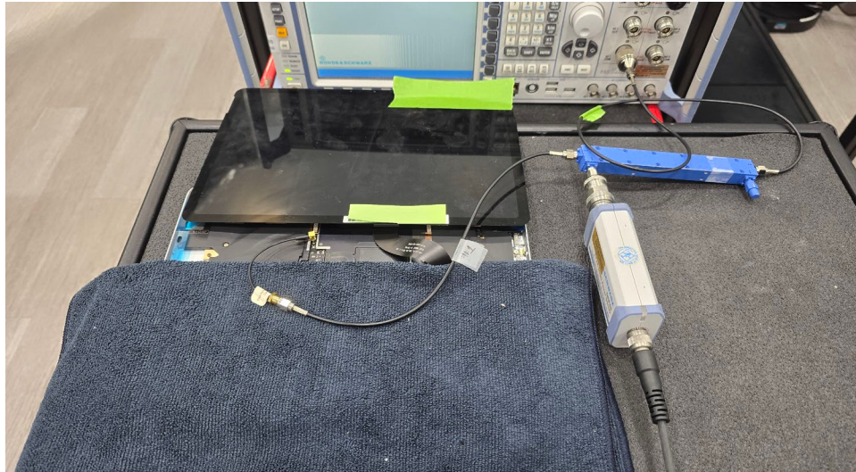
Test Setup Photo 2 – Conducted Test Setup (Figure 6-1a)
