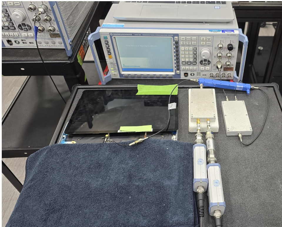
Test Setup Photo 3 – Conducted Test Setup (Figure 6-1b)
