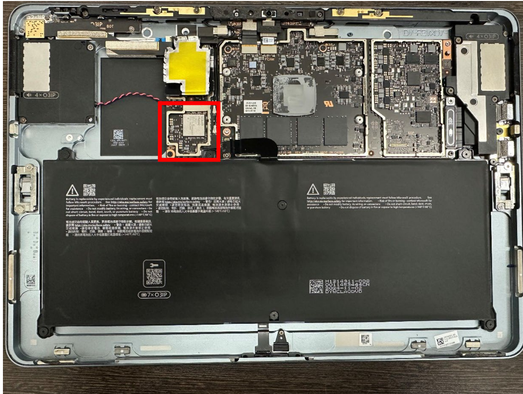
Figure 2: Wifi BT Module
