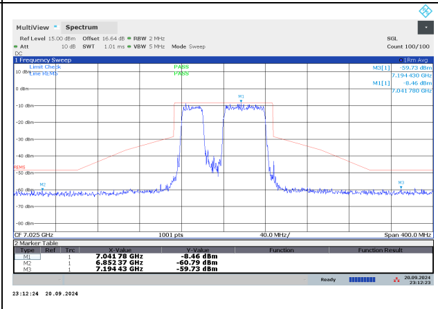
HIGH CHANNEL CHAIN 1
