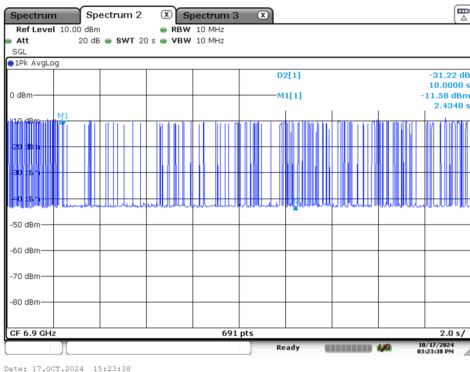
Plot 7-29. Contention Based Protocol Timing Plot (320MHz (UNII Band 7) – Ch. 159 High) - Partial Detection
