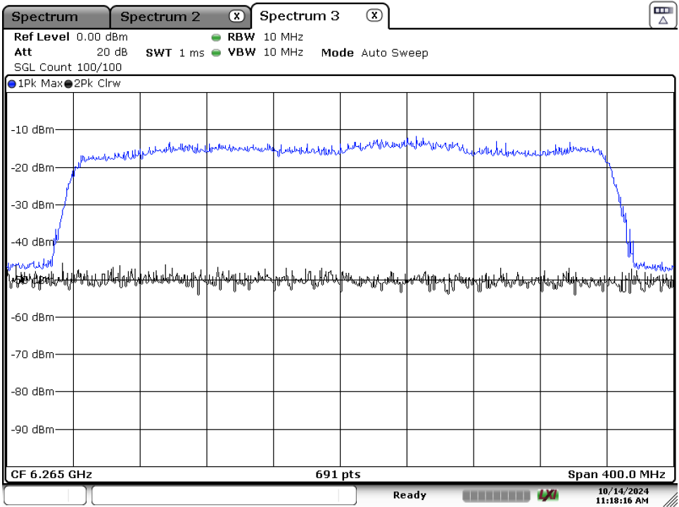
Plot 7-35. CBP 320MHz Ch.31 - Injection Center – [6265 MHz]
