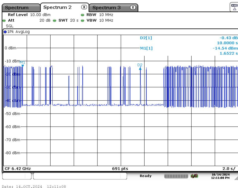
Plot 7-21. Contention Based Protocol Timing Plot (320MHz (UNII Band 5) – Ch. 31 High) - Partial Detection
