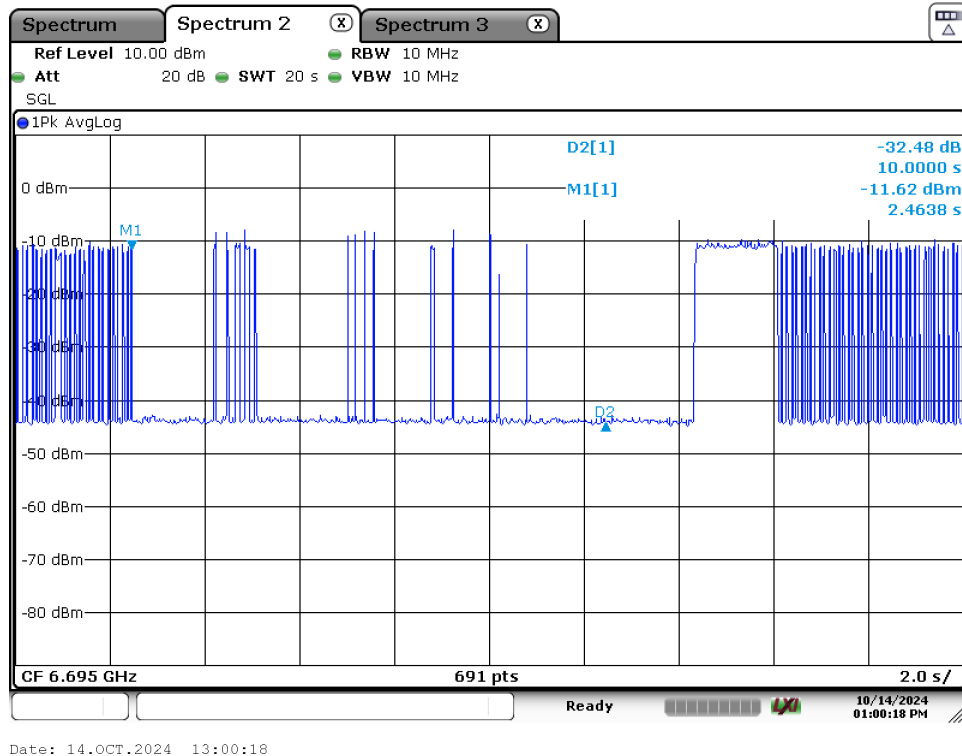
Plot 7-26. Contention Based Protocol Timing Plot (20MHz (UNII Band 7) – Ch. 149) - Partial Detection
