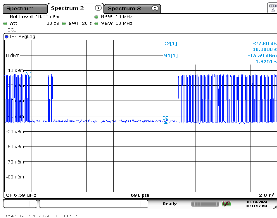
Plot 7-27. Contention Based Protocol Timing Plot (320MHz (UNII Band 7) – Ch. 159 Low) - Partial Detection
