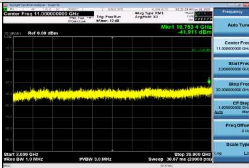
Band2-3MHz-16QAM-18615-1RB#0-Range3:2000~20000MHz
