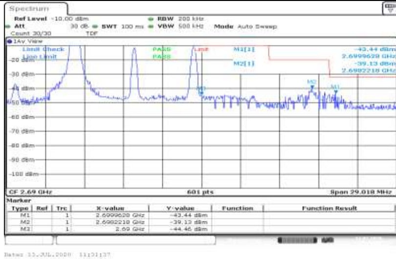
Band41-10MHz-QPSK-41540-50RB#0
