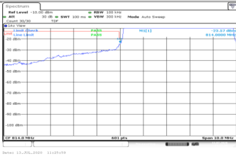
Band26-5MHz-QPSK-26715-25RB#0
