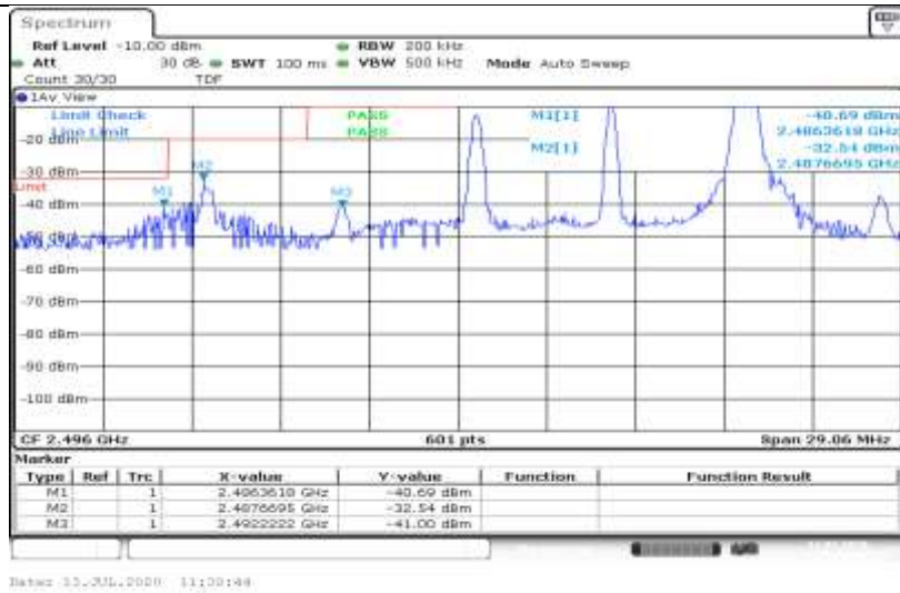
Band41-10MHz-QPSK-39700-1RB#0
