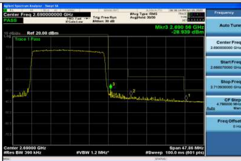
Band41-20MHz-QPSK-41490-100RB#0
