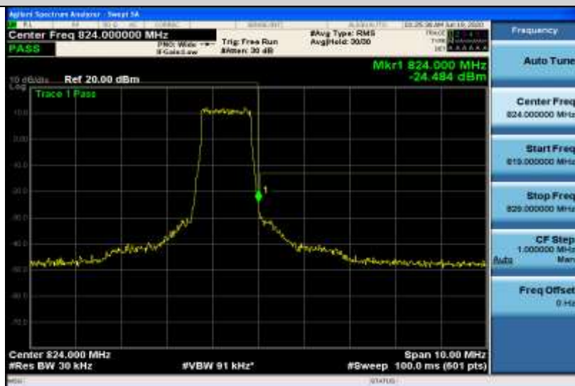
Band26-1.4MHz-QPSK-26783-6RB#0
