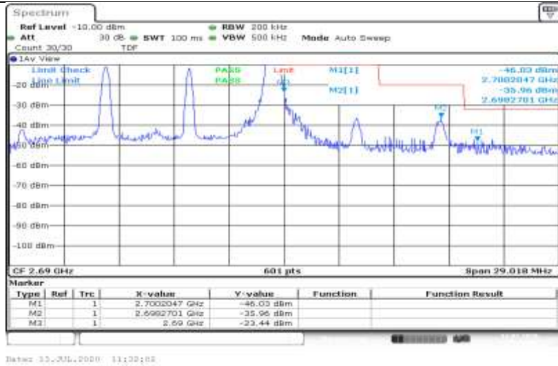
Band41-10MHz-QPSK-41540-1RB#0
