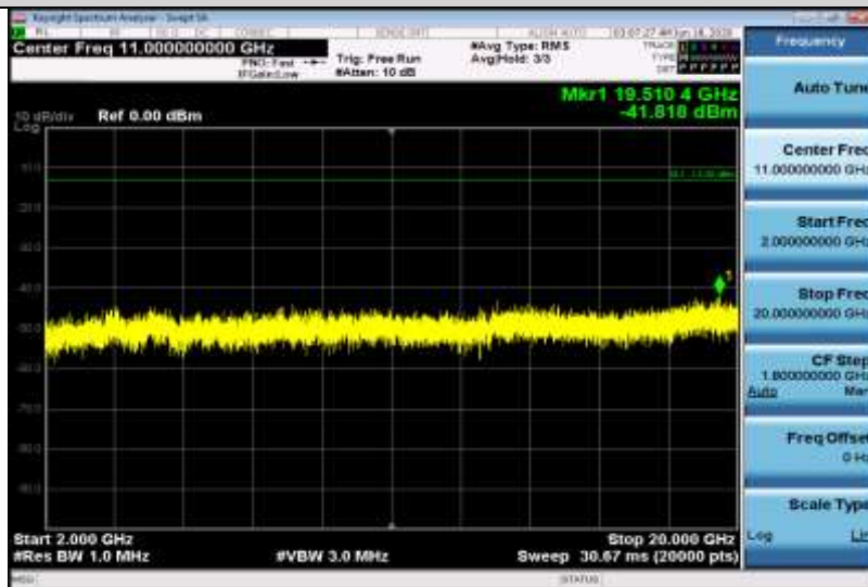
Band2-10MHz-QPSK-18650-1RB#0-Range3:2000~20000MHz
