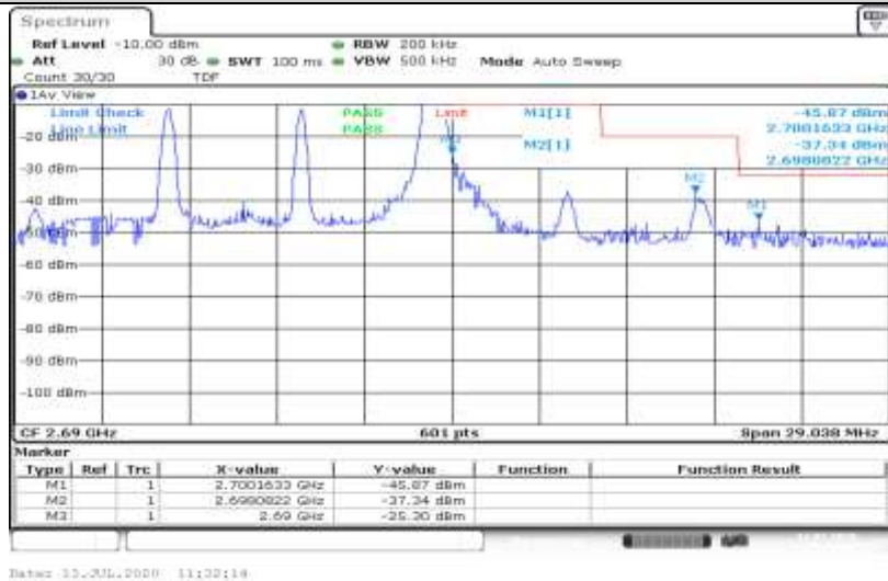
Band41-10MHz-16QAM-41540-50RB#0
