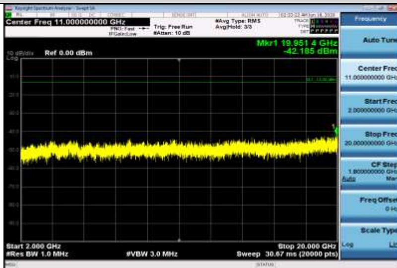
Band2-3MHz-16QAM-19185-1RB#0-Range3:2000~20000MHz
