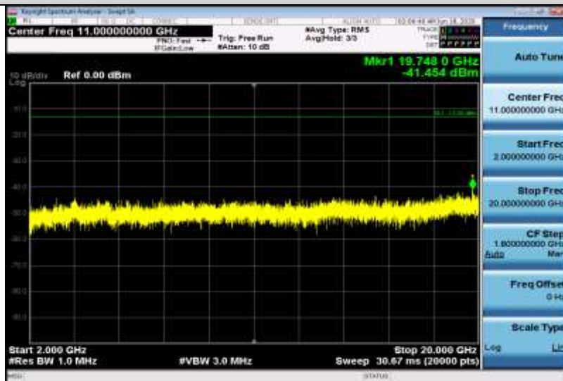
Band2-1.4MHz-16QAM-18607-1RB#0-Range3:2000~20000MHz
