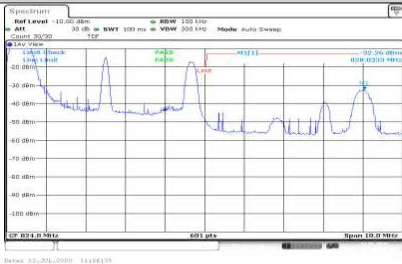
Band26-5MHz-QPSK-26765-25RB#0
