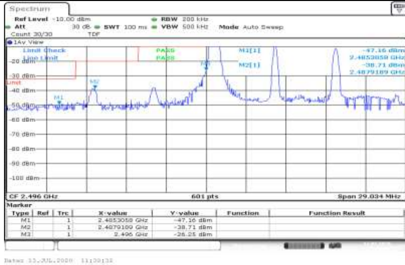
Band41-10MHz-16QAM-39700-50RB#0
