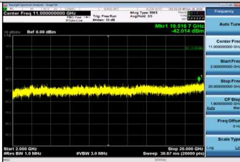
Band2-3MHz-16QAM-18900-1RB#0-Range3:2000~20000MHz
