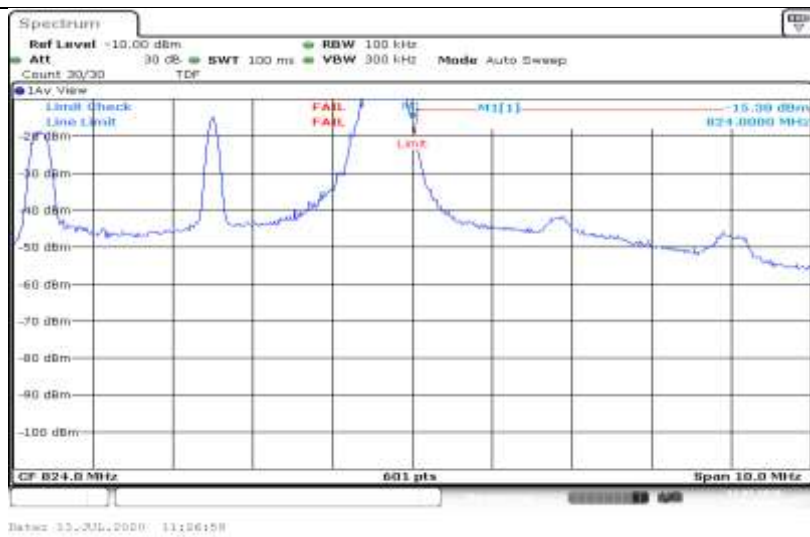
Band26-5MHz-QPSK-26765-1RB#0
