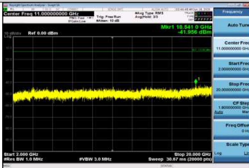
Band2-20MHz-QPSK-19100-1RB#0-Range3:2000~20000MHz
