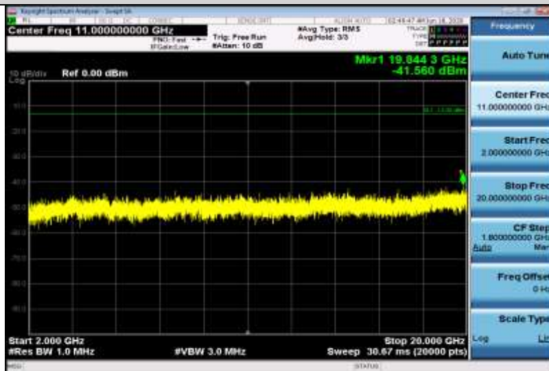
Band2-5MHz-16QAM-18625-1RB#0-Range3:2000~20000MHz
