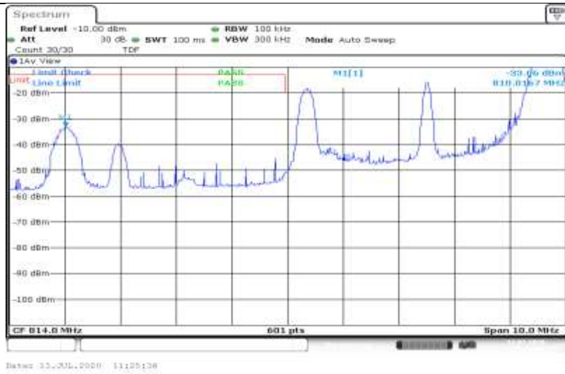
Band26-5MHz-QPSK-26715-1RB#0
