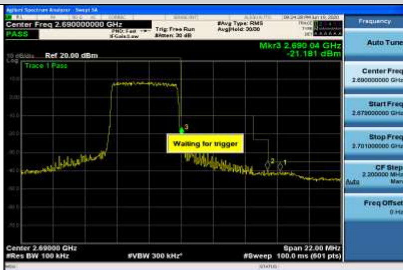
Band41-5MHz-QPSK-41565-25RB#0
