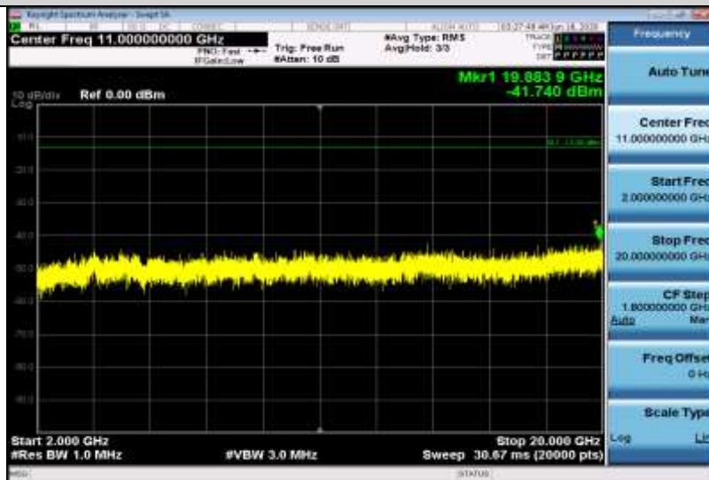
Band2-15MHz-16QAM-19125-1RB#0-Range3:2000~20000MHz
