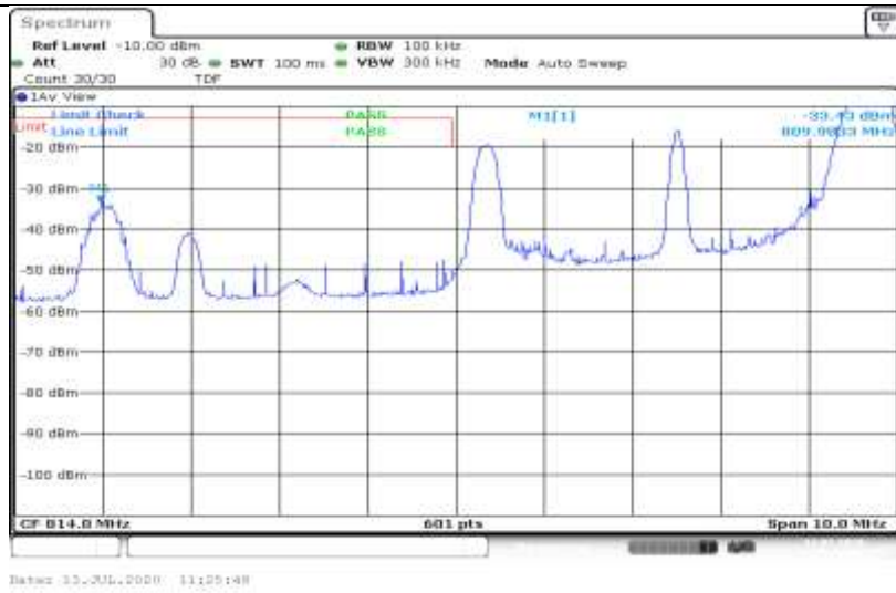
Band26-5MHz-16QAM-26715-1RB#0
