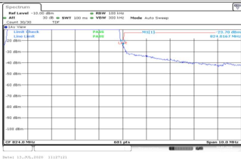
Band26-5MHz-QPSK-26765-25RB#0
