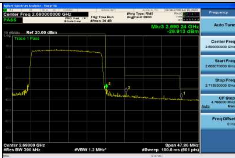
Band41-20MHz-16QAM-41490-100RB#0
