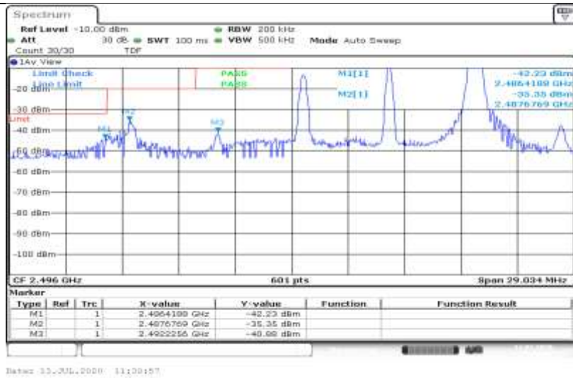
Band41-10MHz-16QAM-39700-1RB#0
