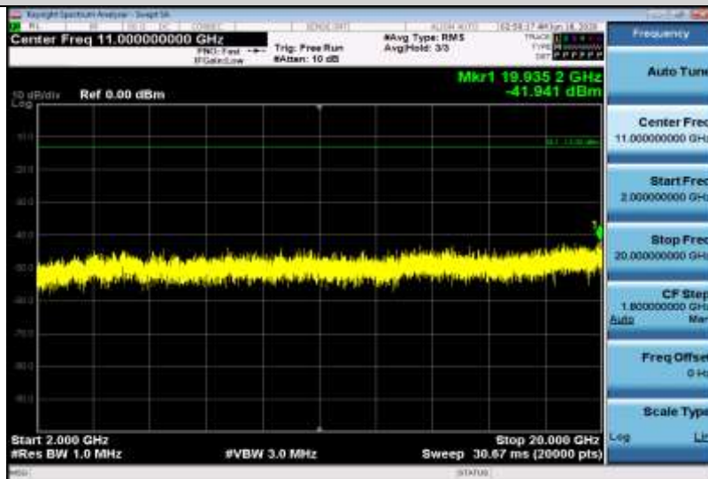
Band2-5MHz-QPSK-18900-1RB#0-Range3:2000~20000MHz
