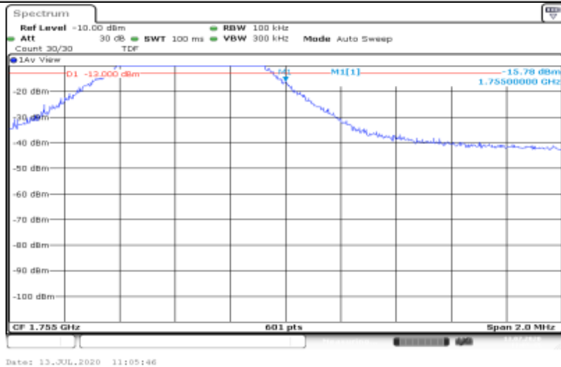
Band4-5MHz-16QAM-20375-25RB#0
