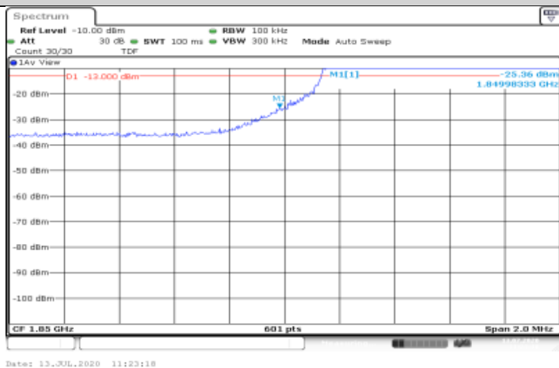
Band25-5MHz-16QAM-26065-25RB#0
