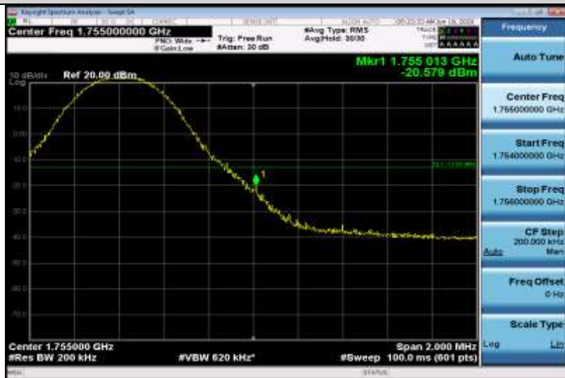
Band4-10MHz-16QAM-20350-50RB#0
