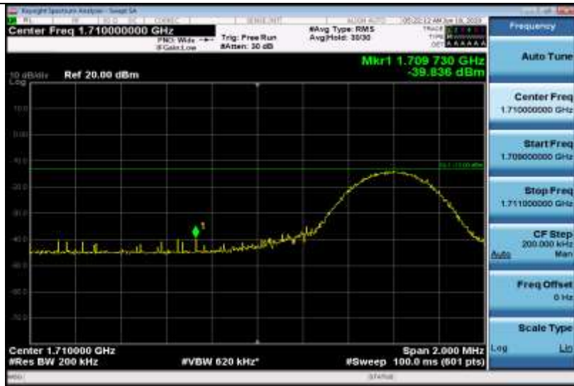
Band4-10MHz-16QAM-20000-1RB#0
