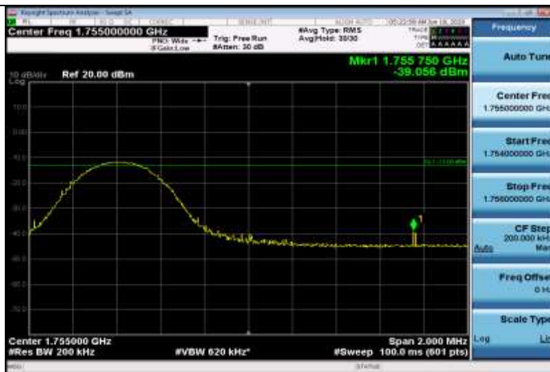
Band4-10MHz-QPSK-20350-1RB#49
