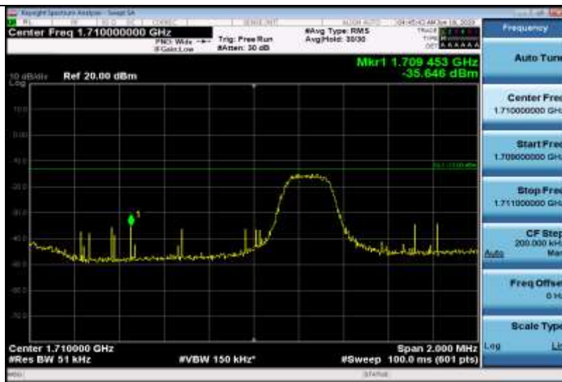
Band4-3MHz-16QAM-19965-1RB#0
