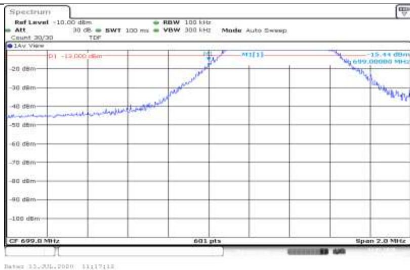
Band12-5MHz-16QAM-23035-1RB#24
