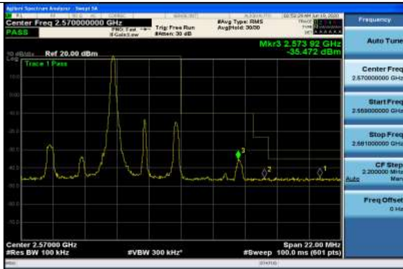
Band7-5MHz-16QAM-21425-1RB#24
