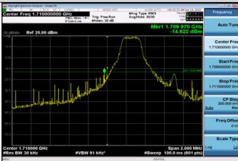
Band4-1.4MHz-QPSK-19957-1RB#0
