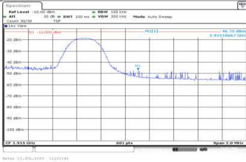
Band25-5MHz-QPSK-26665-1RB#24
