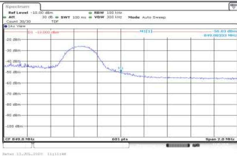
Band5-5MHz-QPSK-20625-25RB#0
