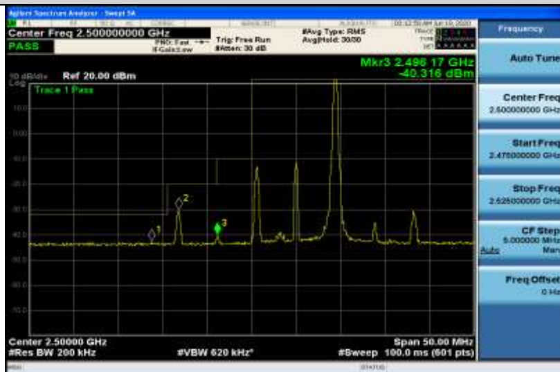
Band7-10MHz-16QAM-20800-50RB#0
