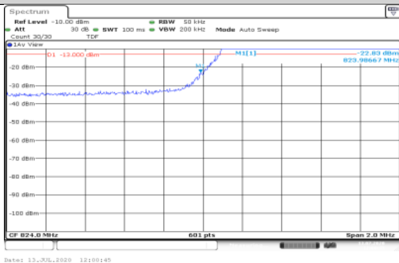
Band5-3MHz-16QAM-20415-15RB#0
