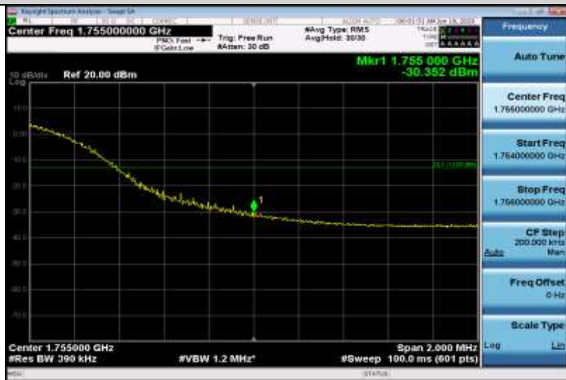
Band4-20MHz-QPSK-20300-100RB#0
