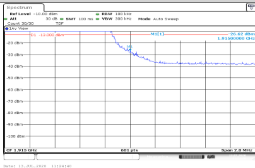
Band25-5MHz-16QAM-26665-25RB#0
