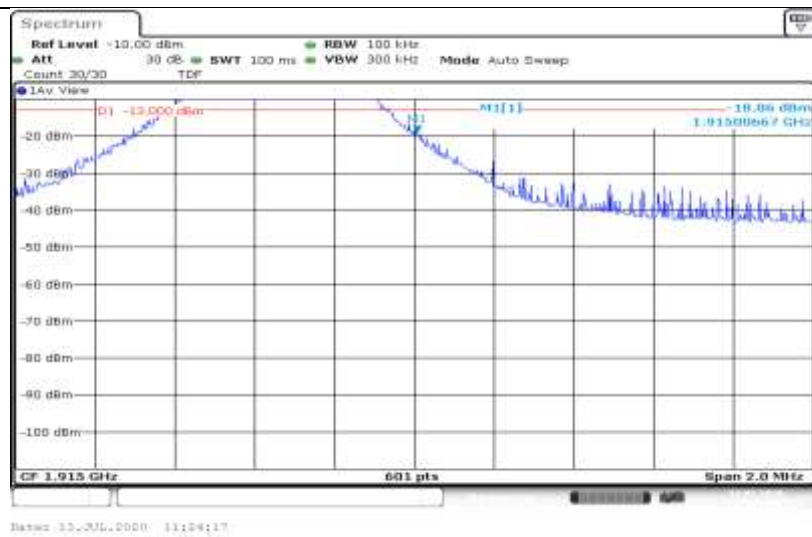
Band25-5MHz-16QAM-26665-1RB#0
