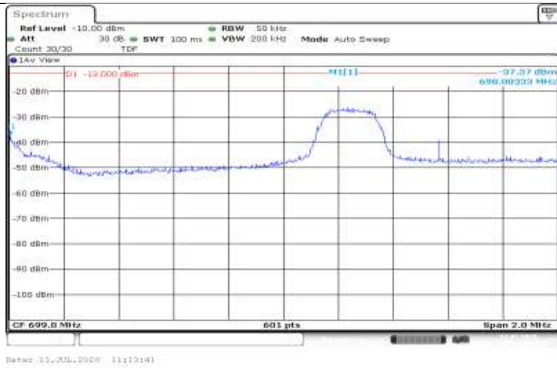
Band12-3MHz-16QAM-23025-1RB#0
