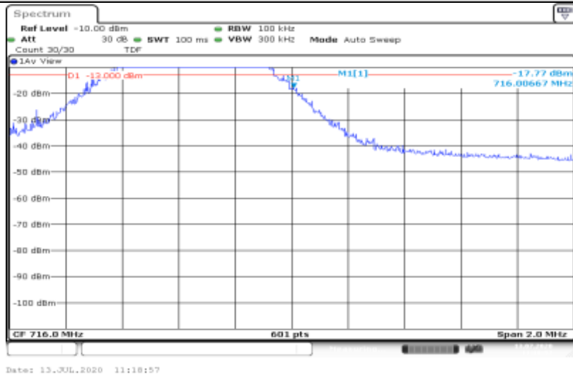
Band12-5MHz-16QAM-23155-25RB#0
