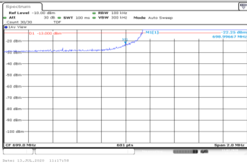
Band12-5MHz-16QAM-23035-25RB#0
