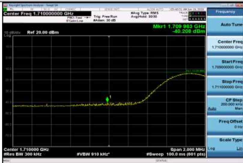
Band4-15MHz-16QAM-20025-75RB#0
