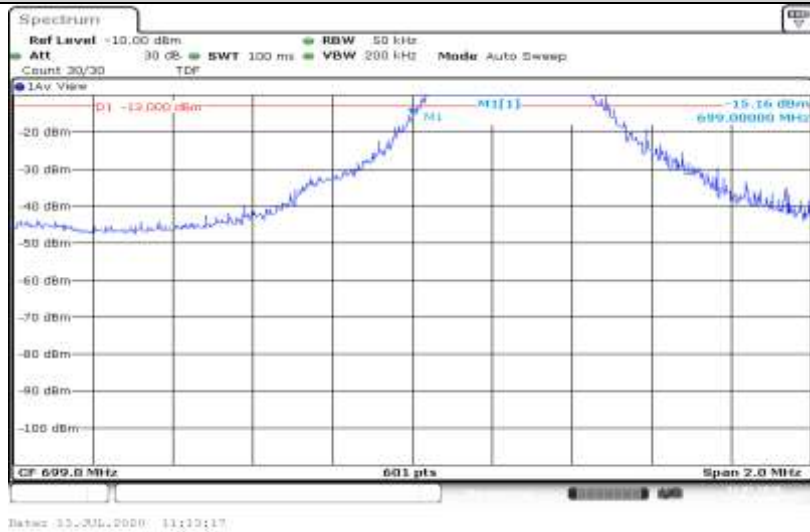
Band12-3MHz-16QAM-23025-15RB#0
