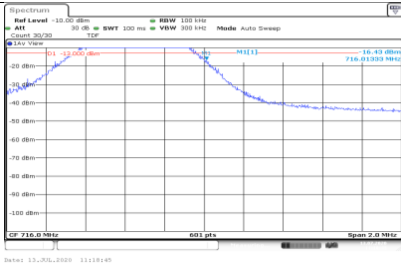
Band12-5MHz-QPSK-23155-1RB#0
