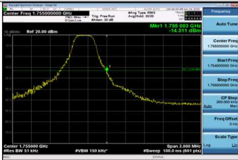
Band4-3MHz-QPSK-20385-15RB#0
