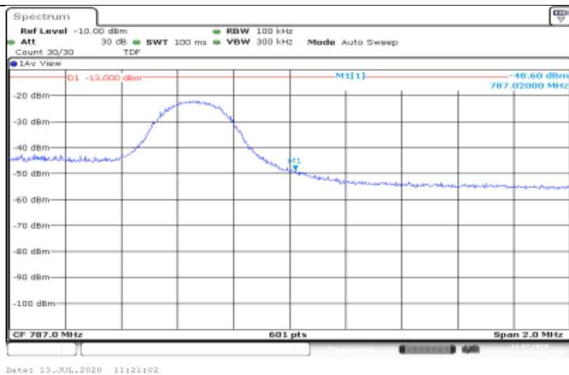
Band13-5MHz-QPSK-23255-1RB#24
