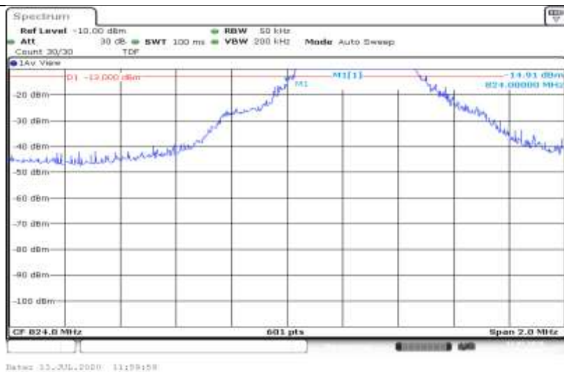
Band5-3MHz-16QAM-20415-1RB#14
