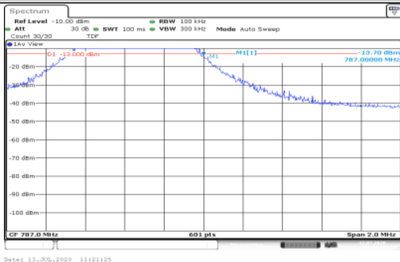
Band13-5MHz-QPSK-23255-25RB#0
