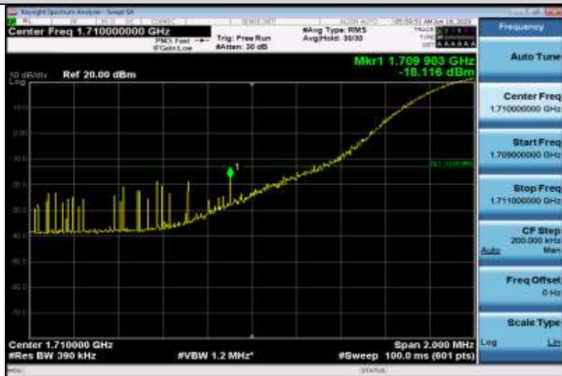
Band4-20MHz-16QAM-20050-100RB#0
