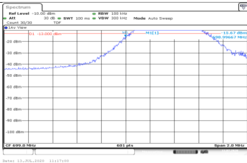
Band12-5MHz-QPSK-23035-1RB#24
