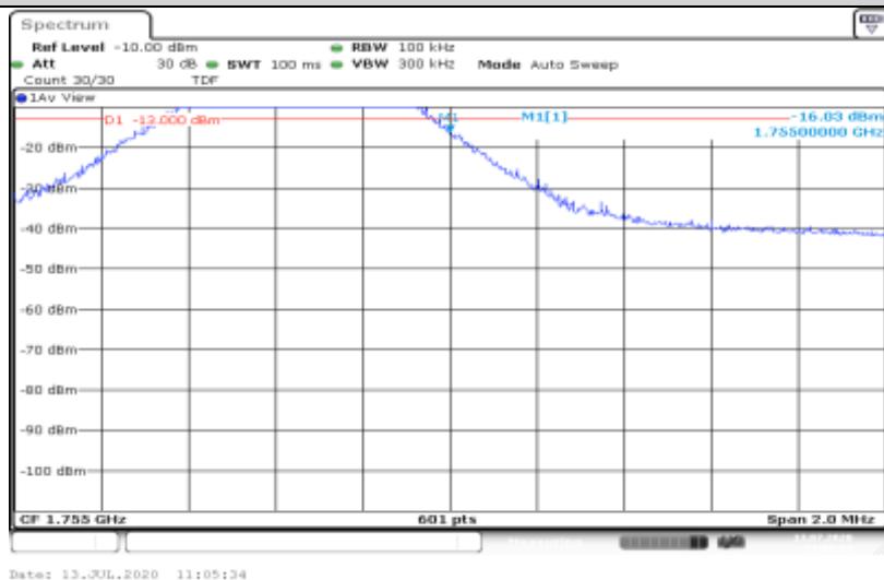
Band4-5MHz-QPSK-20375-25RB#0
