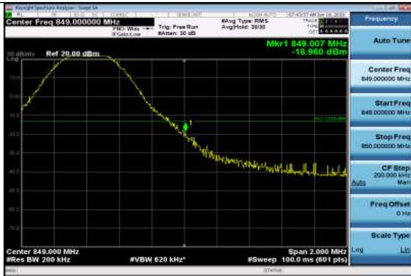
Band5-10MHz-QPSK-20600-1RB#0
