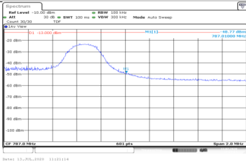
Band13-5MHz-16QAM-23255-25RB#0
