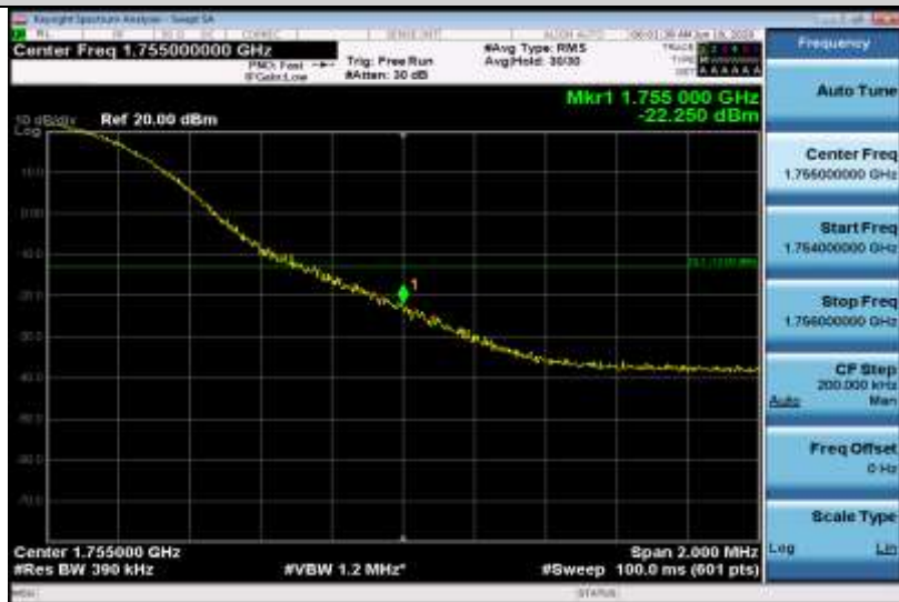
Band4-20MHz-16QAM-20300-100RB#0
