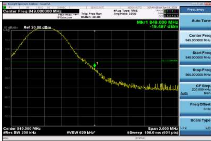
Band5-10MHz-16QAM-20600-1RB#0
