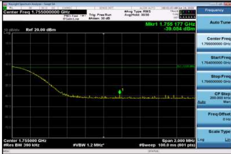
Band4-20MHz-QPSK-20300-100RB#0
