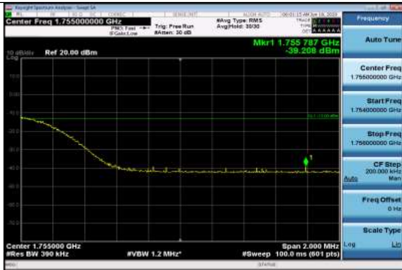
Band4-20MHz-16QAM-20300-1RB#99
