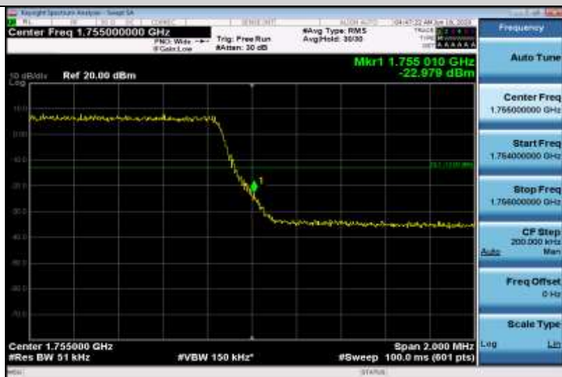
Band4-3MHz-16QAM-20385-15RB#0
