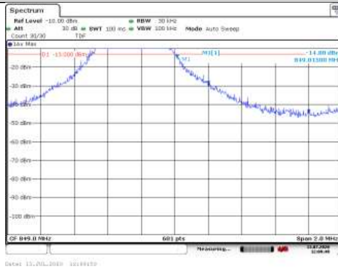
Band5-3MHz-16QAM-20635-15RB#0
