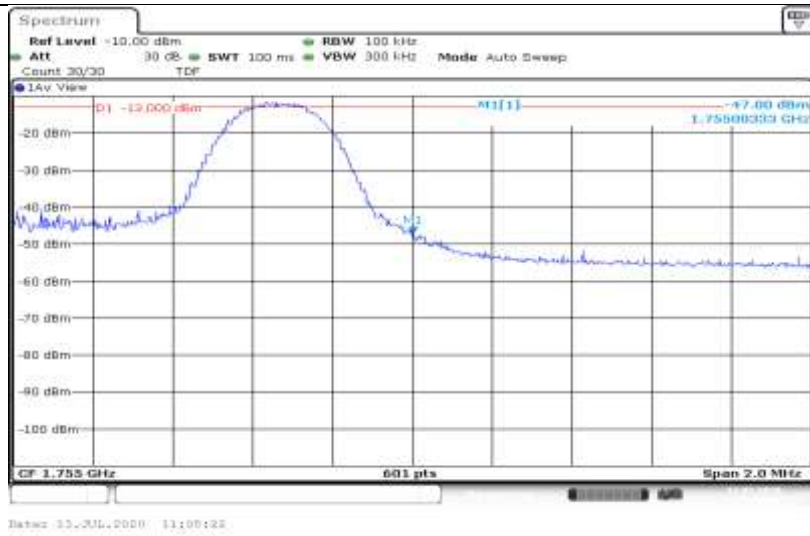
Band4-5MHz-16QAM-20375-1RB#24
