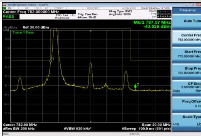
Band13-10MHz-QPSK-23230-50RB#0
