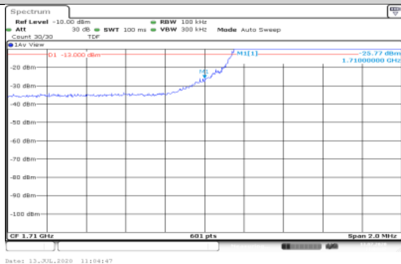
Band4-5MHz-16QAM-19975-25RB#0
