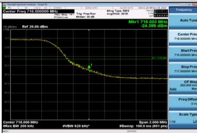
Band12-10MHz-QPSK-23130-50RB#0
