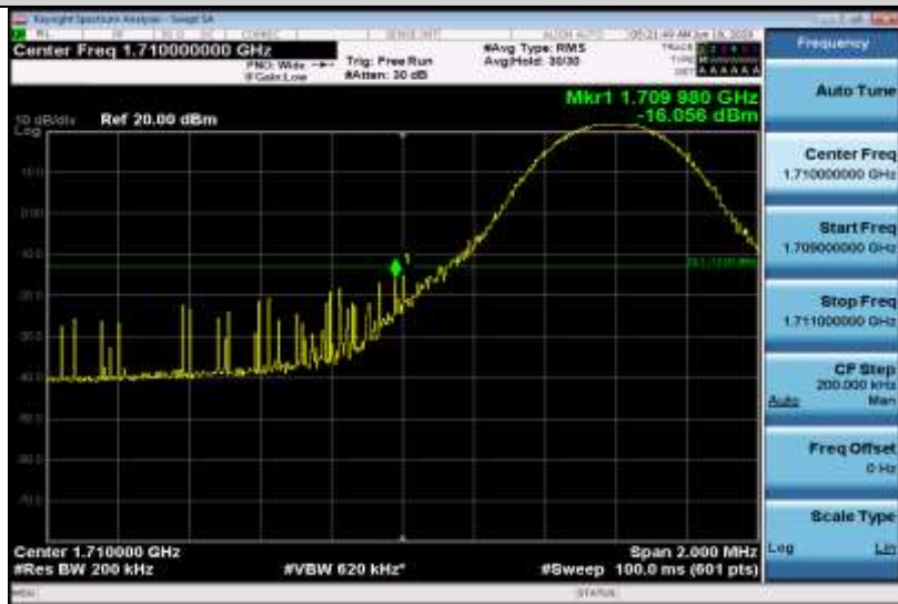
Band4-10MHz-16QAM-20000-50RB#0
