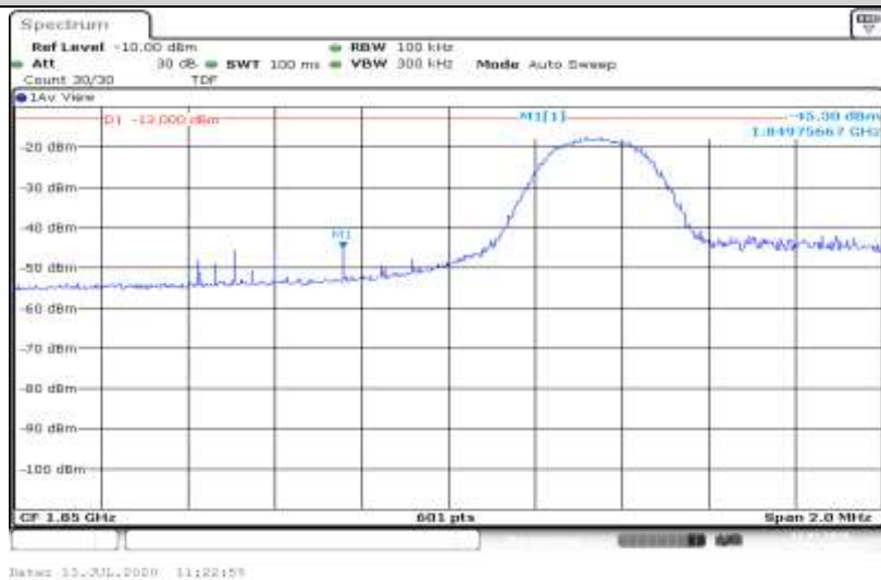
Band25-5MHz-16QAM-26065-25RB#0
