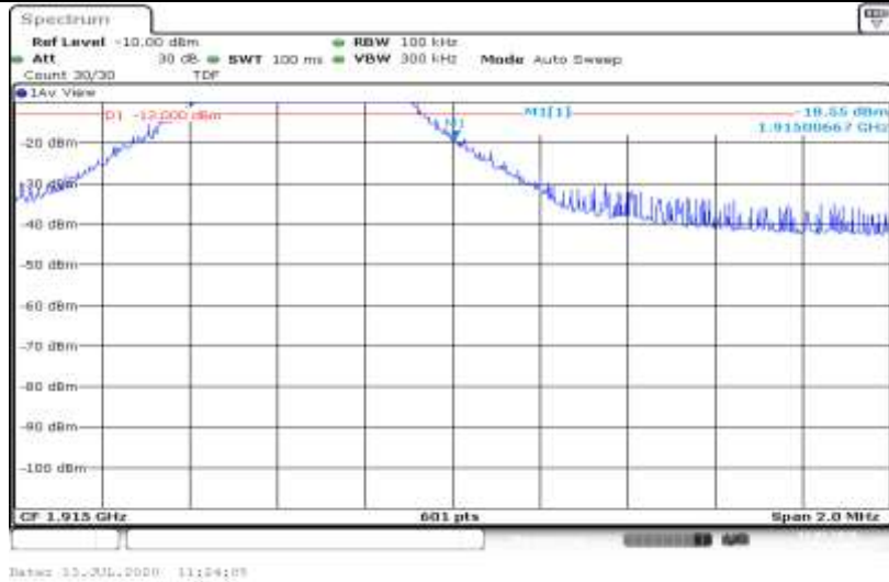
Band25-5MHz-QPSK-26665-25RB#0
