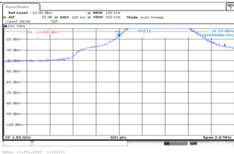
Band25-5MHz-16QAM-26065-1RB#24
