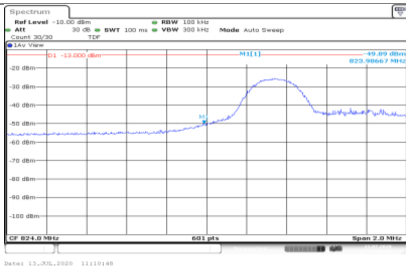
Band5-5MHz-QPSK-20425-1RB#0
