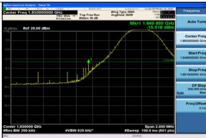
Band25-10MHz-16QAM-26090-1RB#49
