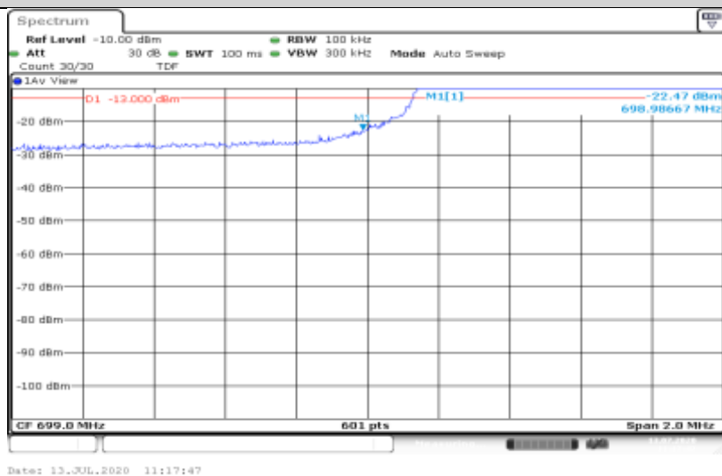
Band12-5MHz-QPSK-23035-25RB#0
