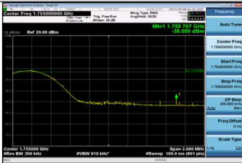
Band4-15MHz-16QAM-20325-75RB#0
