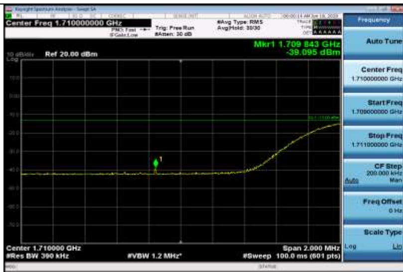
Band4-20MHz-16QAM-20050-1RB#0
