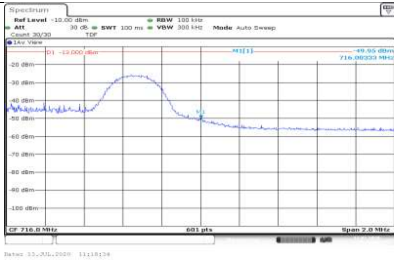
Band12-5MHz-16QAM-23155-1RB#24
