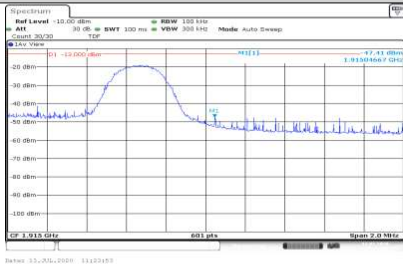
Band25-5MHz-16QAM-26665-25RB#0
