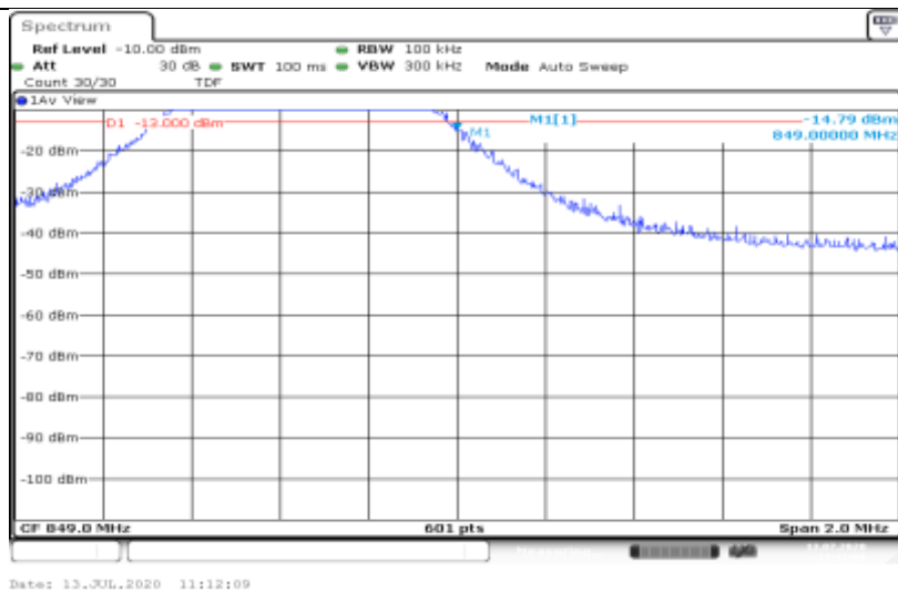
Band5-5MHz-QPSK-20625-1RB#0
