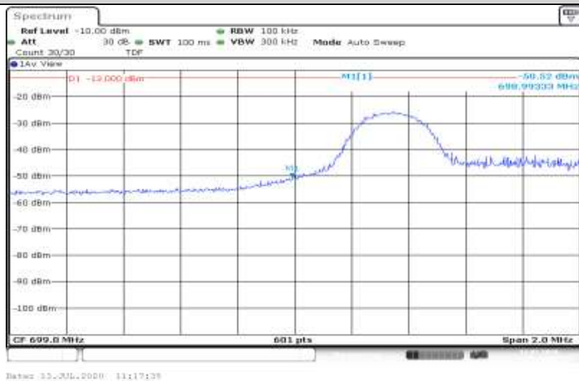
Band12-5MHz-16QAM-23035-25RB#0
