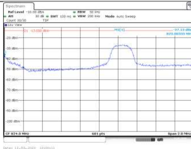
Band5-3MHz-QPSK-20415-15RB#0
