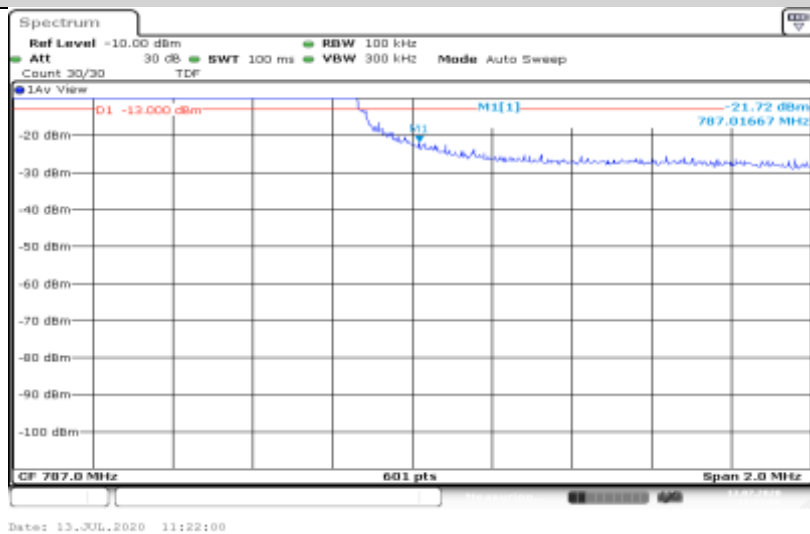
Band13-10MHz-QPSK-23230-1RB#49
