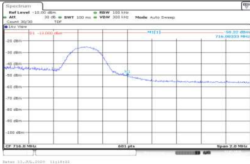
Band12-5MHz-QPSK-23155-25RB#0
