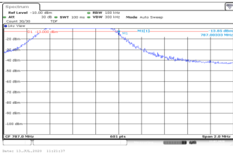
Band13-5MHz-16QAM-23255-1RB#0
