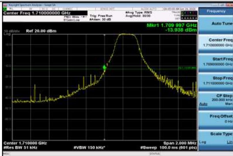
Band4-3MHz-QPSK-19965-15RB#0
