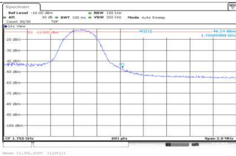
Band4-5MHz-QPSK-20375-1RB#24
