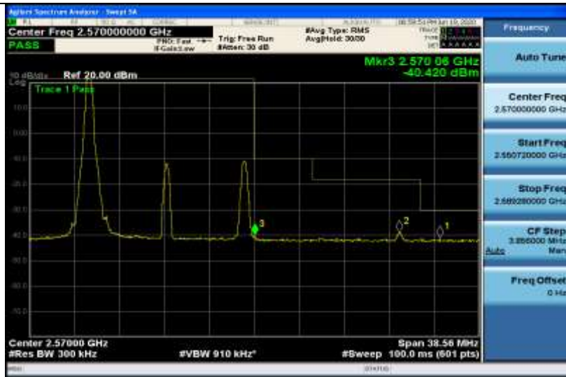
Band7-15MHz-QPSK-21375-1RB#74
