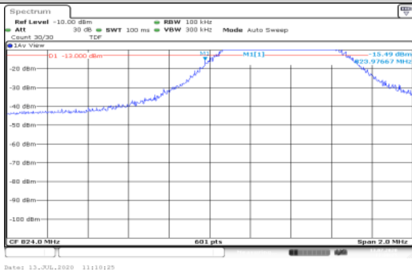
Band5-5MHz-QPSK-20425-1RB#0
