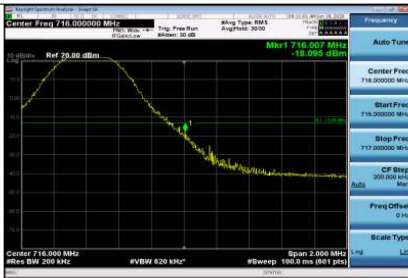
Band12-10MHz-QPSK-23130-1RB#0
