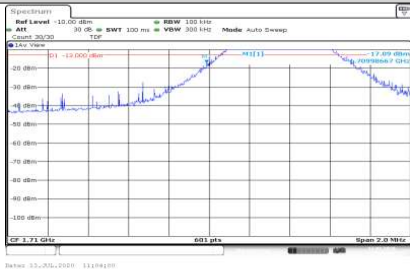
Band4-5MHz-16QAM-19975-25RB#0
