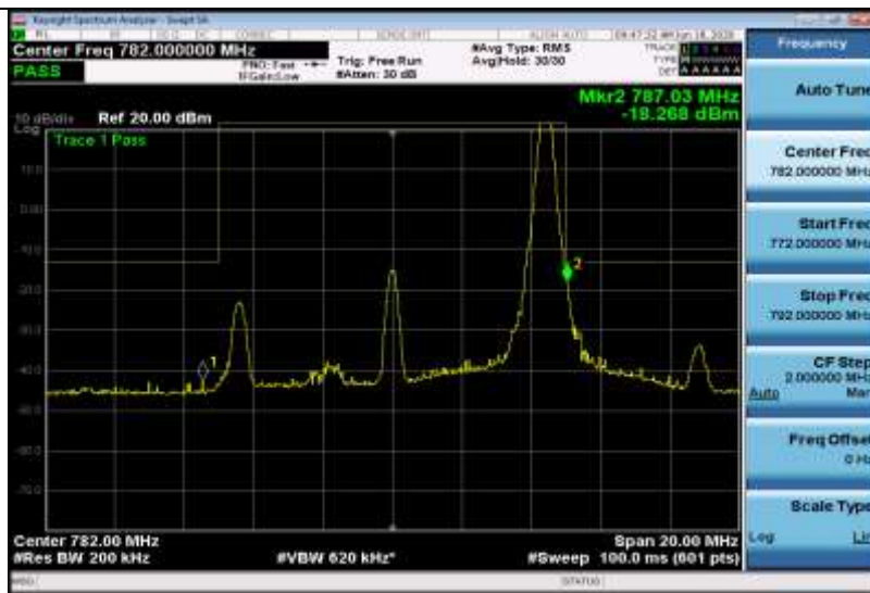
Band13-10MHz-QPSK-23230-1RB#0
