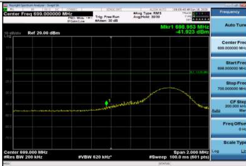
Band12-10MHz-QPSK-23060-50RB#0
