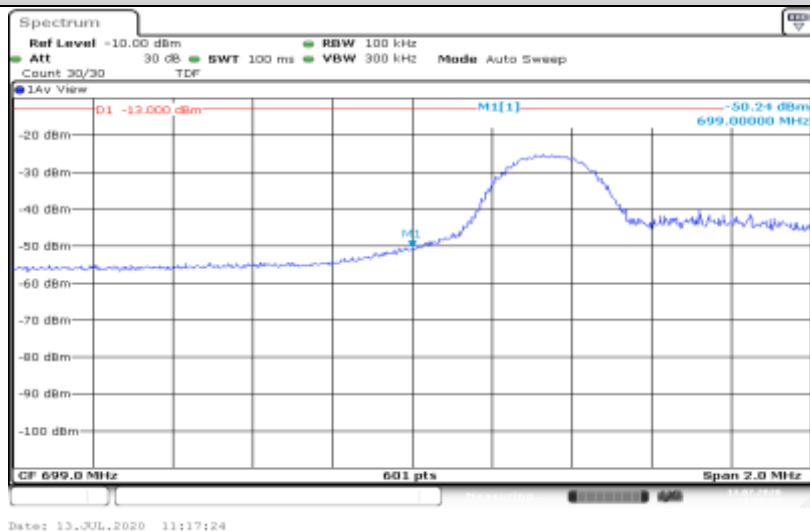
Band12-5MHz-QPSK-23035-25RB#0
