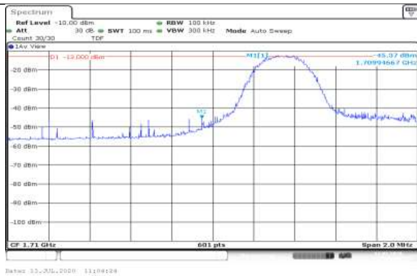
Band4-5MHz-16QAM-19975-1RB#0
