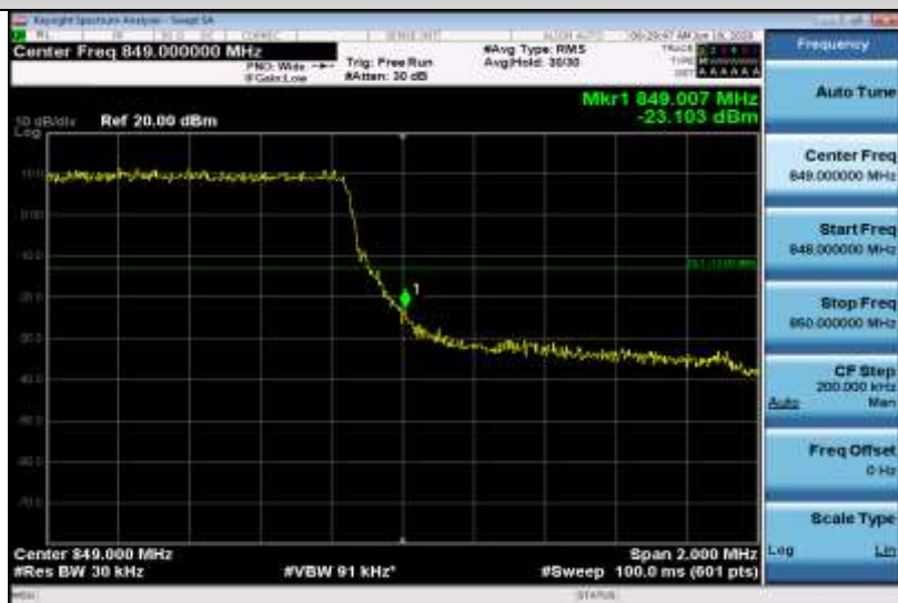
Band5-1.4MHz-16QAM-20643-6RB#0
