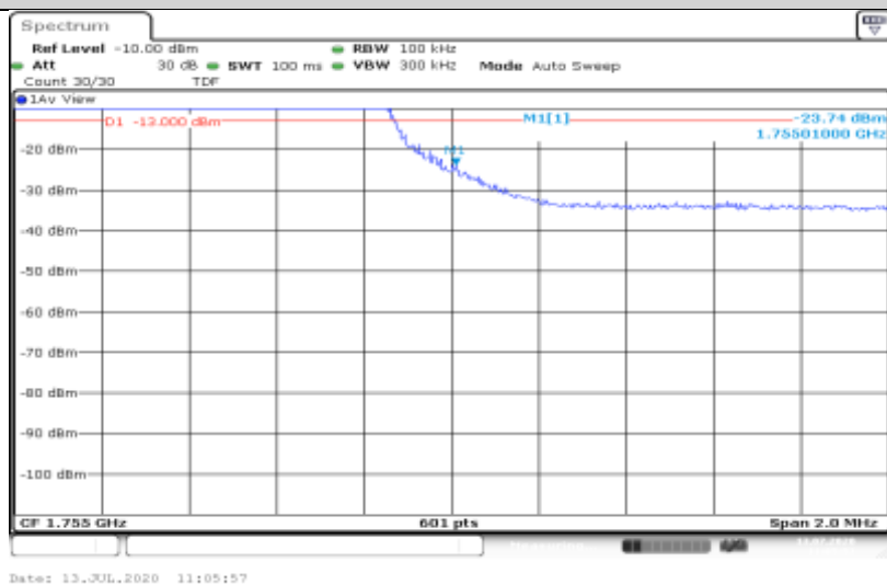
Band4-5MHz-QPSK-20375-25RB#0
