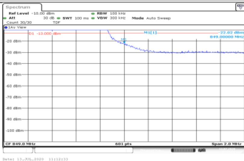
Band5-5MHz-QPSK-20625-25RB#0
