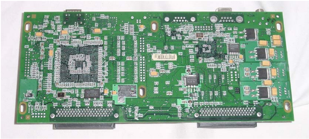
Internal Photo 3 – Digital Board Bottom View
