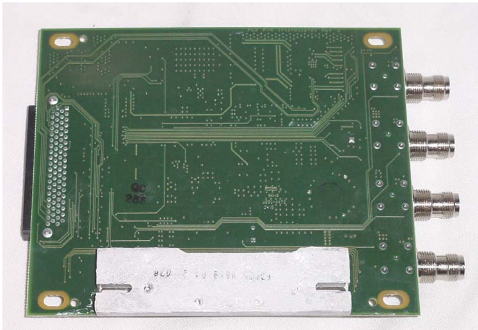
4 Port UHF Board Bottom View
