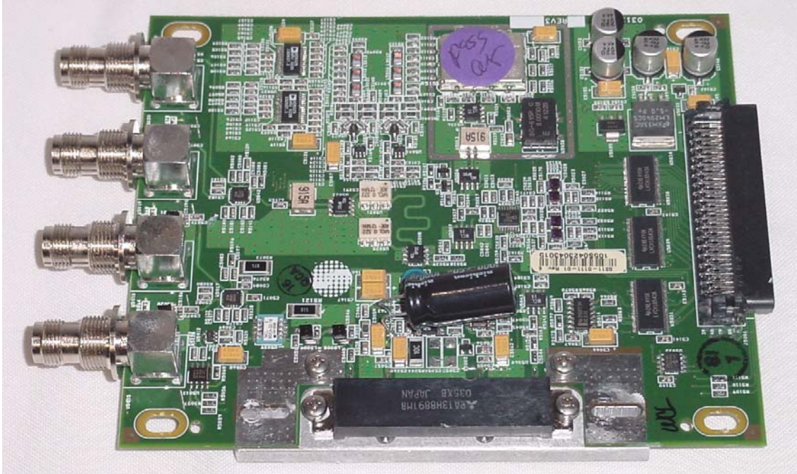
2 Port UHF Board Top View
