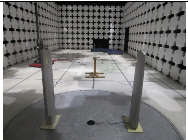
Radiated Emissions (<30MHz) – Rear View at 90 Degree
