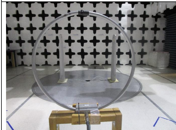
Radiated Emissions (<30MHz) – Front View at 0 Degree
