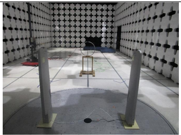
Radiated Emissions (<30MHz) – Rear View at 0 Degree
