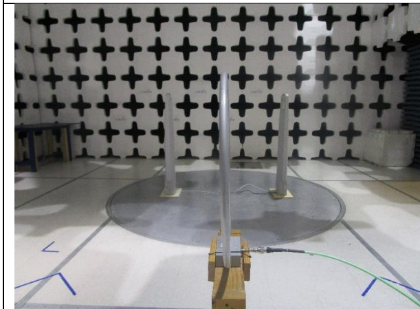
Radiated Emissions (<30MHz) – Front View at 90 Degree
