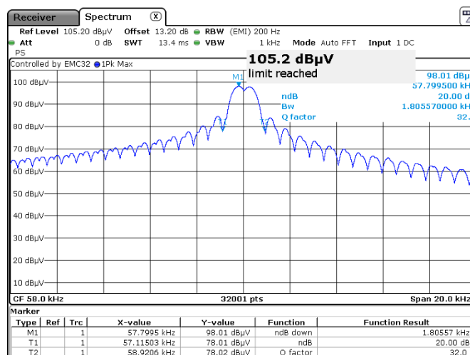
Figure 7.5-4: 20 dB bandwidth
