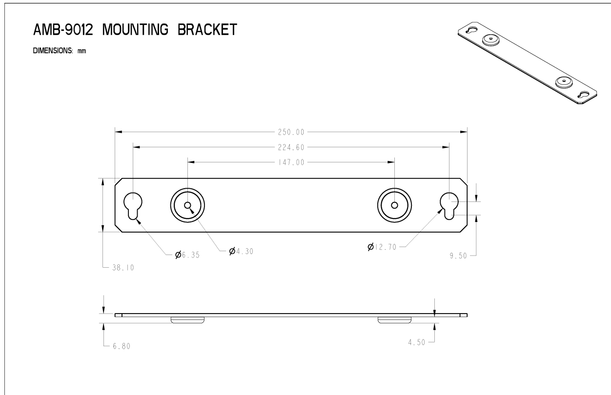
Figure 5: Mounting bracket
