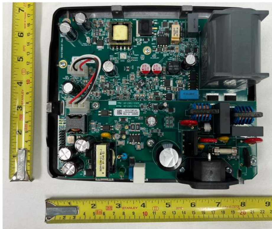
Cover Removed
