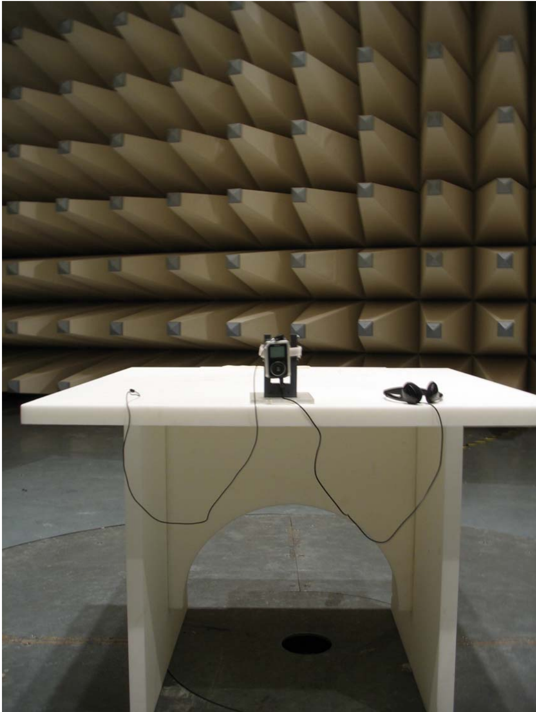
Photo 4: (Radiated Emission) Rx mode
