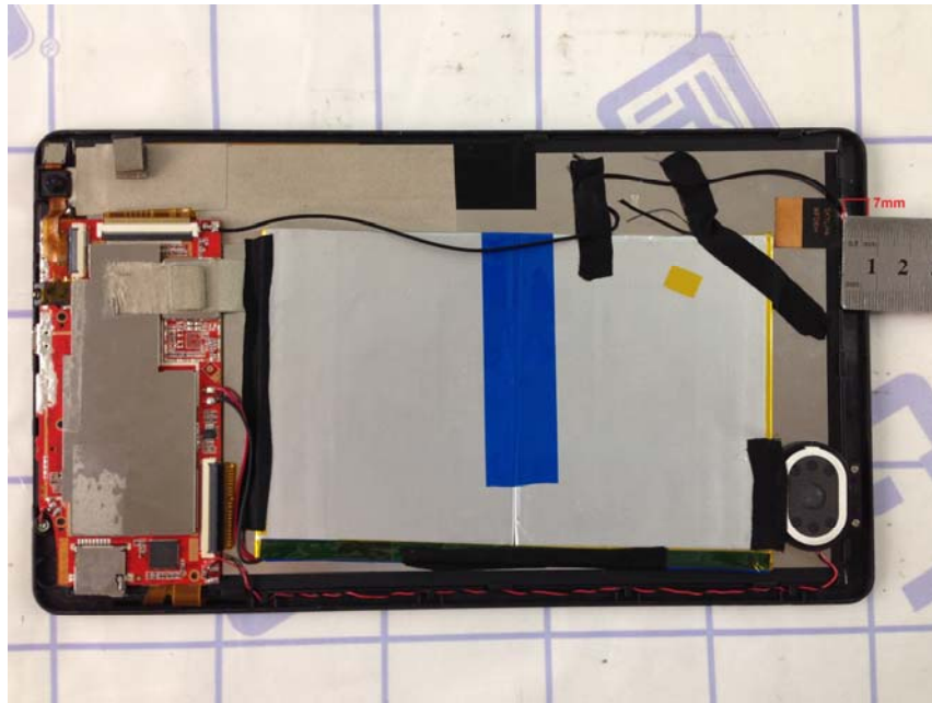
Antenna separation distance view-1
