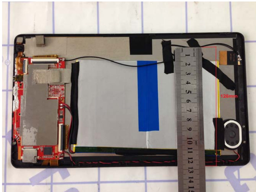
Antenna separation distance view-2
