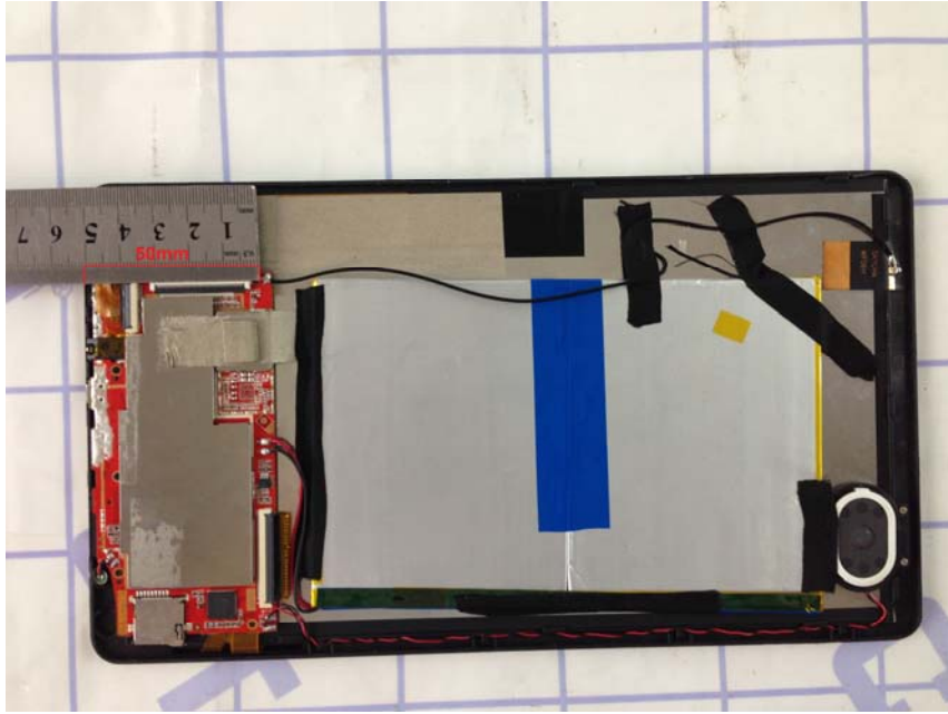
Antenna separation distance view-3
