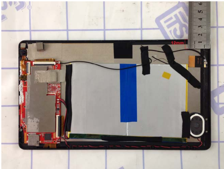
Antenna separation distance view-4
