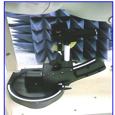
Figure 4. Device Holder
