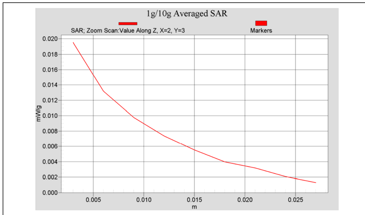
Body SAR Measurement _ Parent unit_close body _CH2
