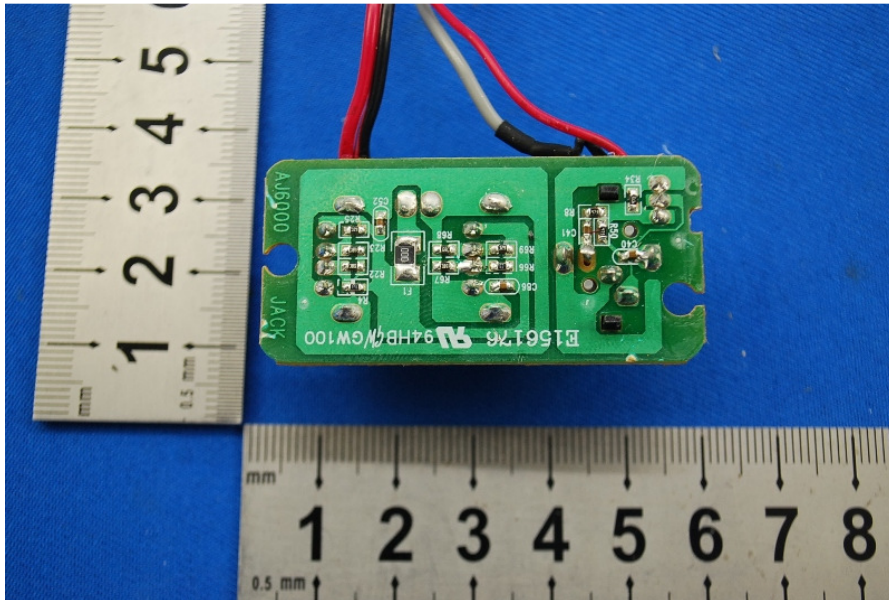
Adapter
