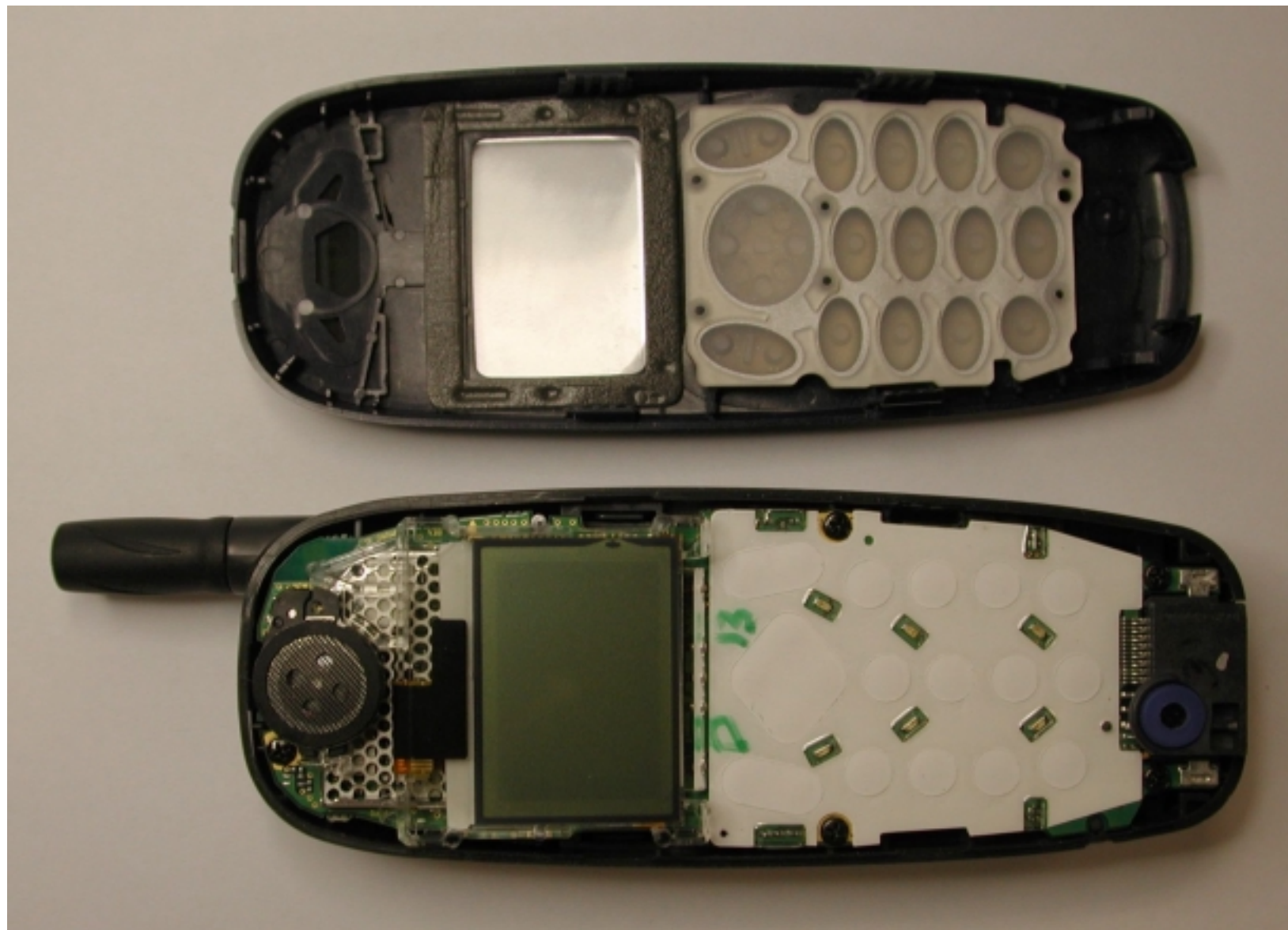
Photograph 2 -- MT289XG01A (Cover Off)
