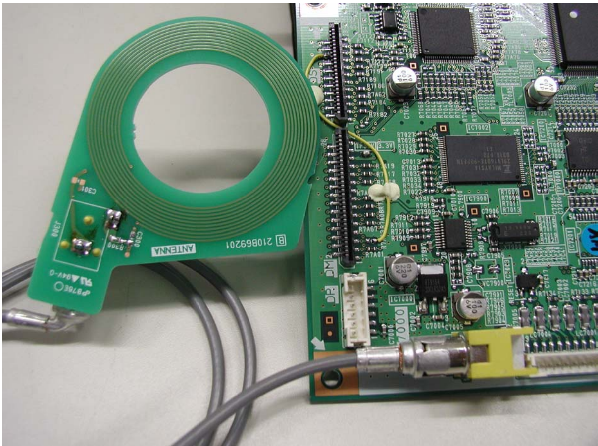
RFID part and Antenna (Side A)
