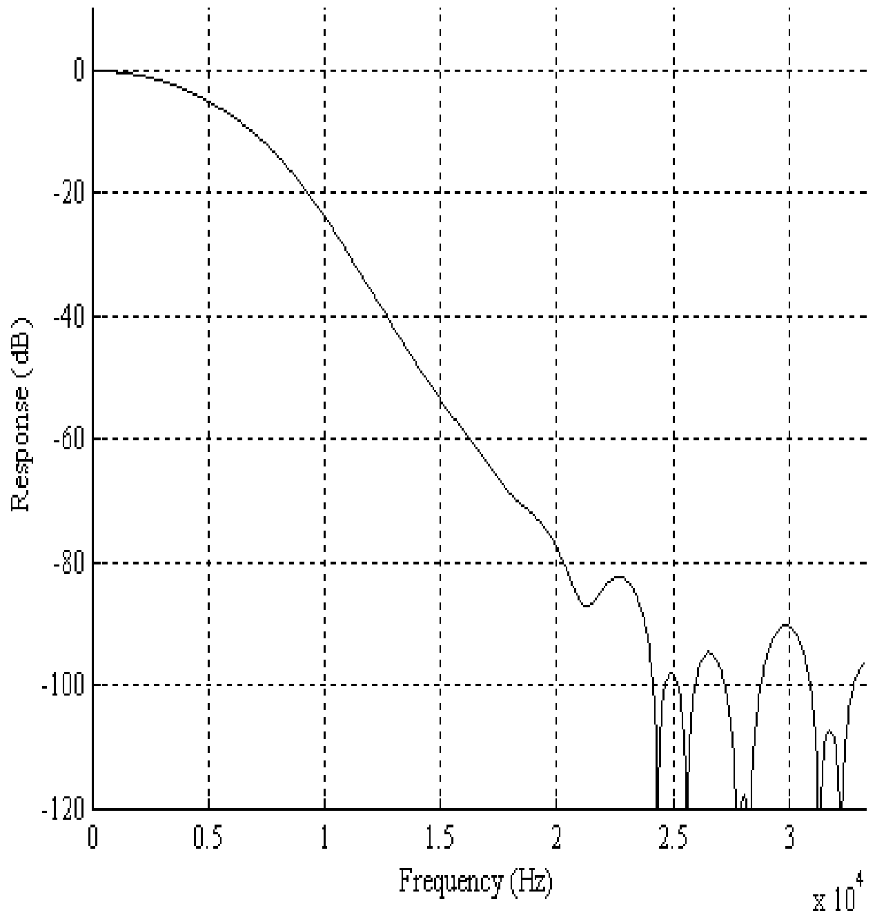
Frequency Response of Data Mode Premodulation Filter (88us)
