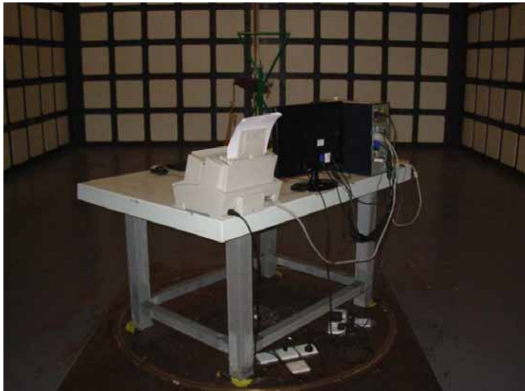
SETUP WITH MAXIMUM DETECTED EMISSION AT VERTICAL POLARIZATION (HDMI 1920*1080@60Hz)
