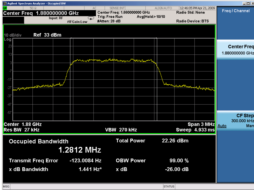
Plot 7-7. Occupied Bandwidth Plot (PCS CDMA Mode – Ch. 600)
