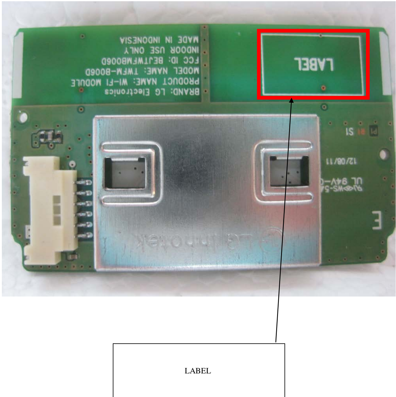
Figure 1.2 LABEL LOCATION
