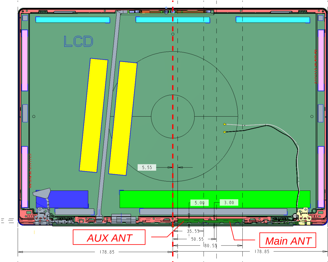
Figure 46 L1LRF015-CS-H, WLAN Combo Antenna Position
