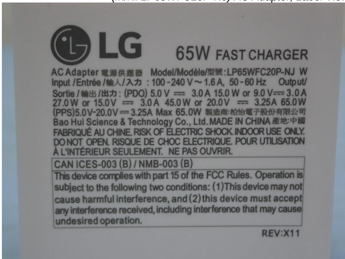
Figure 68 (M/N: LP65WFC20P-NJ) AC Adapter, Label View
