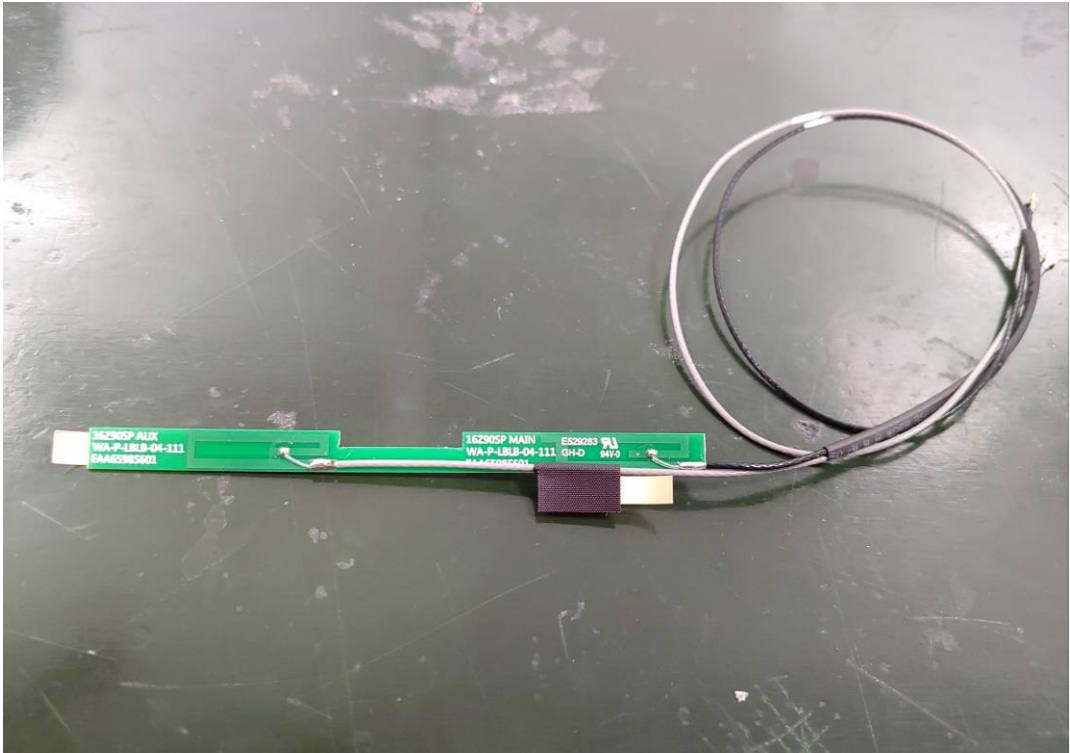
Figure 43 WA-P-LBLB-04-111, WLAN Combo Antenna
