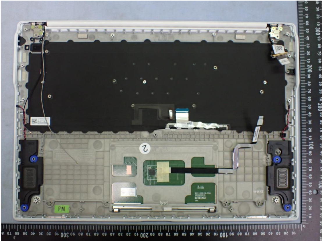
Figure 50 Internal View
