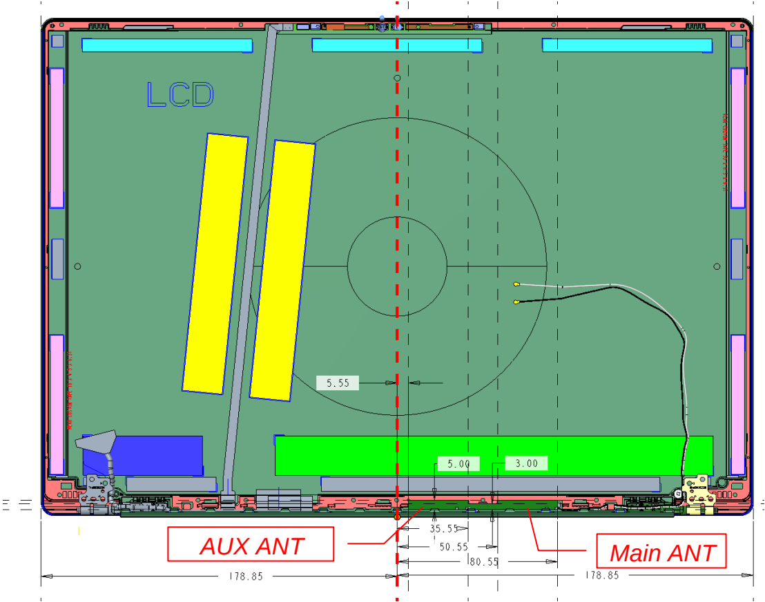
Figure 44 WA-P-LBLB-04-111, WLAN Combo Antenna Position
