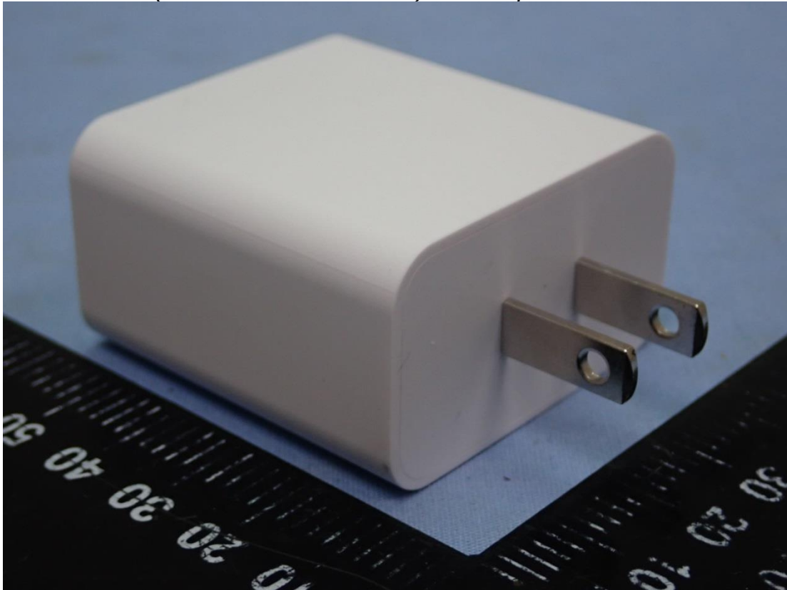
Figure 67 (M/N: LP65WFC20P-NJ) AC Adapter, Back and Side View
