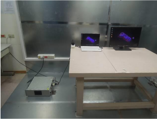
FCC_15_225_NFC_Conduction_Setup
