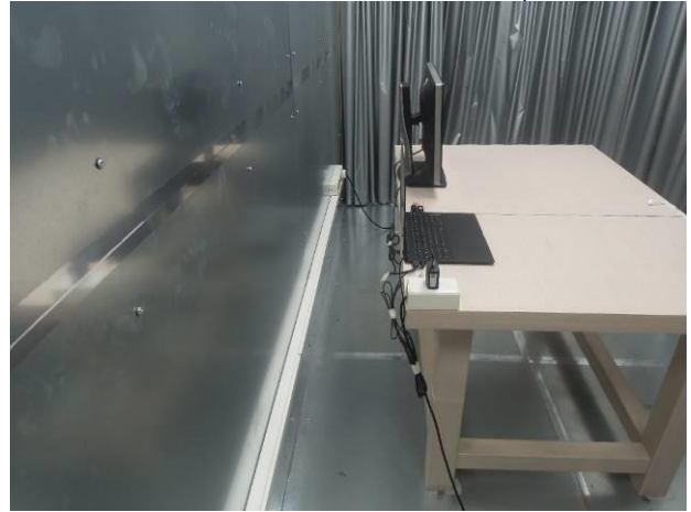
FCC_15_247_BT_Conduction_Setup
