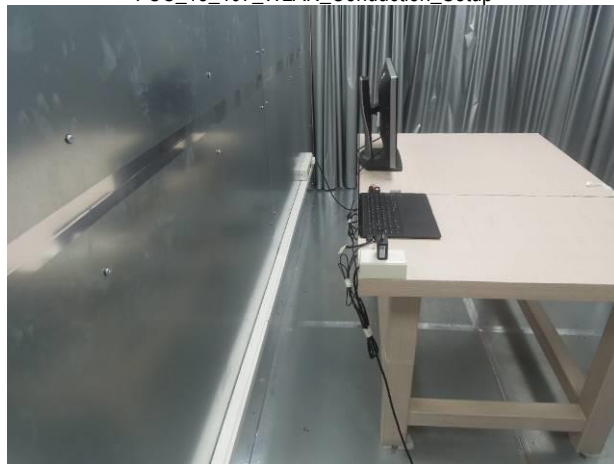
FCC_15_407_WLAN_6E_Conduction_Setup
