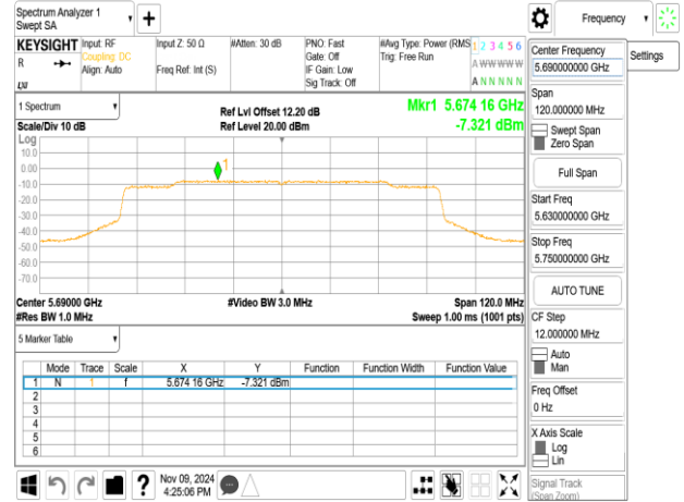
802.11ax_80MHz_ChainA_5690MHz_UNII 3
