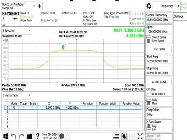
802.11ax_40MHz_ChainA_5310MHz_RU242_62
