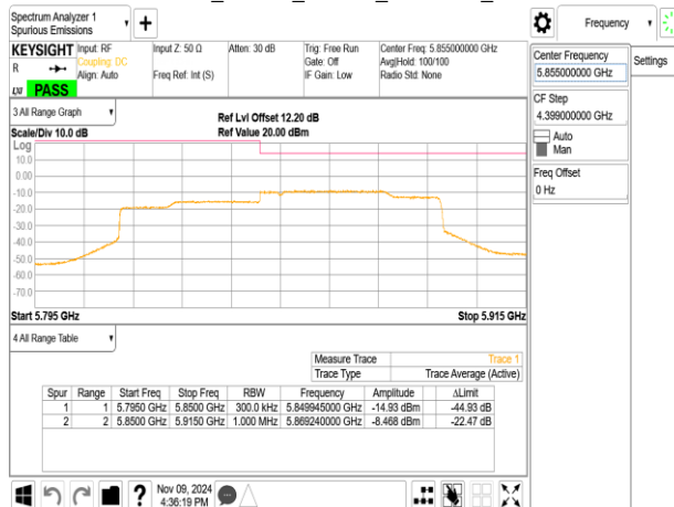
802.11ax_80MHz_ChainB_5855MHz_UNII 2C
