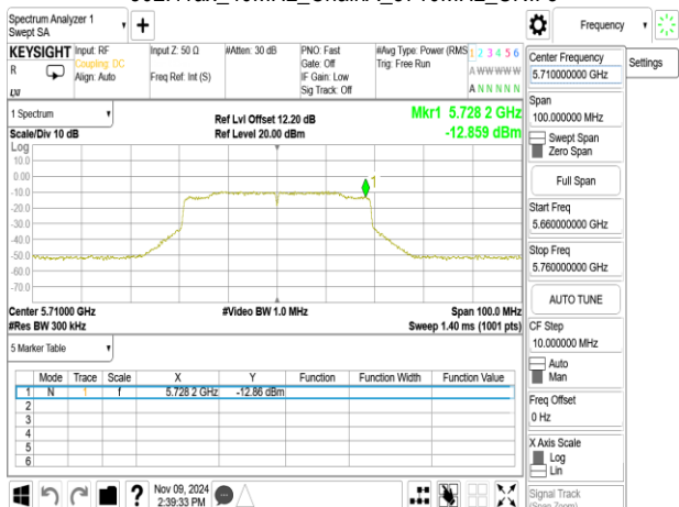
802.11ax_40MHz_ChainA_5710MHz_UNII 3
