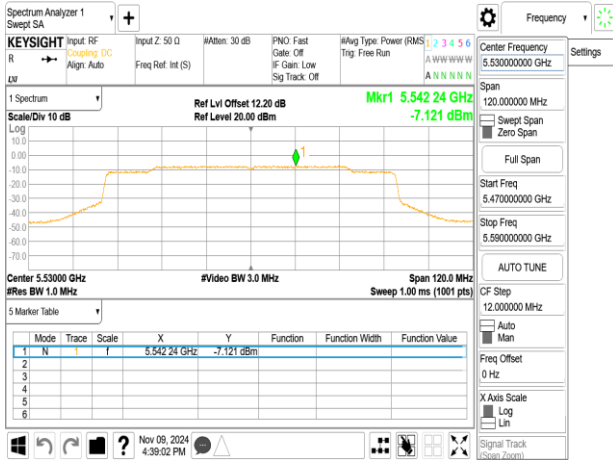
802.11ax_80MHz_ChainA_5530MHz_RU484_65
