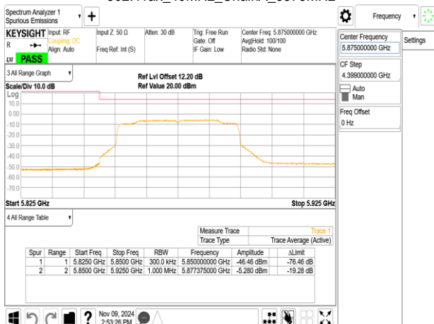
802.11ax_40MHz_ChainA_5875MHz
