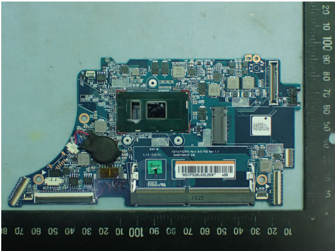
Figure 36 Internal View (LGIT, M/N 13/14/15Z970 Main Board, Back View)
