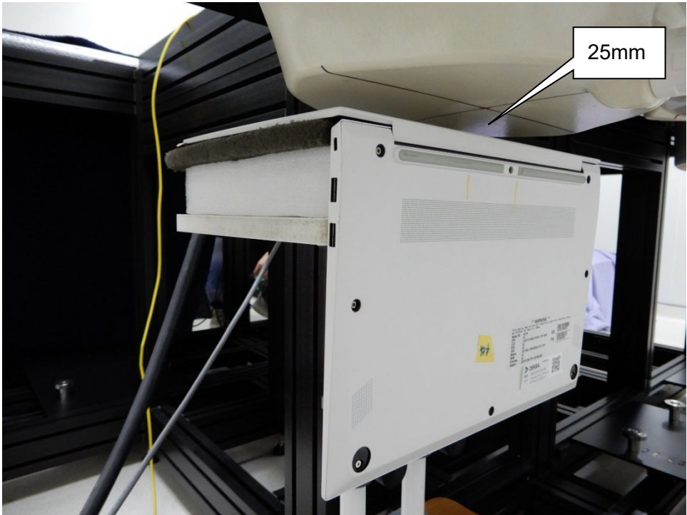
EUT Back_25mm
