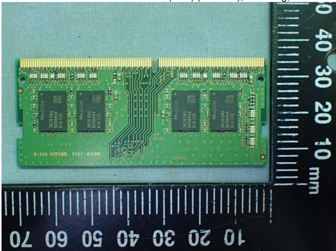
Figure 44 RAM (8GB) (On Card), Samsung, Back View
