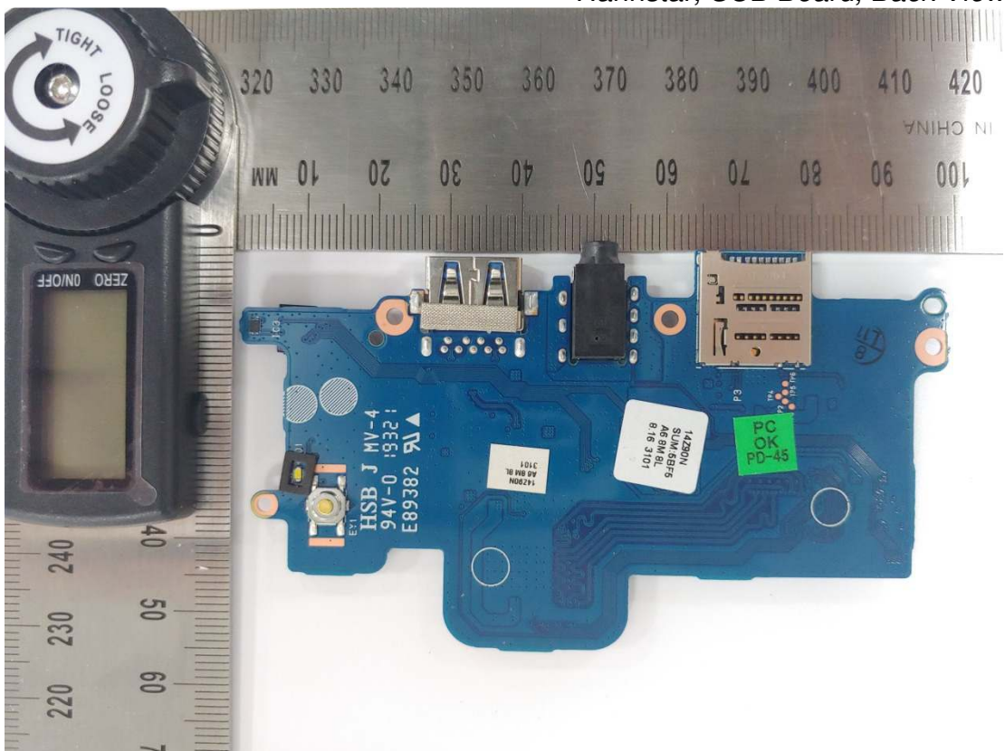
Figure 26 Hannstar, SUB Board, Back View
