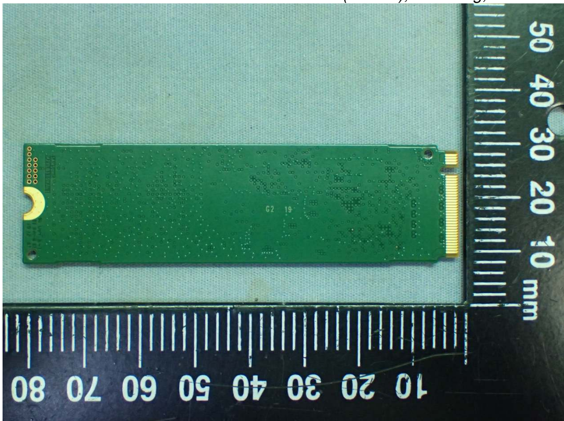
Figure 42 #2 SSD (256GB), Samsung, Back View
