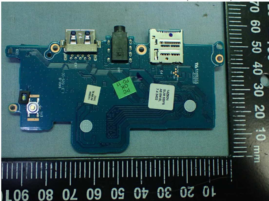
Figure 28 Elec & Eltek, SUB Board, Back View
