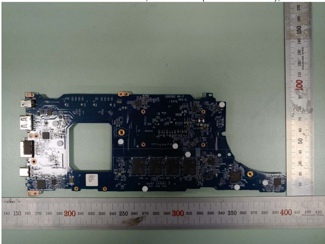
Figure 22 Hannstar, Main Board (with Thunderbolt), Back View
