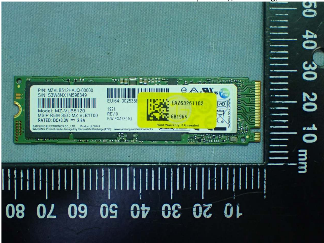
Figure 39 SSD (512GB), Samsung, Front View
