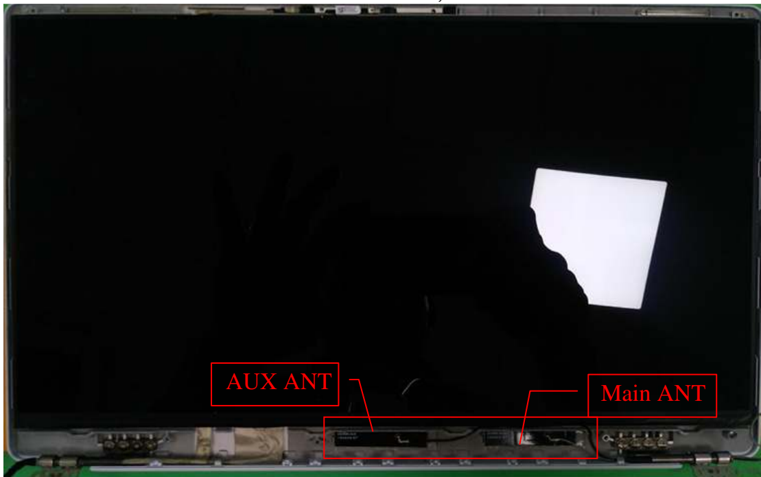
Figure 34 M/N L1LRF002-CS-H, WLAN Combo Antenna Position
