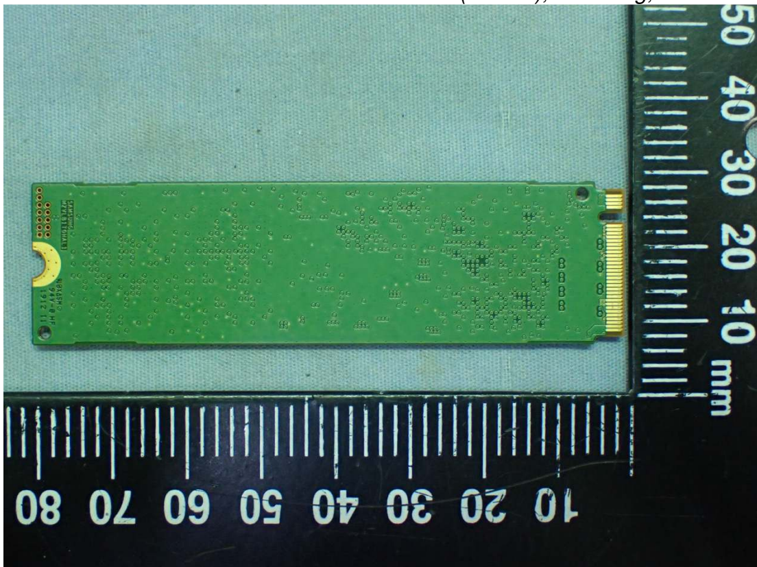
Figure 40 SSD (512GB), Samsung, Back View
