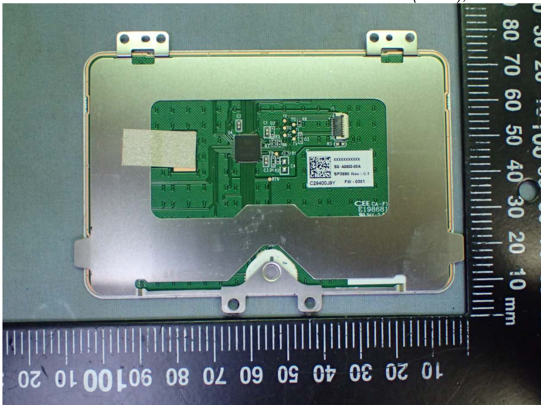
Figure 48 Touch Pad (White), Back View
