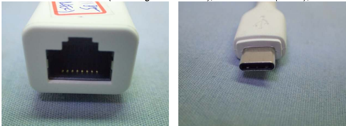
Figure 54 MEC (100 Megabit Ethernet), LAN Gender (White), IO View
