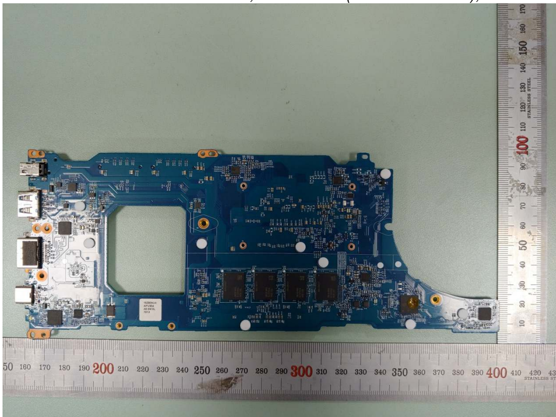
Figure 24 Elec & Eltek, Main Board (with Thunderbolt), Back View
