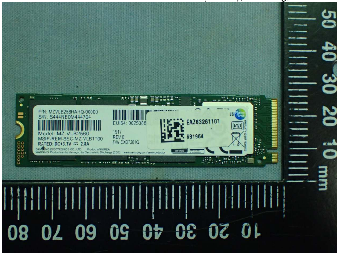
Figure 41 SSD (256GB), Samsung, Front View
