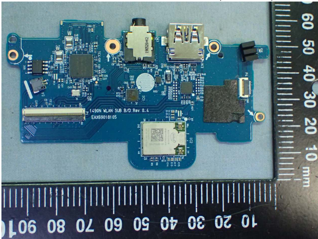
Figure 27 Elec & Eltek, SUB Board, Front View
