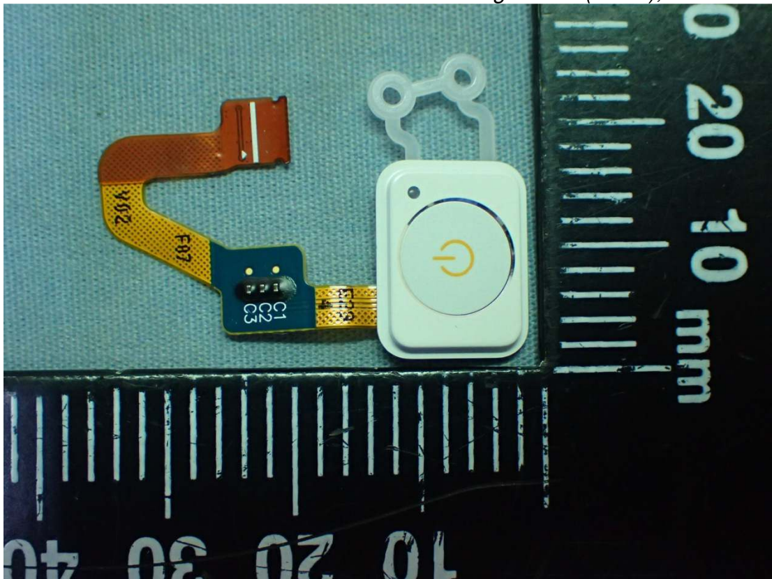
Figure 49 Finger Print (White), Front View
