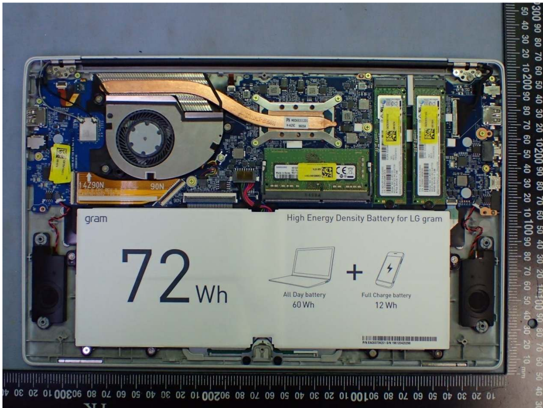
Figure 17 Internal View
