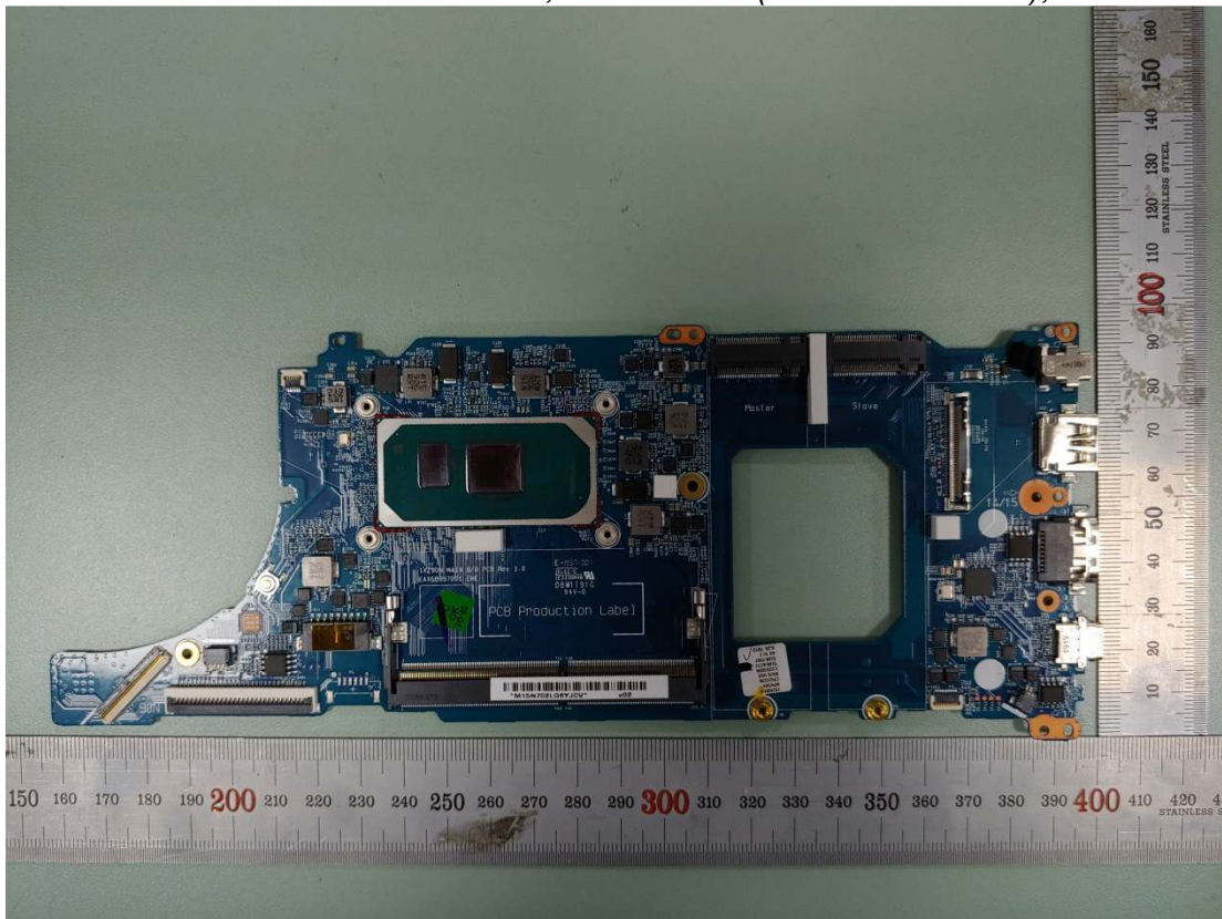
Figure 23 Elec & Eltek, Main Board (with Thunderbolt), Front View
