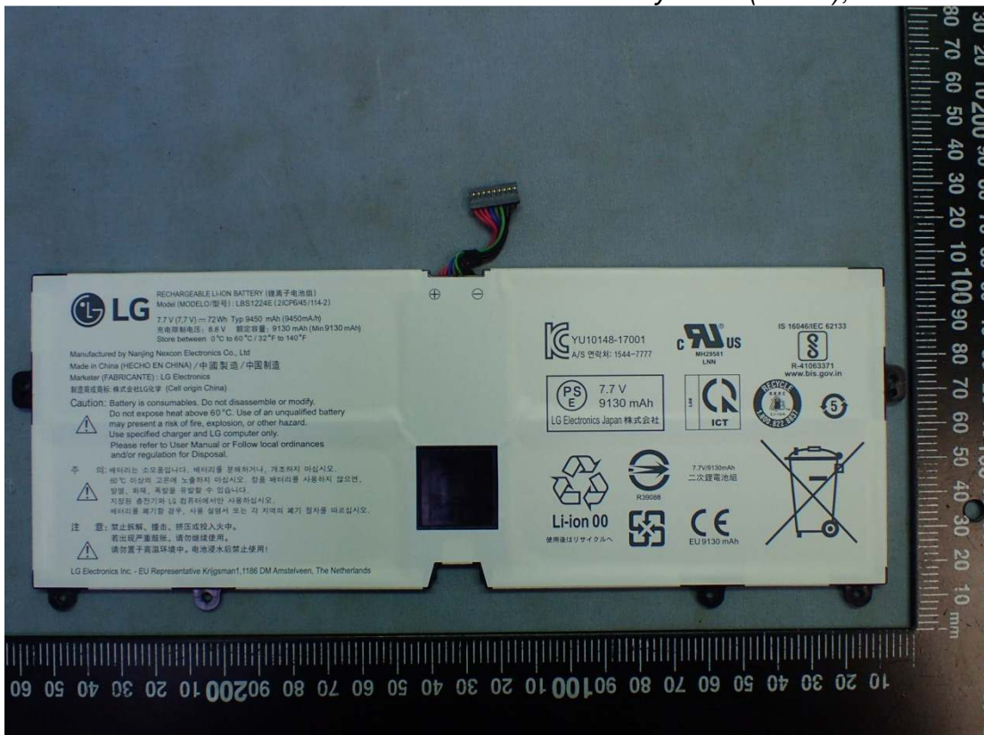
Figure 38 Battery Pack (72Wh), Back View
