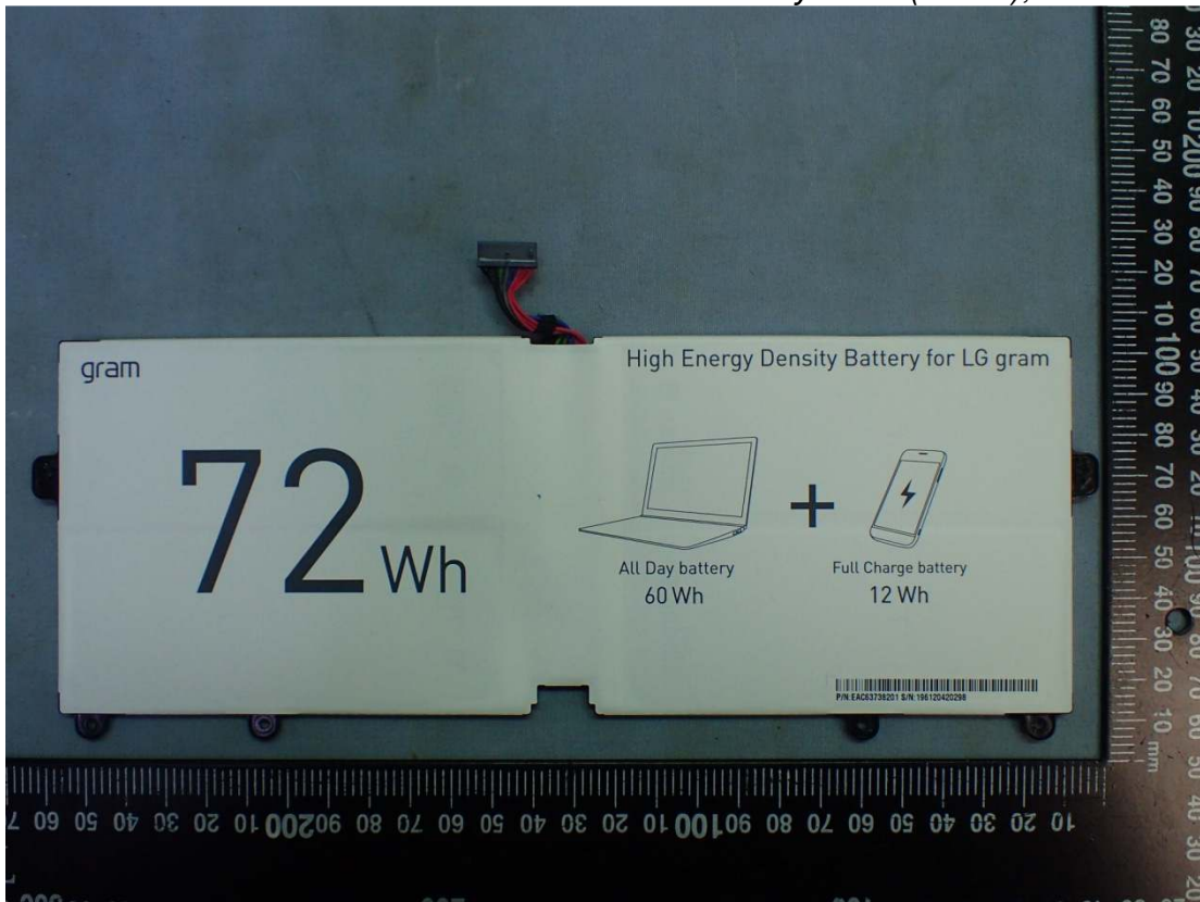
Figure 37 Battery Pack (72Wh), Front View
