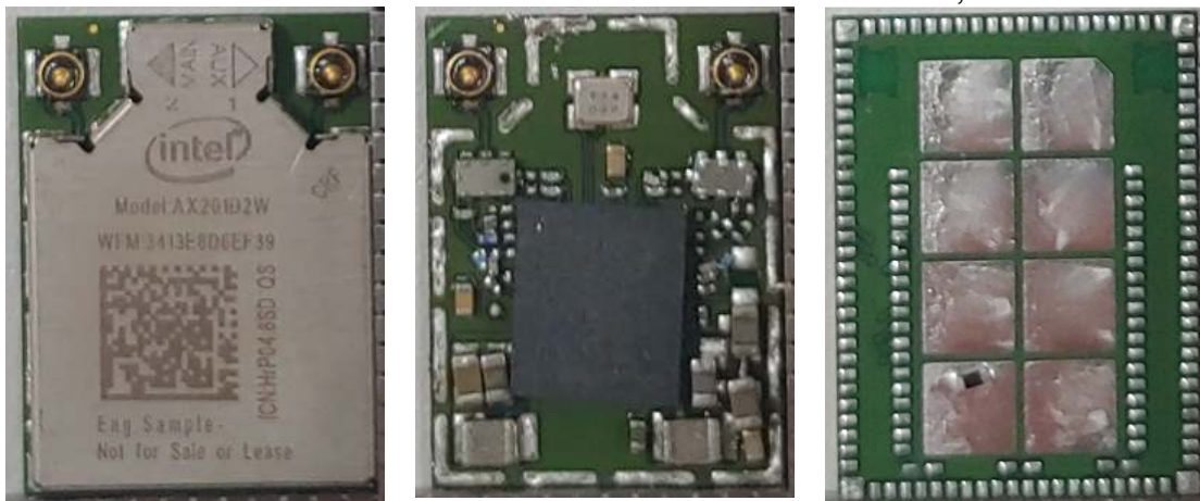
Figure 30 WLAN Combo Card, Remove Cover
